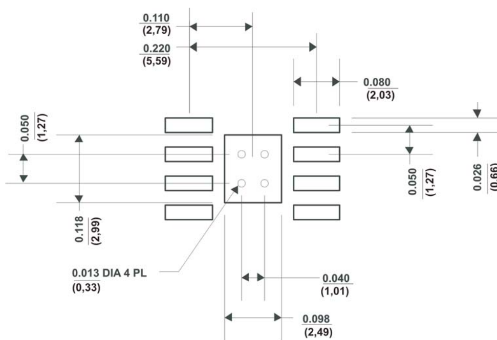
Figure 9. Design Layout
