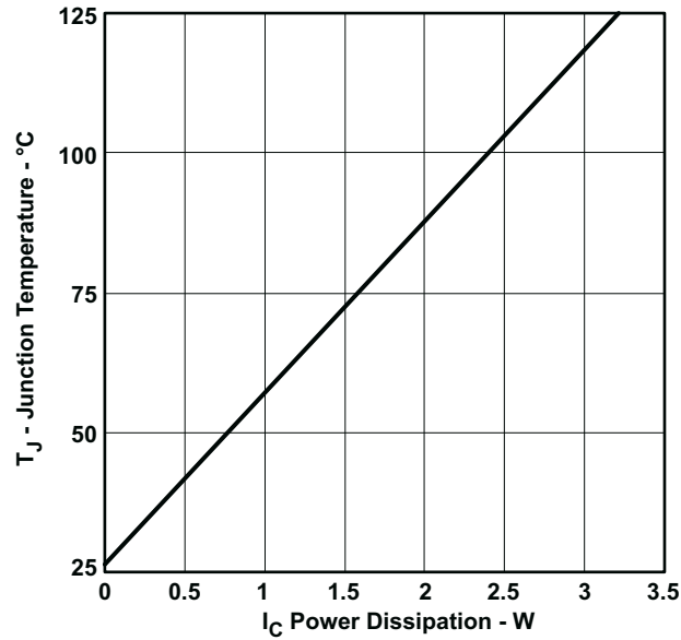
Figure 18. TPS5450 Power Dissipation vs Junction Temperature.
