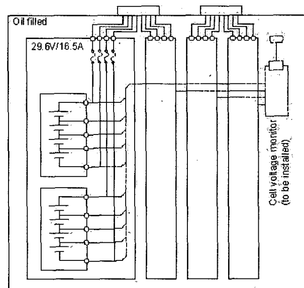
Fig. 2: a Li-ion battery pack
