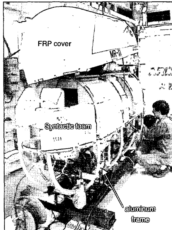
Fig. 1: An overview of MR-X1.
