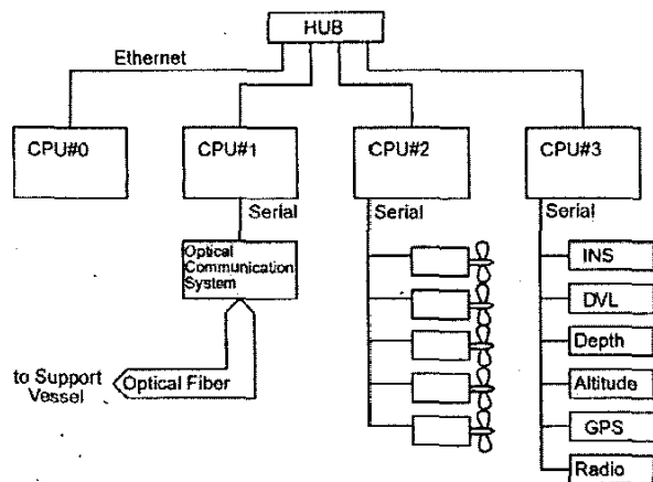
Fig. 3: A block diagram of early prototype MR-X1
