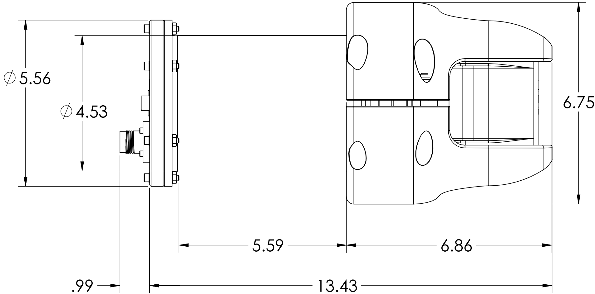
IMPULSE CONNECTOR MSSJ-7-FCR
