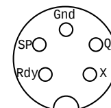
Strobe Connector Female Face View
