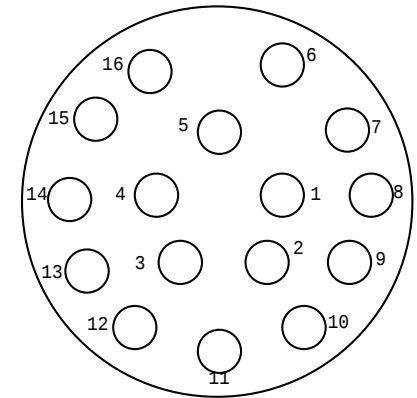
Subconn DCM16M Male Face View
