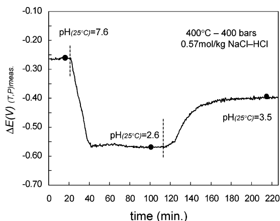
Figure 3. YSZ cell potential \Delta E(V)_{(T,P)\text{meas}} vs recording time during a typical flow-through experiment with 0.57 mol/kg NaCl–HCl solution at 400 °C and 400 bar (modified after ref 32). Dash lines indicate changes in the \text{pH}_{(25^\circ\text{C})} (7.6 to 2.6 and 2.6 to 3.5) of source fluid. Solid symbols represent real time measurements of \text{pH}_{(25^\circ\text{C})} of fluid leaving the reactor. Taking account of reactor volume (50 mL), and flow rate (2 mL/min), which promotes continuous fluid mixing, data indicate that cell potential responds rapidly to changes in acidity of the source fluid.
