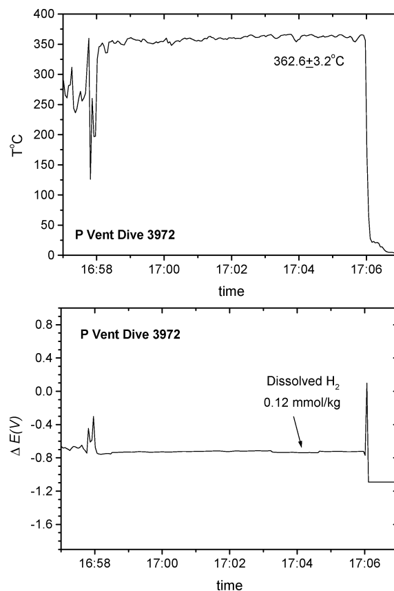
Figure 29. In situ chemical sensor measurement of dissolved \text{H}_2 along with fluid temperature at P vent in 2004 (EPR 9°50'N). This particular deployment was conducted in real time mode, independently from the time series monitoring effort depicted in Figure 28. In situ dissolved \text{H}_2 concentration determined from the real-time deployment is consistent with data obtained separately from a gastight sample (0.18 mmol/kg, shown in Figure 24), and is also consistent with the value acquired through time series monitoring study (see text and Figure 28). The time axis is in the GMT time with a format of hour/minute.
