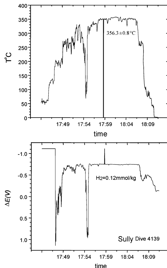
Figure 22. Chemical and temperature data from real-time deployment of the sensor system at Sully vent site (MEF) (modified after ref 79). Measured dissolved H 2 sensor potentials ( \Delta E(V) ) of hydrothermal fluids demonstrate rapid response rate. The time scale is in the format of hour/minute. Changes in temperature indicate seawater-mixing effects. In spite of the dynamic nature of hydrothermal vents, the sensor response is sufficiently rapid to delineate primary (endmember hydrothermal fluids) and secondary (seawater) sources.
