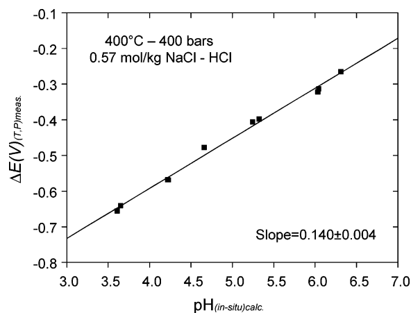
Figure 6. Measured potential \Delta E(V)_{(T,P)} for YSZ–pH sensor at 400 °C and 400 bar plotted against theoretically calculated \text{pH}_{(\text{in-situ})\text{calc}} to constrain the thermodynamic viability of the sensor (modified after ref 32). The slope of the linear correlation is very close to that predicted for standard Nernstian response (0.134) at the conditions tested, which suggests that the YSZ–pH sensor is thermodynamically sound and responds specifically to \text{pH}_{(\text{in-situ})} .
