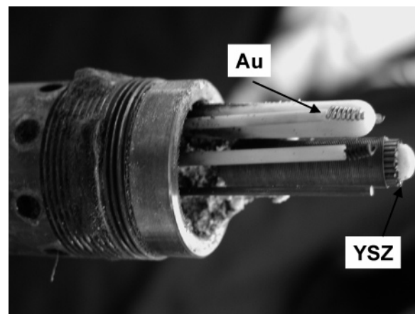
Figure 30. Close-up examination of the electrochemical and thermocouple array following deployment in vent fluid issuing from P-vent at temperatures in excess of 360 °C (EPR 9°50'N). In situ sensors used for dissolved \text{H}_2 (Au electrode) and pH (YSZ pH) are appropriately indicated.
