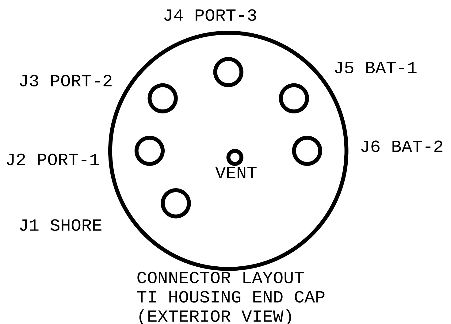
SYSTEM CONTROLLER HOUSING
