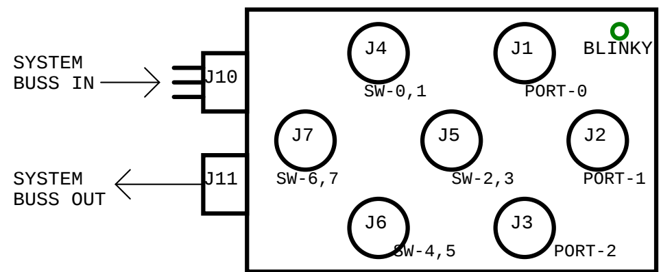
CONNECTOR LAYOUT TOP VIEW
