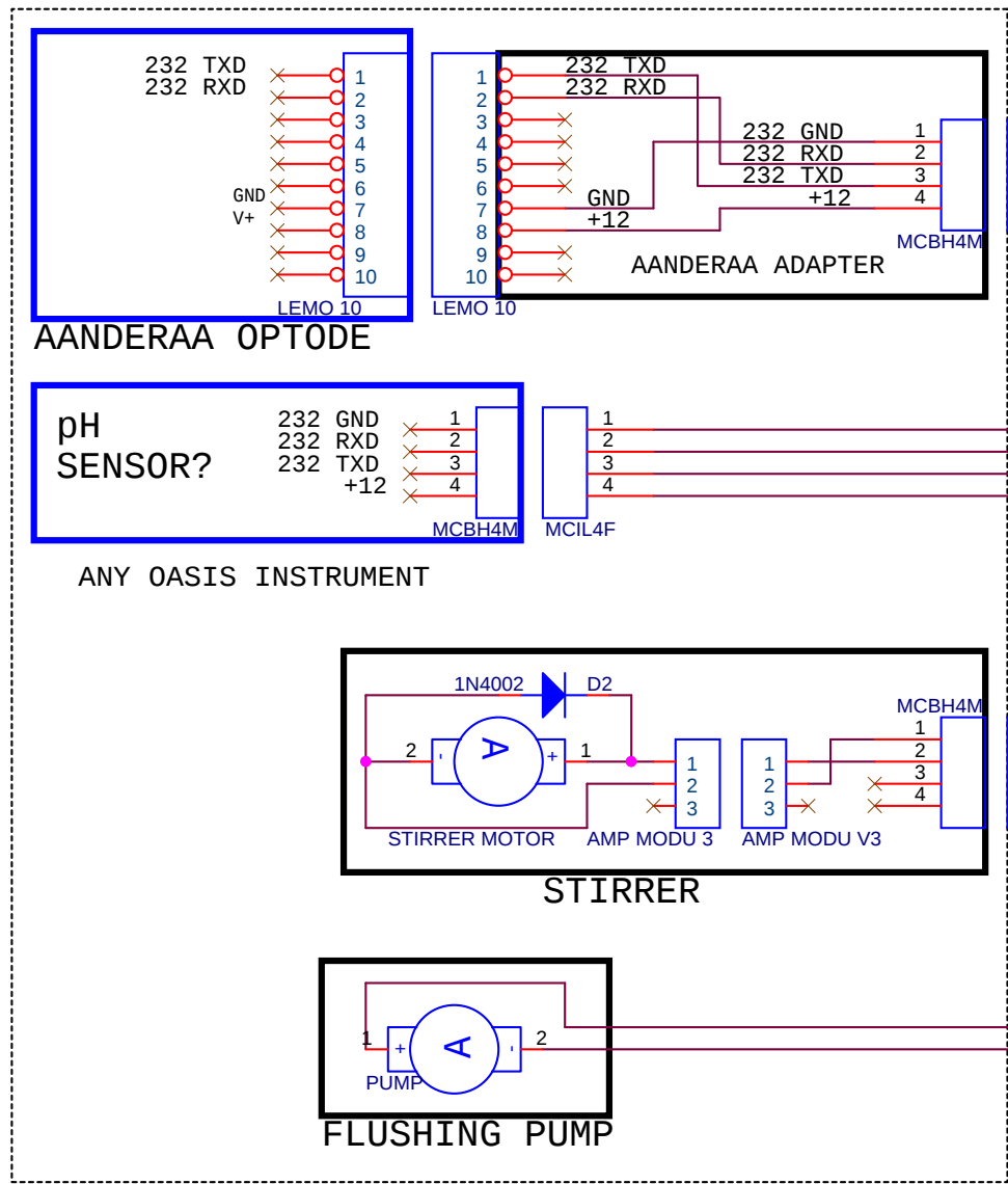
RESPIRATION CHAMBER OR D-SAMPLER
