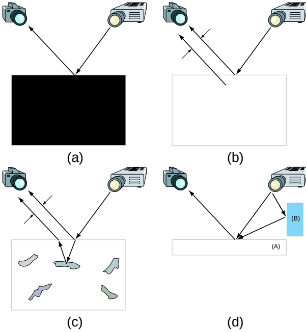
Figure 2. Raytracing in 3D scanning. (a) 3D geometry can be estimated reliably only from the direct reflection off the surface. (b) The subsurface scattering in translucent objects shifts the observed intensity peak away from the point of incidence. (c) Opaque structures beneath the surface pollute the range estimate. (d) The signals of different projector rays are overlaid due to interreflection from another surface.
