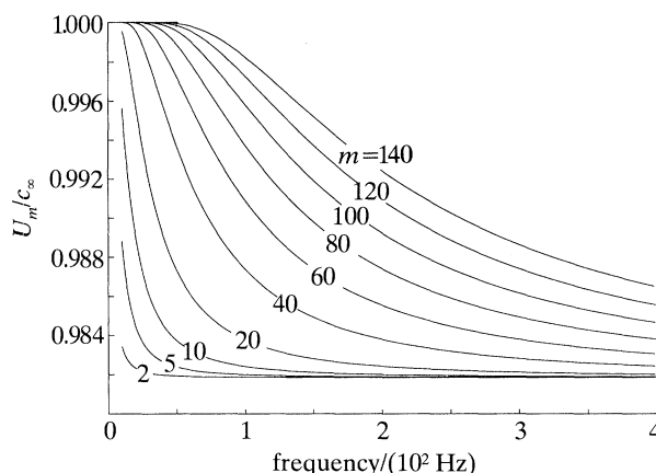
Figure 13. Group velocities of modes in the Arctic profile of figure 5.
