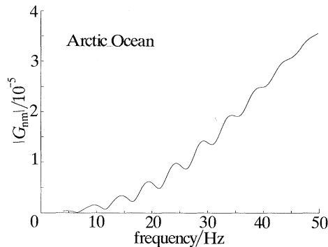
Figure 10. |G_{nm}| (Arctic Ocean) as a function of frequency from (47) ( Q = 1 ), with the source and receiver at the same depth (below the surface) of 50 m and separated in range by 10 km.
