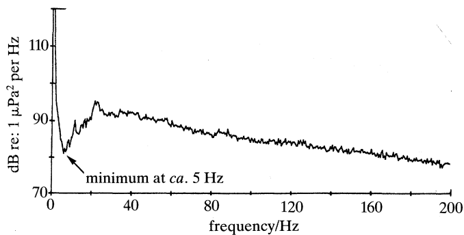
Figure 12. VLF ambient noise spectrum from the MIZ east of Greenland. ( 76^{\circ} 37.6' \text{ N} , 07^{\circ} 32.2' \text{ W} ; hydrophone depth \approx 160 \text{ m} ; 60% ice cover; light wind, speed \approx 3.5 \text{ m s}^{-1} ; sea state, 1–2; swell, nil; visibility greater than 10 km; 4 September 1988.)
