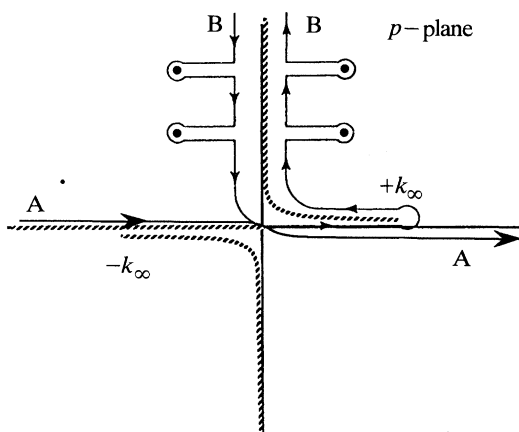
Figure 22. Branch cuts (hatched lines) for S_\mu(\eta) , beginning at \pm k_\infty (which is assumed to have a infinitesimal imaginary component); and for the Hankel functions, along the negative real axis. Contour (A-A) of integration for the integral I is deformed (B-B) to follow the upper branch cut enclosing the poles of S_\mu(\eta) .
