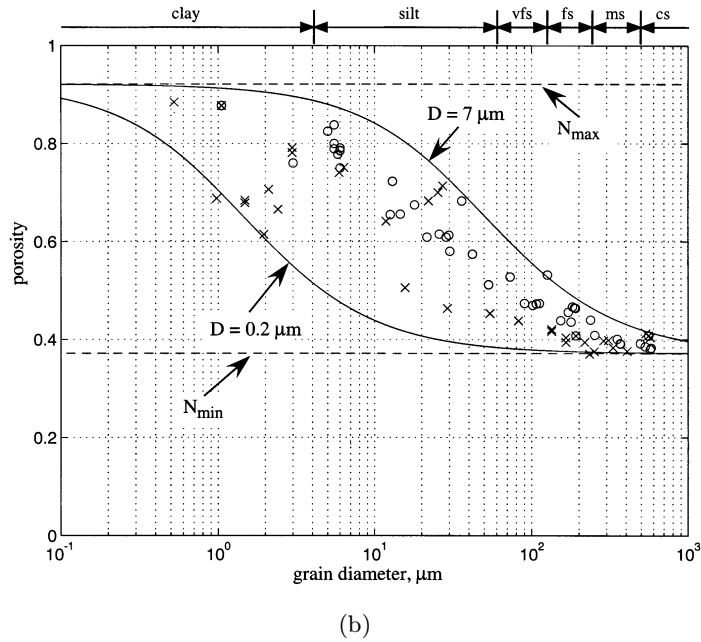
Fig. 1. Porosity versus grain size for unconsolidated marine sediments. The symbols represent data from Hamilton 10,20 (circles), Richardson and Briggs 21 (crossed circles), and Richardson and Briggs 22 (crosses). The limiting values of porosity, N_{\max} and N_{\min} , are discussed in the text. The theoretical curves labeled (a) D = 3 \mu\text{m} and (b) D = 7 \mu\text{m} and D = 0.2 \mu\text{m} represent Eq. (2.3), as evaluated using the cited values of the r.m.s. grain roughness. The key to the grain-size categories is: cs = coarse sand, ms = medium sand, fs = fine sand, and vfs = very fine sand.
