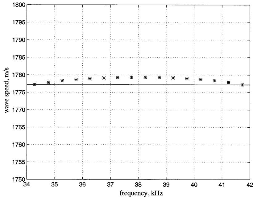
Fig. 13. Wave speed at 30-cm depth in the sediment as a function of frequency, as estimated from the pulses in Fig. 8. The asterisks (*) were computed from (28) and the solid line is the wave speed estimated from the inter-receiver correlation delay between the pulse arrivals.
