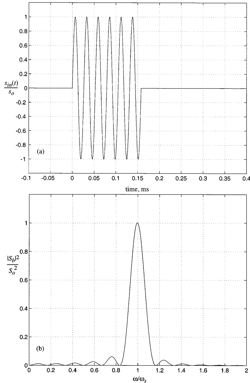
Fig. 2. (a) Sinusoidal input pulse from (5). (b) Its power spectrum from (7) ( m = 6 and \omega_s/2\pi = 38 kHz).
