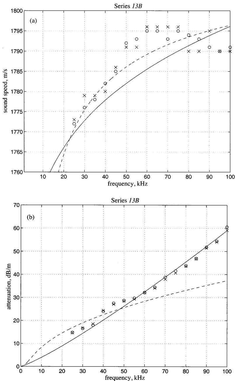
Fig. 21. (a) Wave speed; (b) attenuation as a function of frequency. The data (circles, o, and crosses, x) are the same Series 13B data points as in the top-right and bottom-right panels of Fig. 19. The solid lines are from the grain shearing theory, (37) and (38), with c_o = 1687 m/s, n = 0.205 and \eta = 0.009 ; and the broken lines are from the Biot theory, (43) and (44), with c_o = 1687 m/s, c_\infty = 1820 m/s and \gamma = 0.03 ms.
