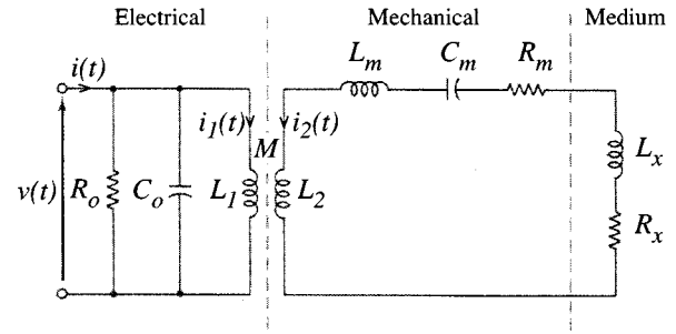
Fig. 1. Equivalent electrical circuit of the piezoelectric source transducer.
