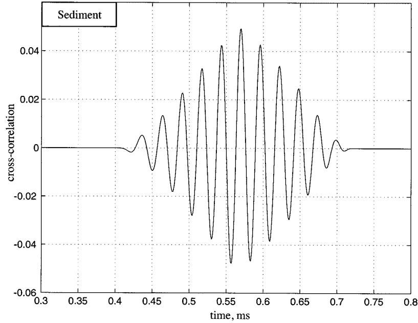
Fig. 9. Correlation function between the two sediment arrivals in Fig. 8. Zero-padding was used to suppress noise before and after the pulse arrivals. The distance between the two receivers, as calibrated acoustically from the correlation delay in the water column, was d_w = 1.013 m.
