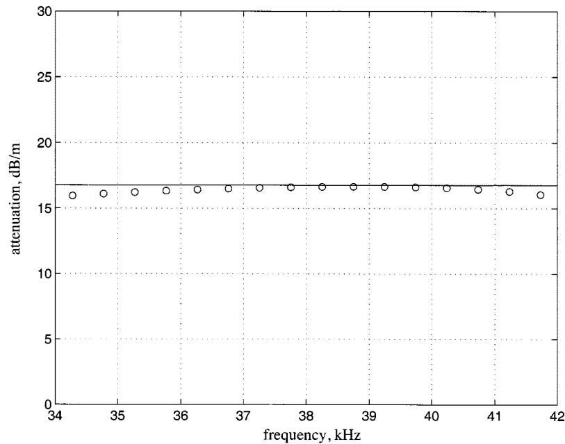
Fig. 14. Attenuation as a function of frequency at a depth of 30 cm in the sediment, estimated from the pressure-pulse arrivals in Fig. 8. The open circles were computed from the power spectra of the pulses using (32), and the solid line is the attenuation estimated from the mean-square values of the two pulses, (35).
