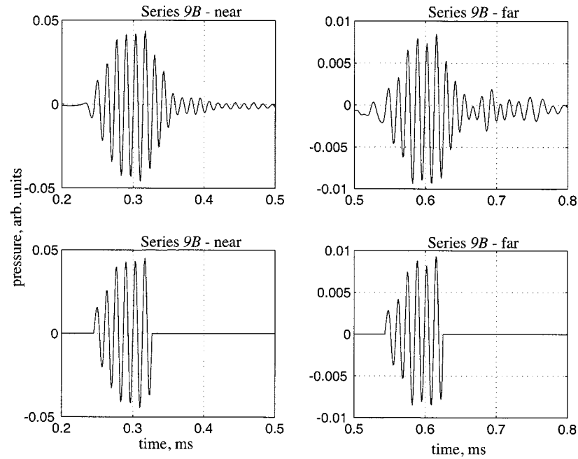
Fig. 18. Series 9B, 75 kHz arrivals in sediment, raw data (a) near-phone and (b) far-phone. The same signals are shown in (c) and (d), respectively, after subtracting the mean level, windowing six cycles, and Butterworth filtering.
