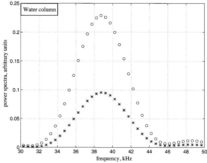
Fig. 10. Power spectra of the water-column pressure-pulse arrivals in Fig. 4. The open circles (o) represent the near receiver (nominal range 0.298 m) and the asterisks (*) the far receiver (nominal range 1.3 m). For clarity of presentation, the latter levels have been scaled up by a factor of 10.
