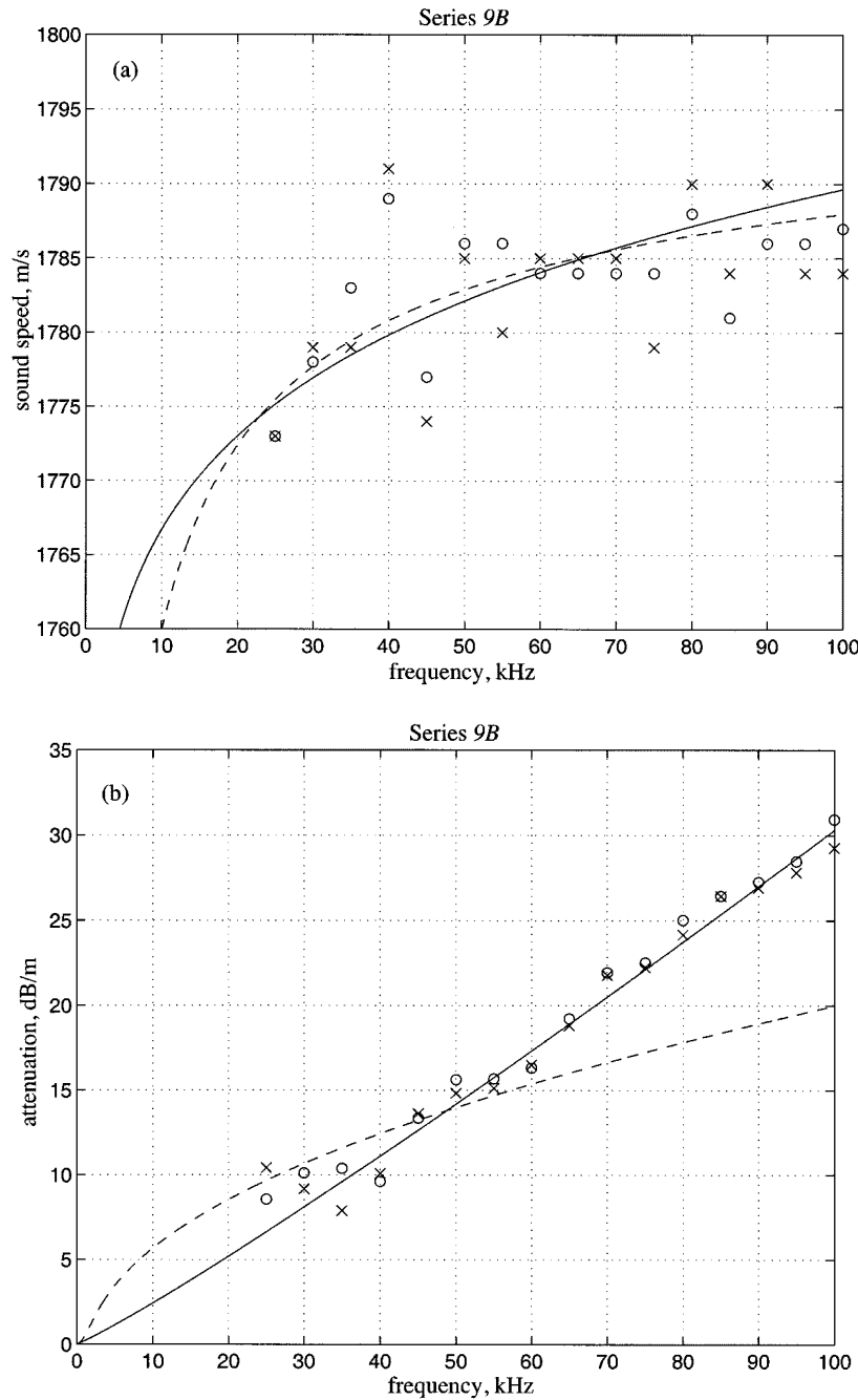
Fig. 20. (a) Wave speed; (b) attenuation as a function of frequency. The data (circles, o, and crosses, x) are the same Series 9B data points as in the top-left and bottom-left panels of Fig. 19. The solid lines are from the grain shearing theory, (37) and (38), with c_o = 1687 m/s, n = 0.113 and \eta = 0.028 ; and the broken lines are from the Biot theory, (43) and (44), with c_o = 1687 m/s, c_\infty = 1800 m/s and \gamma = 0.08 ms.
