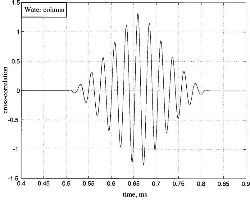
Fig. 5. Correlation function (unnormalized) between the water-column arrivals in Fig. 4. Zero padding was used to eliminate noise before and after the pulse arrivals.
