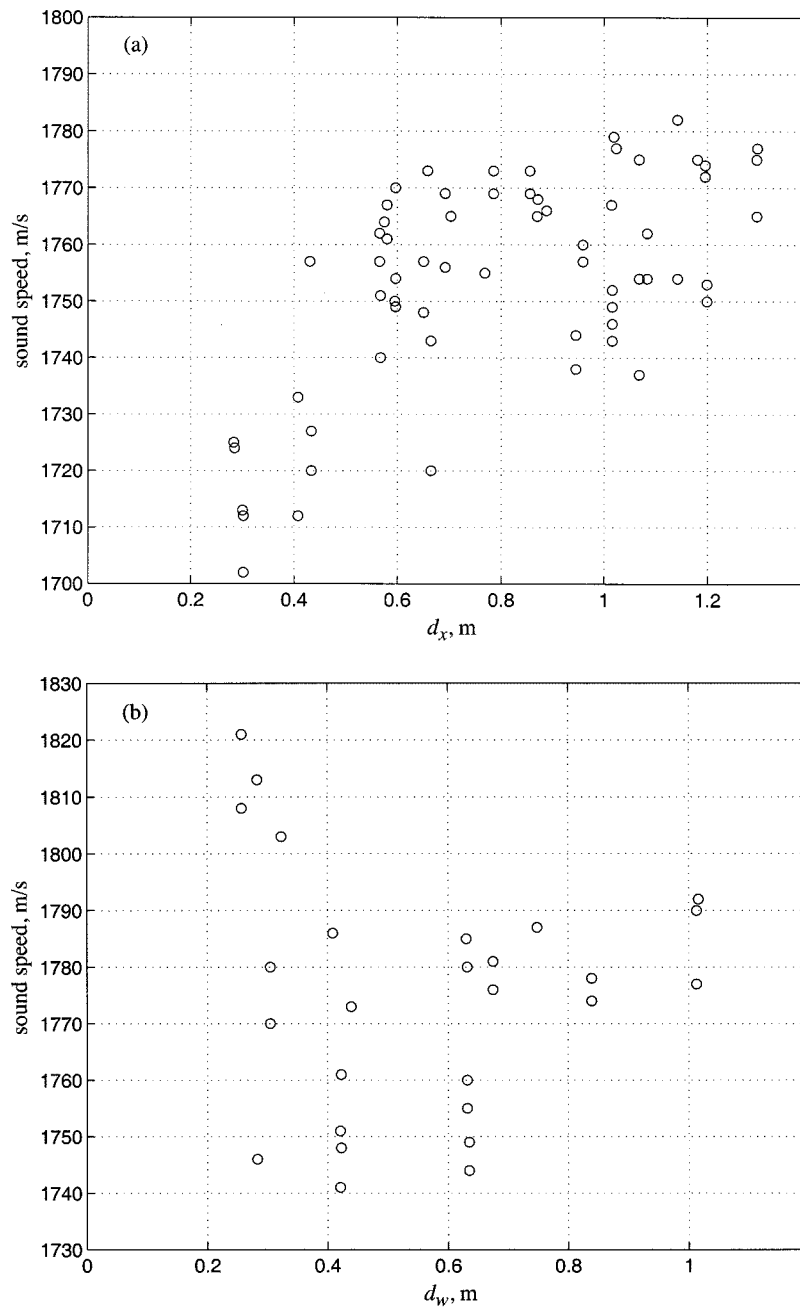
Fig. 15. Measured sound speed at stations 15 and 23 with probes 30-cm deep in the sediment, as a function of transducer separation. (a) Source-to-receiver path lengths, d_x , cross-correlation timing, and (29). Note the trend toward higher sound speeds at greater distances. (b) Receiver-to-receiver path lengths, d_w , and inter-receiver correlation timing.
