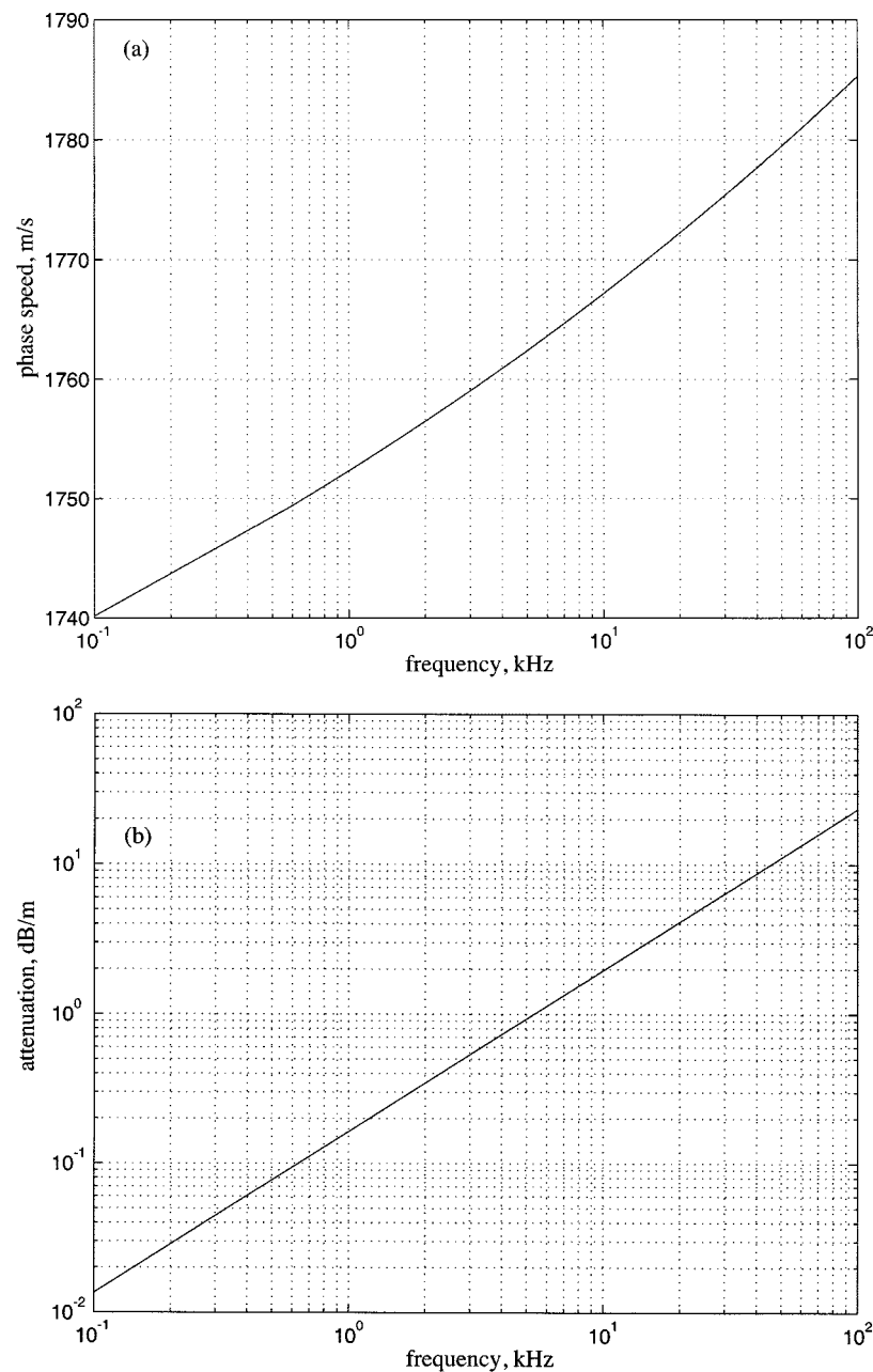
Fig. 7. Theoretical (a) dispersion; (b) attenuation in the sediment, from (26).
