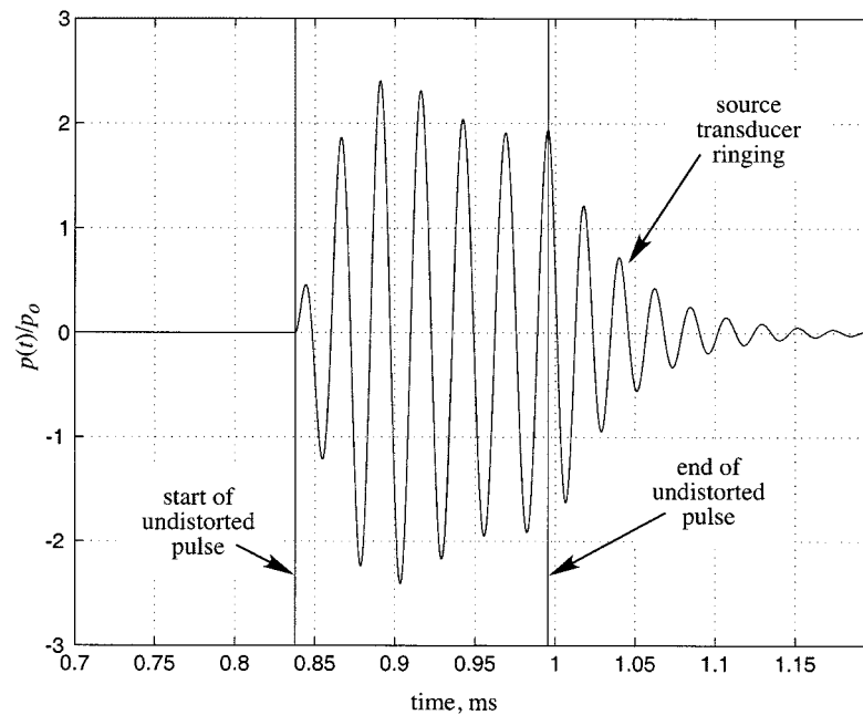
Fig. 3. Theoretical pressure-pulse shape in the water column, range 1.3 m, evaluated from (14) for operating conditions on Julian day 291, SAX99 (see text). The vertical lines indicate where the beginning and end of the pressure pulse would have fallen had there been no distortion from the source transducer.
