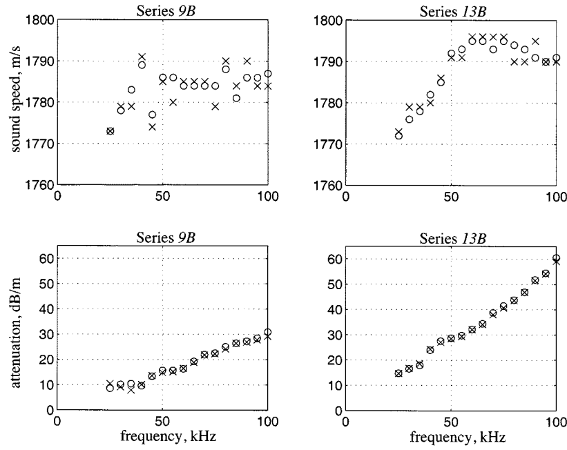
Fig. 19. Group speed from cross-correlation (crosses, \times ) and phase speed from phase delay (circles, \circ ) as a function of frequency. Also shown are the broadband attenuations from mean-square levels (crosses, \times ) and spectral amplitudes (circles, \circ ).
