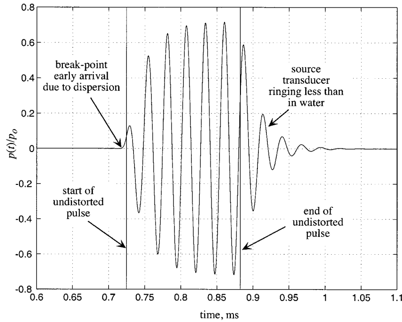
Fig. 6. Theoretical pressure-pulse shape in sediment, at range 1.3 m, evaluated from (10). The vertical lines indicate where the beginning and end of the pulse would have fallen had there been no dispersion or attenuation in the medium, and no distortion from the source transducer.
