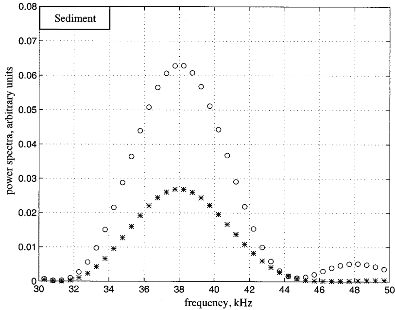
Fig. 11. Power spectra of the sediment pressure-pulse arrivals in Fig. 8. The open circles (o) represent the near receiver (nominal range 0.298 m) and the asterisks (*) the far receiver (nominal range 1.3 m). For clarity of presentation, the latter levels have been scaled up by a factor of 500.
