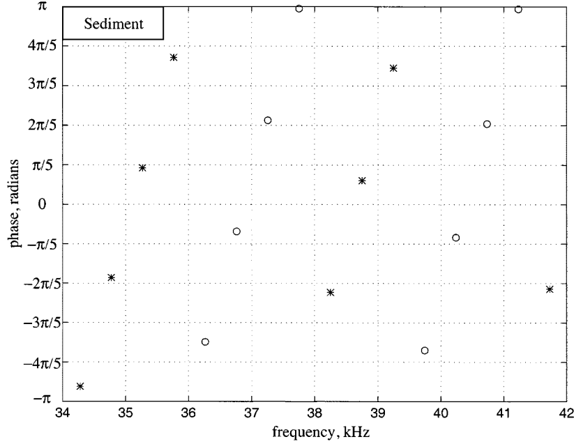
Fig. 12. Four-quadrant phase delay between the two sediment pressure-pulse arrivals in Fig. 8. On passing through a discontinuity in the phase, the symbol changes from an asterisk to an open circle or vice-versa .
