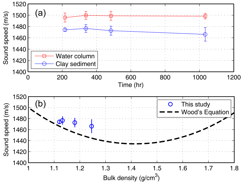
Fig. 5-7. (a) Sound speed in the consolidating clay bed and the overlying water; (b) bulk density versus sound speed in clay-water mixture.
