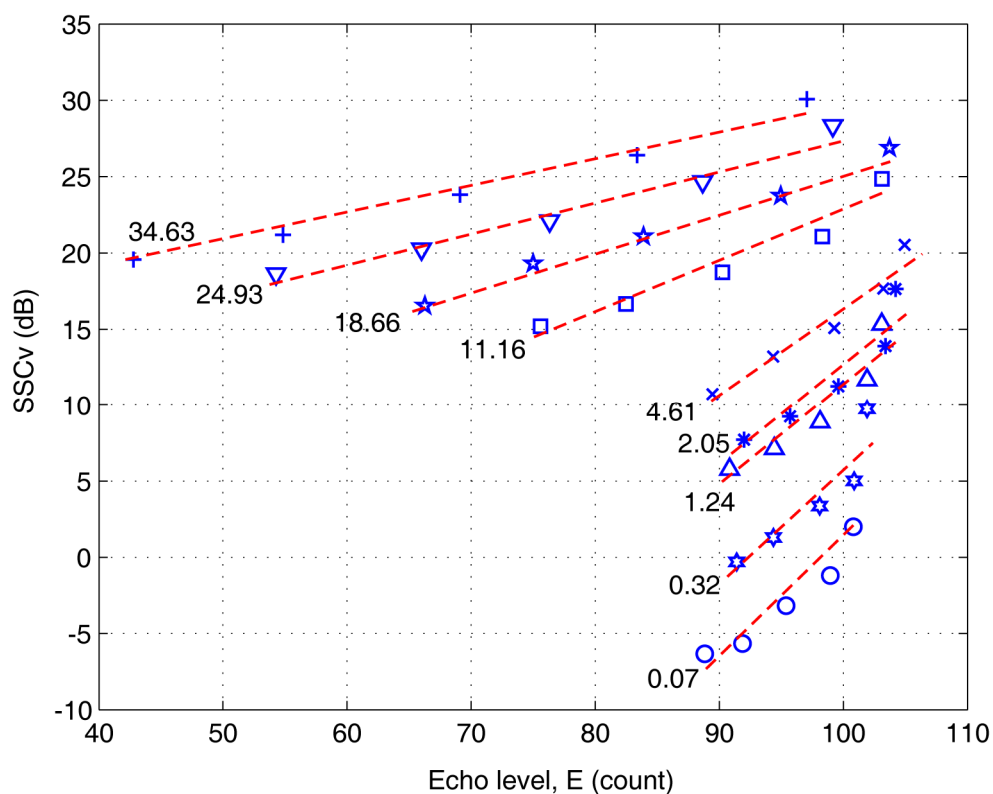
Fig. 3-8. Calibration results for kaolinite. Numbers indicate the suspended sediment concentration (in g/L). The lowest and highest echo levels at each concentration indicate the signals from the range of 59 and 19 cm, respectively.
