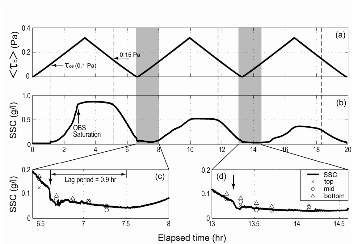
Fig. 4-5. Experiment results from the first simulated tidal cycles. (a) \langle \tau_b \rangle ; and (b) OBS-derived SSC. (c) and (d) are details of the shaded areas in the second panel. The symbols represent the sample-derived SSC at three different levels.
