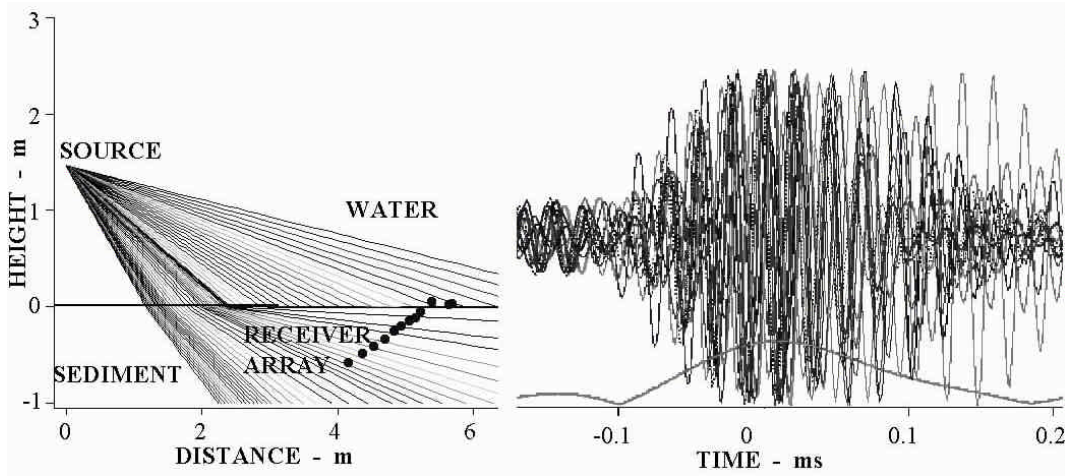
Figure 3. Illustration of refraction modeling: raypaths and superposition of experimentally recorded signals in the 40-50 kHz band at a grazing angle of 20^\circ from SAX99; lower trace shows the amplitude of the coherent sum.
