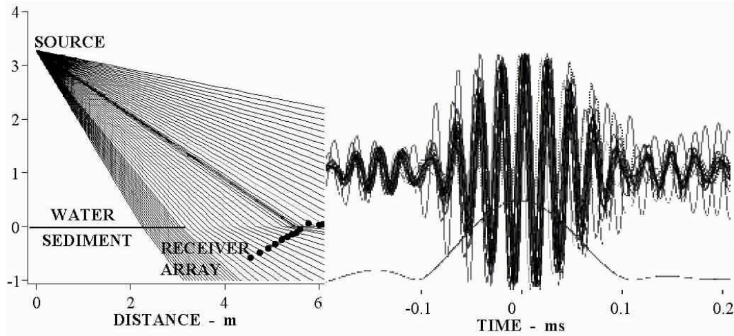
Figure 2. Illustration of refraction modeling: raypaths and superposition of experimentally recorded signals in the 40-50 kHz band at a grazing angle of 30^\circ from SAX99; lower trace shows the amplitude of the coherent sum.
