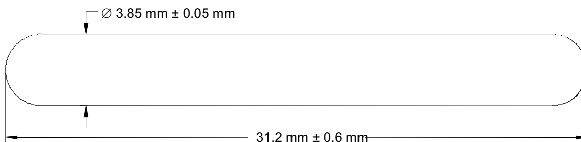
Figure 2-1. Dimensions of the 32-mm Glass Transponder (Read Only, Read/Write)
