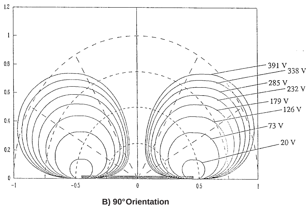
Figure 2-7. Charge-Up Diagram for the G03C Antenna Antenna Voltage From 20 V to 391 V in 53-V Steps (Peak-to-Peak) (Scale in Meters)
