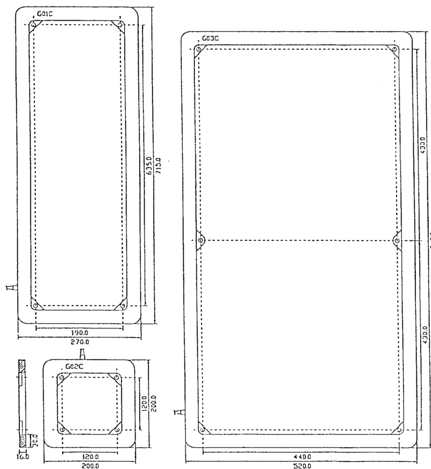
Figure 6-1. Antenna Dimensions
