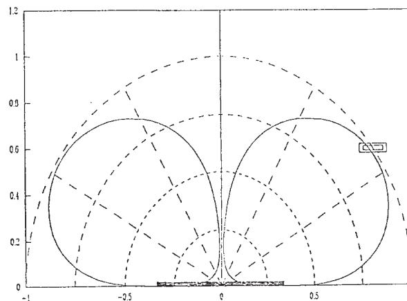
Figure 2-4. 90° Transponder Orientation
