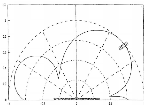
Figure 2-3. 60° Transponder Orientation
