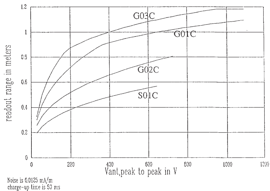
Figure 3-2. Readout Range ( V_{antenna} )
