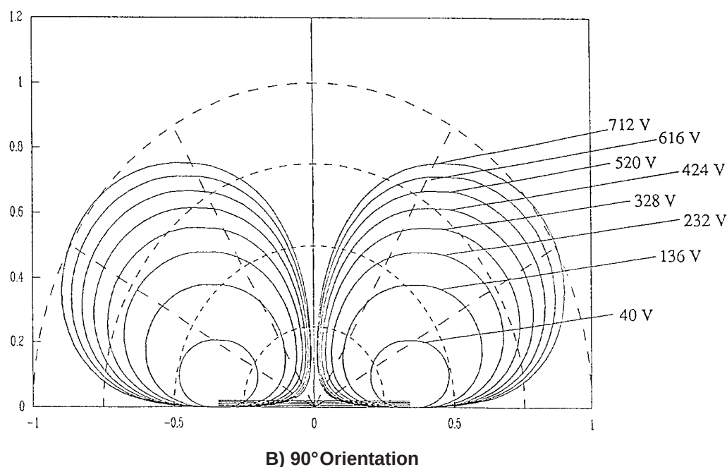
Figure 2-5. Charge-Up Diagram for the G01C Antenna Antenna Voltage From 40 V to 712 V in 96-V Steps (Peak-to-Peak) (Scale in Meters)
