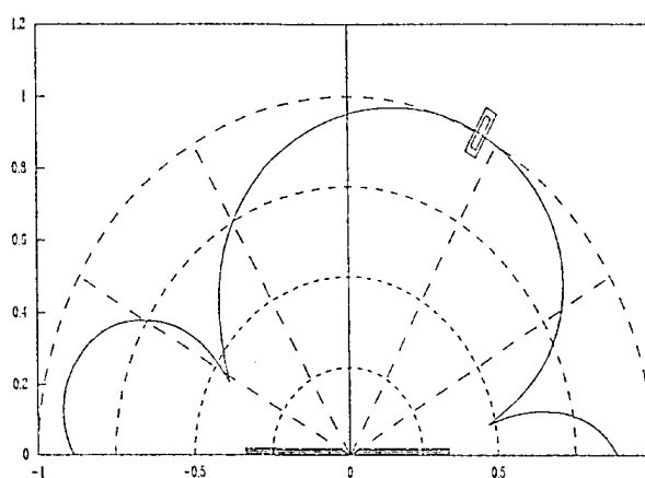
Figure 2-2. 30° Transponder Orientation
