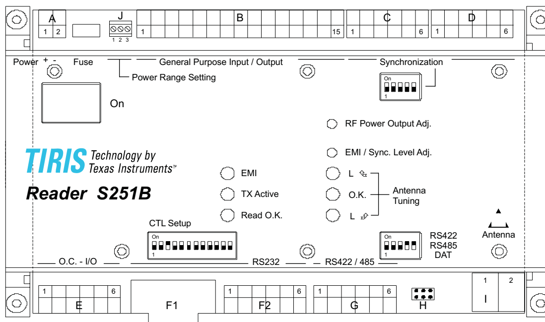
Figure 2-2. S251B Connector Locations
