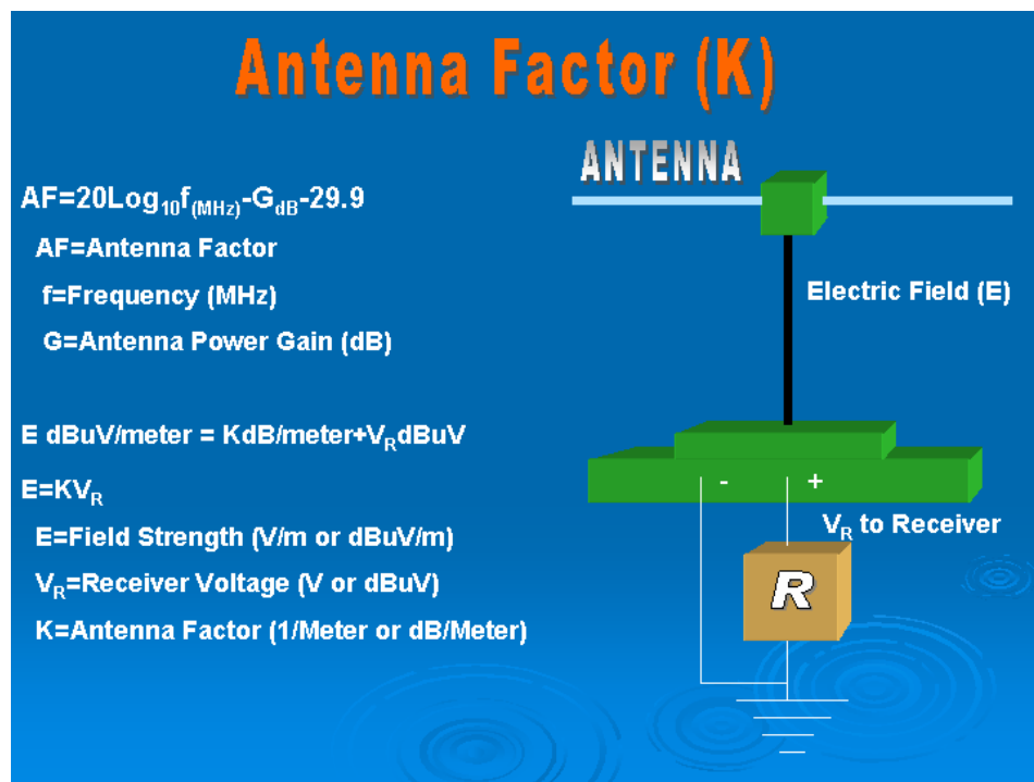
FIGURE 2. ANTENNA FACTOR
