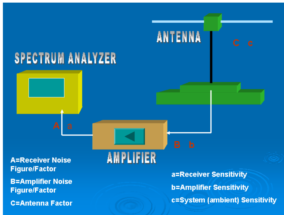
FIGURE 1. RECEIVER SYSTEM BLOCK DIAGRAM
