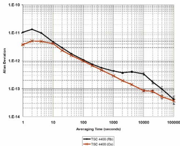
Typical Performance (10 MHz)
