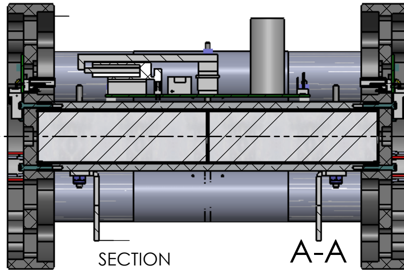
Battery Pack1
