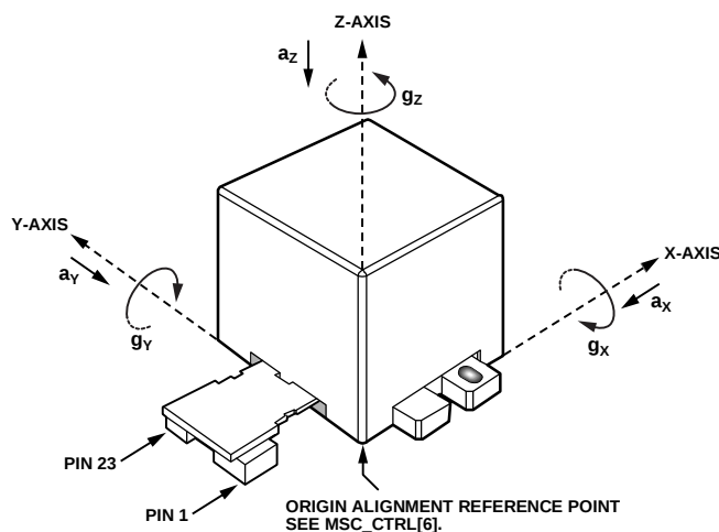
Figure 5. Pin Configuration
