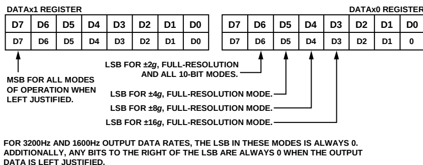
Figure 52. Data Formatting When Output Data Is Left Justified
