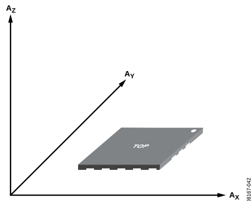
Figure 59. Axes of Acceleration Sensitivity (Corresponding Output Increases When Accelerated Along the Sensitive Axis)
