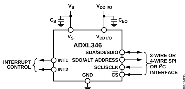
Figure 43. Applications Diagram
