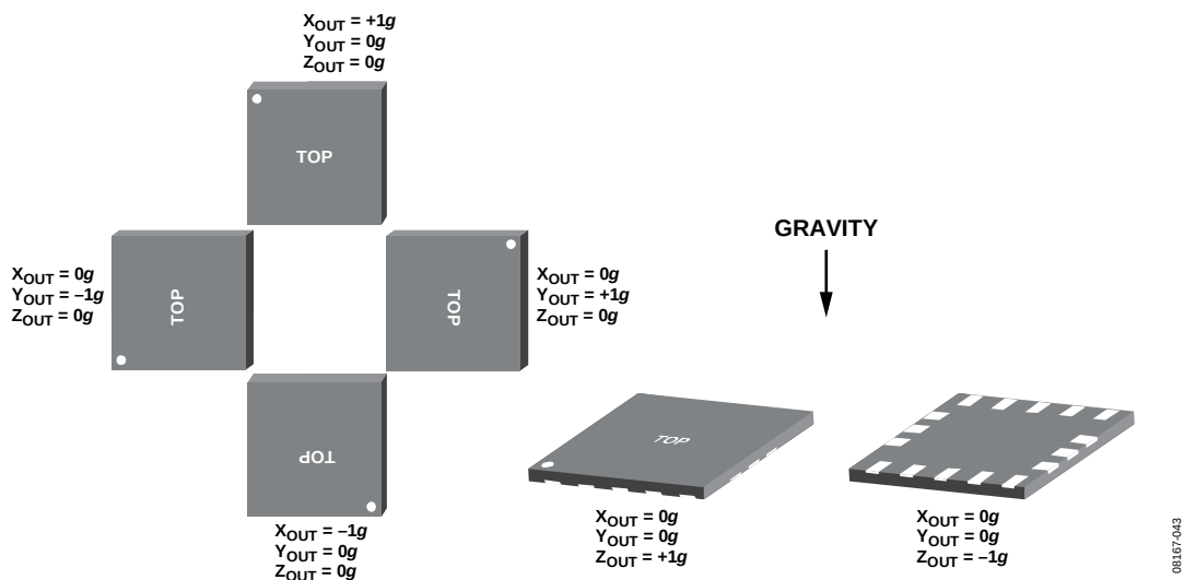
Figure 60. Output Response vs. Orientation to Gravity
