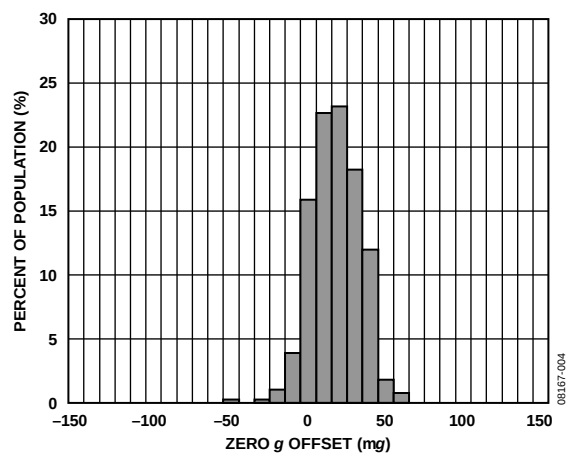
Figure 4. X-Axis Zero g Offset at 25°C, V_S = 2.6\text{ V}
