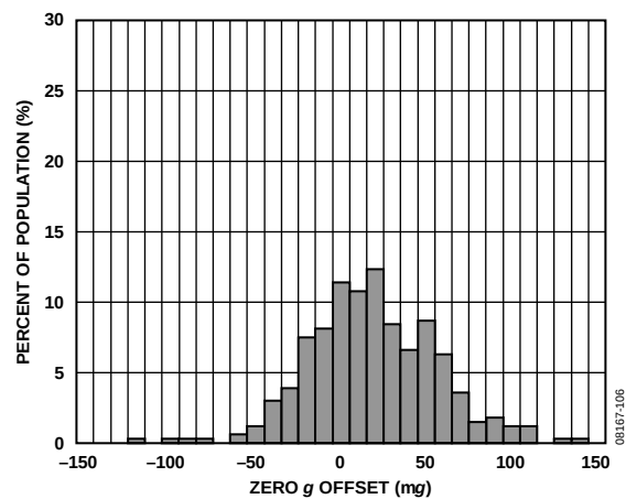
Figure 9. Z-Axis Zero g Offset at 25°C, V_S = 1.8\text{ V}
