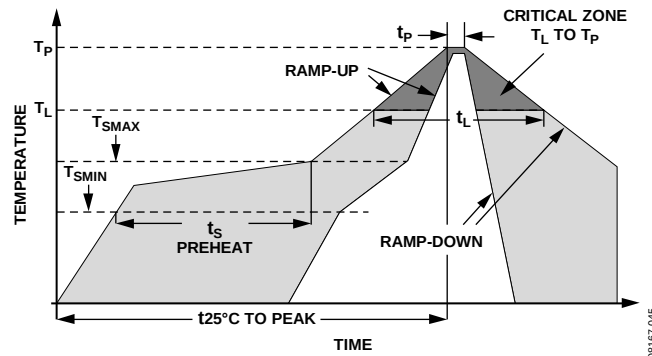
Figure 62. Recommended Soldering Profile
