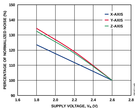
Figure 55. Normalized Noise vs. Supply Voltage
