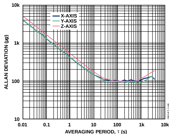
Figure 54. Allan Deviation
