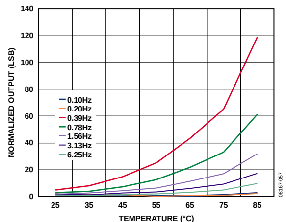
Figure 57. Typical Y-Axis Output vs. Temperature at Lower Data Rates, Normalized to 100 Hz Output Data Rate, V_S = 2.6 V
