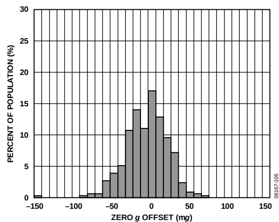
Figure 8. Y-Axis Zero g Offset at 25°C, V_S = 1.8\text{ V}
