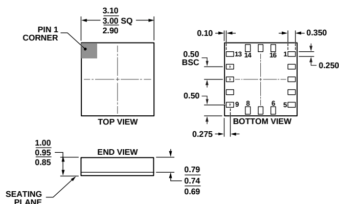
Figure 63. 16-Terminal Land Grid Array [LGA] (CC-16-3)
