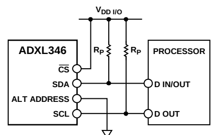
Figure 39. I 2 C Connection Diagram (Address 0x53)
