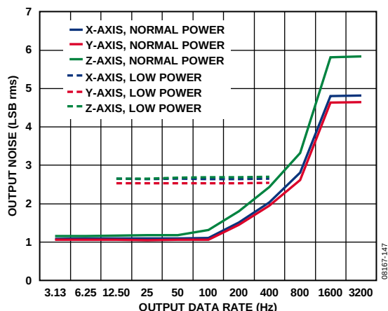
Figure 53. Noise vs. Output Data Rate for Normal and Low Power Modes, Full Resolution (256 LSB/g)
