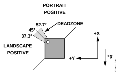
Figure 50. Orientation Showing a 15.4^\circ Dead Zone Region
