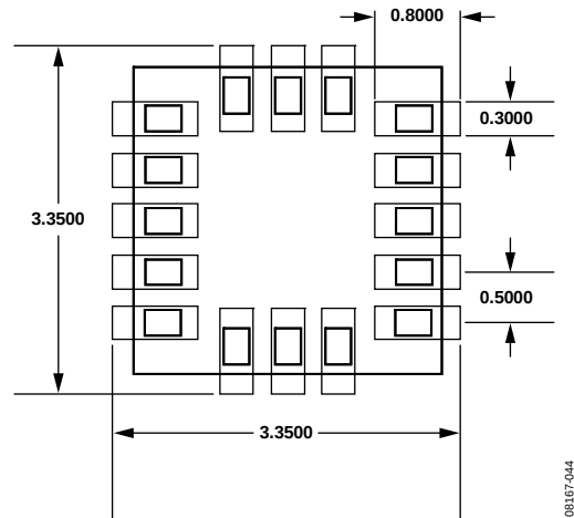
Figure 61. Recommended Printed Wiring Board Land Pattern (Dimensions shown in millimeters)
