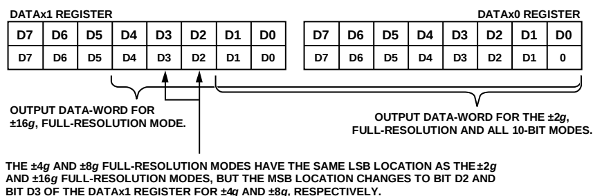
Figure 51. Data Formatting When Output Data Is Right Justified
