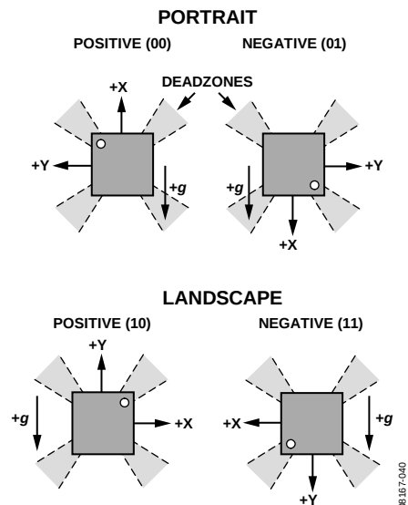
Figure 49. 2D Orientation with Corresponding Codes
