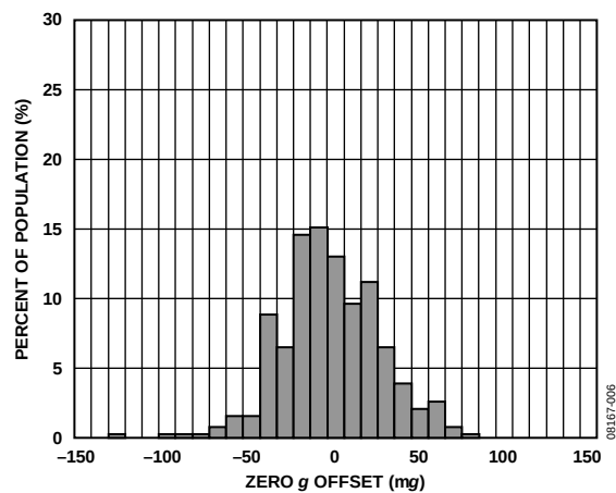
Figure 6. Z-Axis Zero g Offset at 25°C, V_S = 2.6\text{ V}
