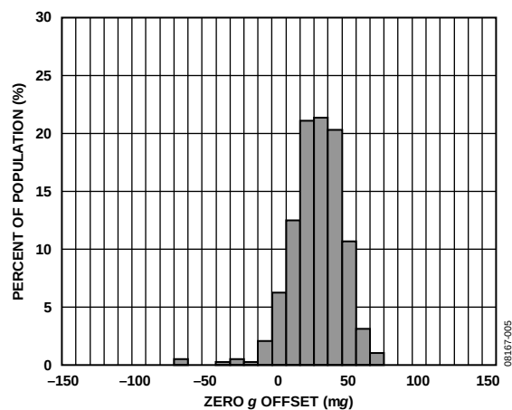
Figure 5. Y-Axis Zero g Offset at 25°C, V_S = 2.6\text{ V}
