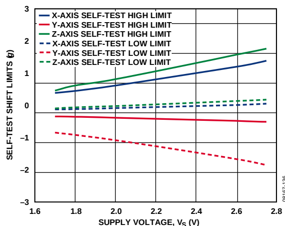
Figure 42. Self-Test Output Change Limits vs. Supply Voltage
