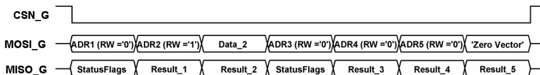
Figure 6. Communication example.
