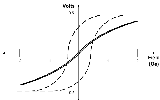
Figure 8. Bridge sensor output for a 12 k \Omega bridge using 10 V bridge excitation. The dotted line is with no field biasing current while the solid line is with 40 mA.
