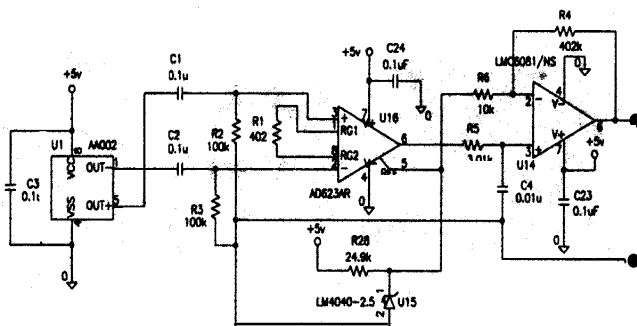
Figure 9. A low-field GMR Wheatstone Bridge sensor with instrumentation amplifier, operational amplifier, and high and low-pass filters.
