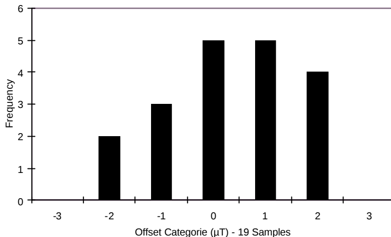
Figure 2.4 Offset distribution( \mu\text{T} ) (@1 MHz , 5V)
