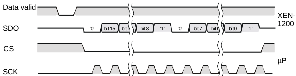
Figure 2.6 SPI/microwire transmission
