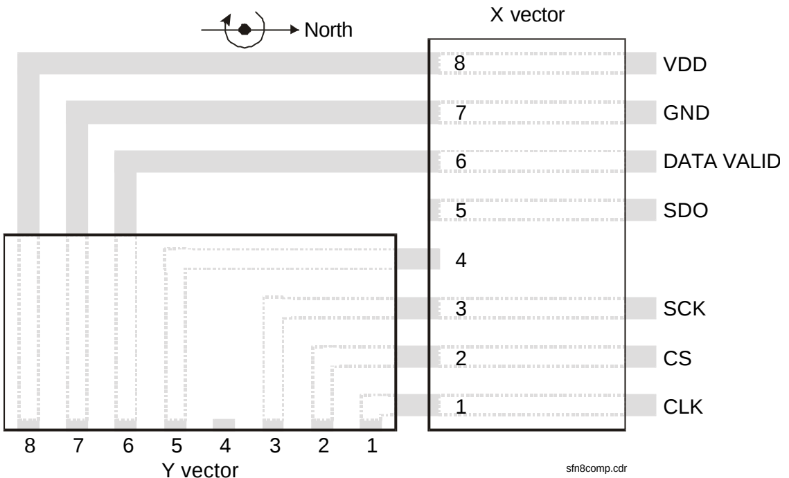
Figure 3.2 Example of PCB connection scheme for two SFN8 packages
