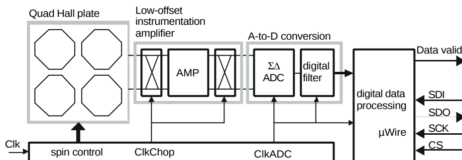
Figure 1.1 XEN-1200 scheme with Quad Hall plate sensor
