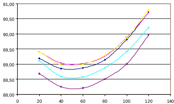
Figure 2.3 Sensitivity temperature drift (@1 MHz , 5V)
