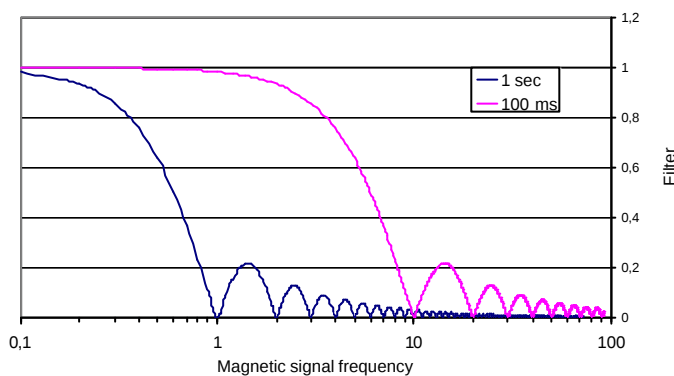
Figure 2.10 Filter characteristics for sine shape signals
