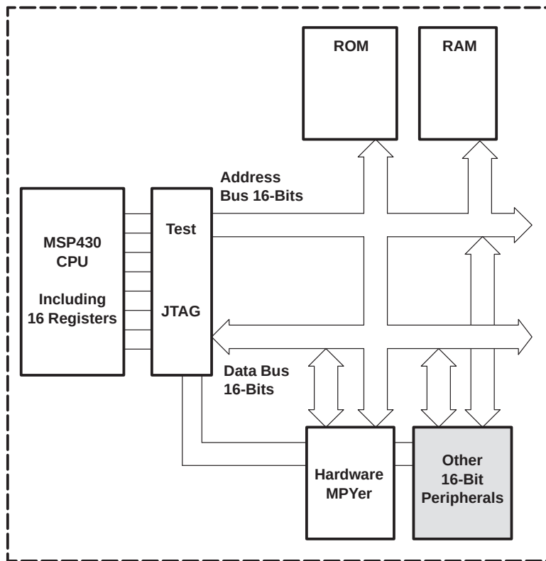
Figure 6–56. The Internal Connection of the MSP430 16 × 16-Bit Hardware Multiplier
