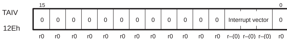
Figure 6–6. Timer Vector Register (TAIV)
