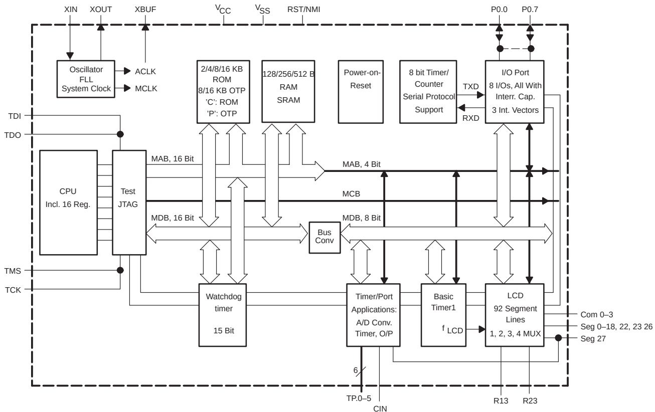
Figure 1–1. MSP430C31x Block Diagram
