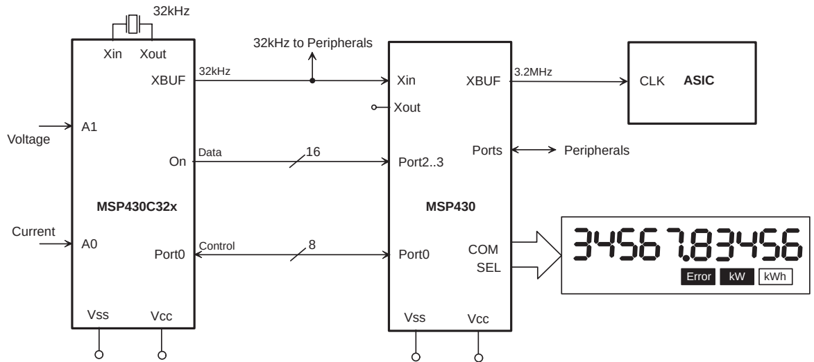
Figure 6–77. Two MSP430s Running From the Same Crystal
