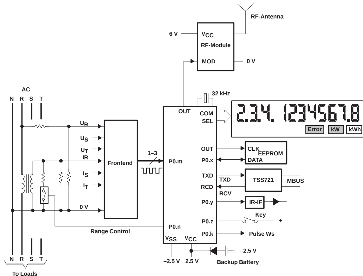
Figure 4–49. MSP430 EE Meter With RF Readout
