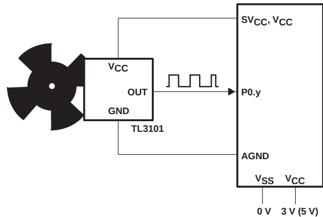
Figure 4–46. Revolution Counter With a Digital Hall Sensor
