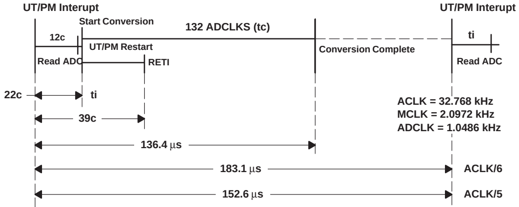
Figure 4–24. Timing for the Reduced Scan Principle
