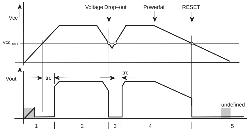
Figure 6–72. System Voltages With a Power Supply Supervisor
