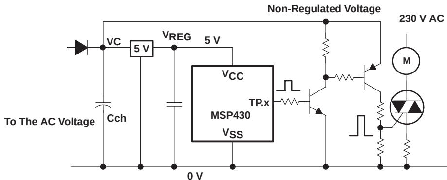
Figure 4–87. Nonregulated Voltage for the TRIAC Control
