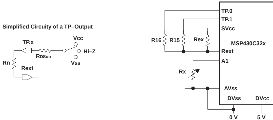
Figure 23. Hardware for a 16-Bit ADC
