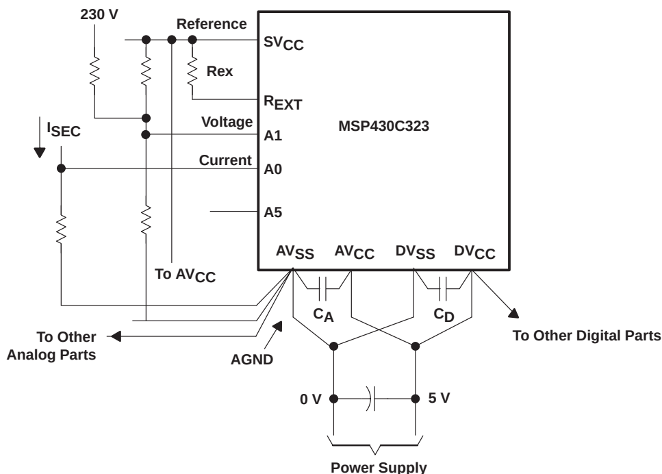
Figure 4–7. MSP430 14-Bit ADC Grounding
