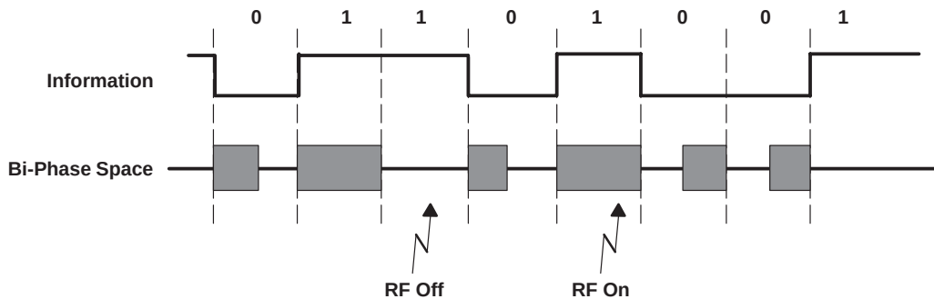
Figure 5–17. Biphase Space Code
