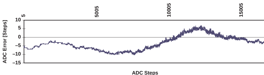
Figure 38. Error Characteristic Device 4
