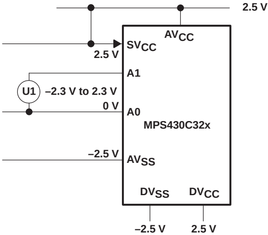
Figure 4–8. Split Power Supply for Level Shifting
