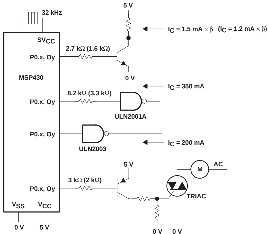
Figure 3–3. Output Buffering
