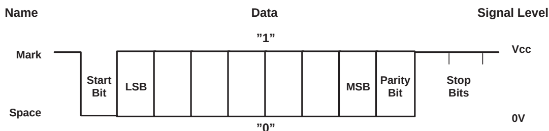
Figure 6–81. The RS232 Format (Levels at the MSP430)
