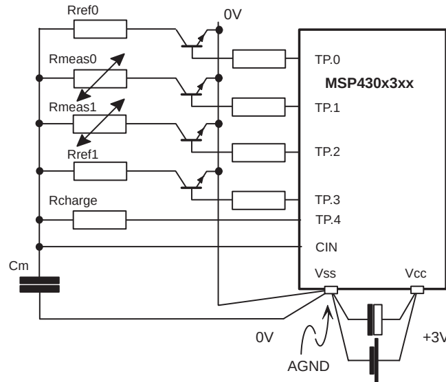
Figure 17. Hardware Schematic for Low-Resistive Sensors
