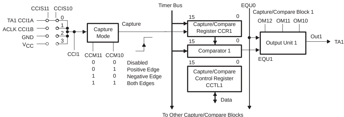
Figure 6–8. Capture/Compare Block 1
