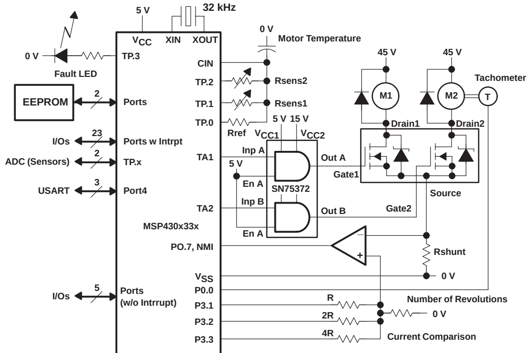
Figure 4–75. Control for Two MOSFET Output Stages
