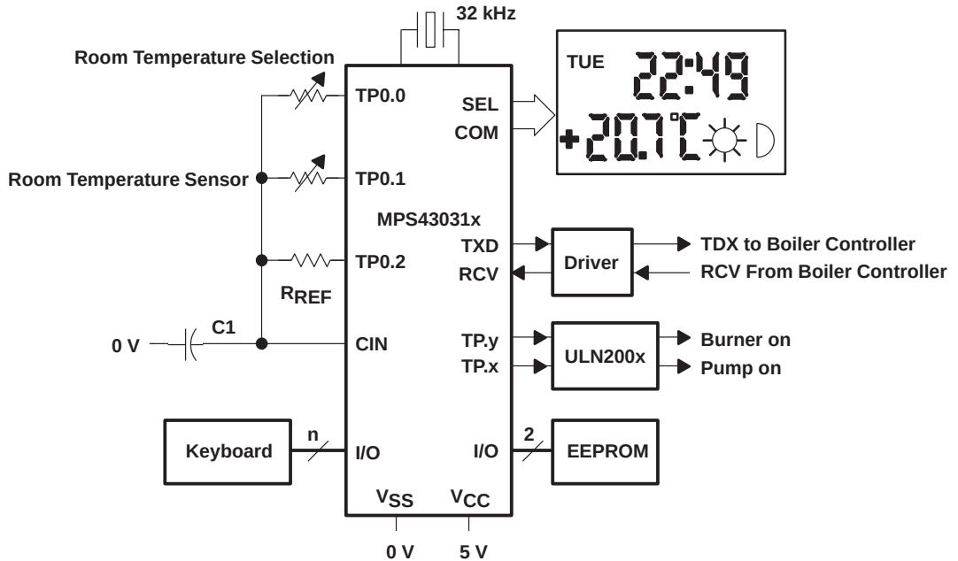
Figure 4–62. Heating Installation Controller for a Single-Family Home
