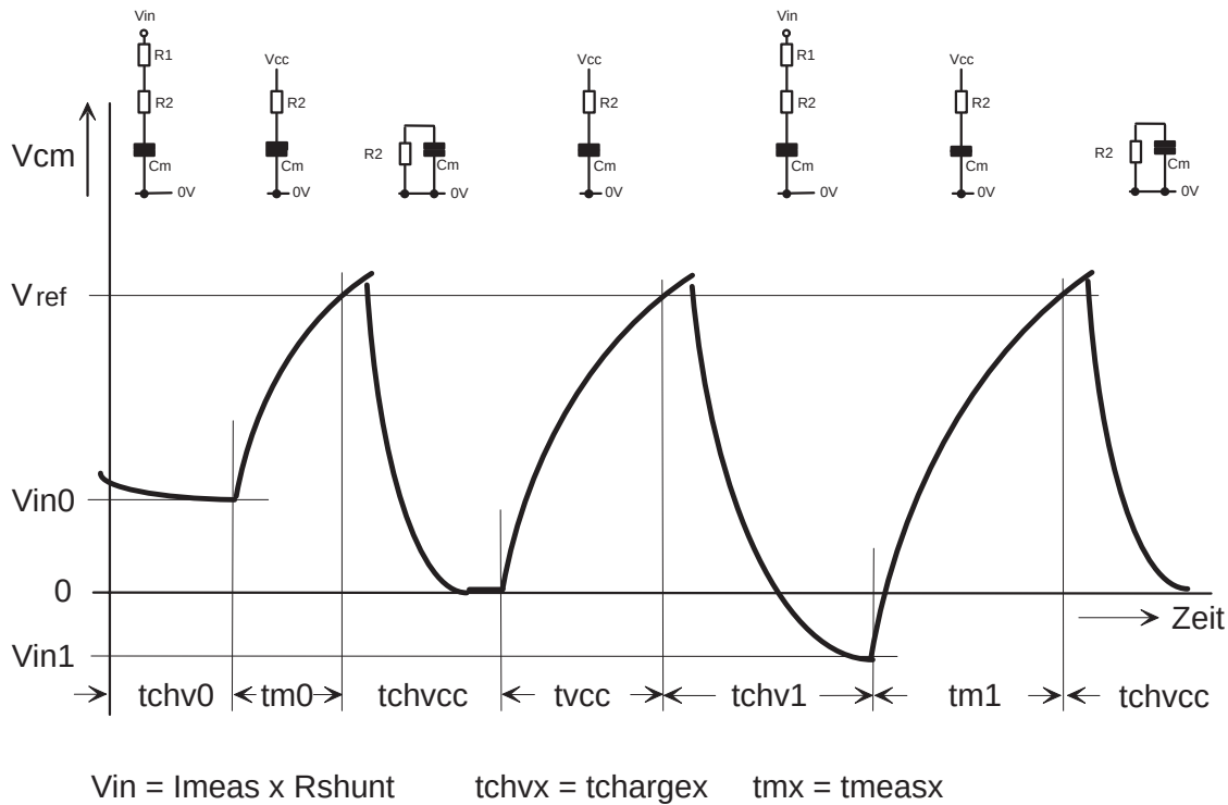
Figure 14. Current Measurement
