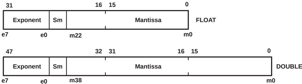
Figure 5–20. Floating Point Formats for the MSP430 FPP
