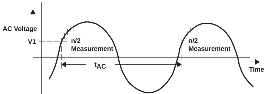
Figure 5–12. Reduction of Hum by Synchronizing to the AC Frequency. Differential Measurement
