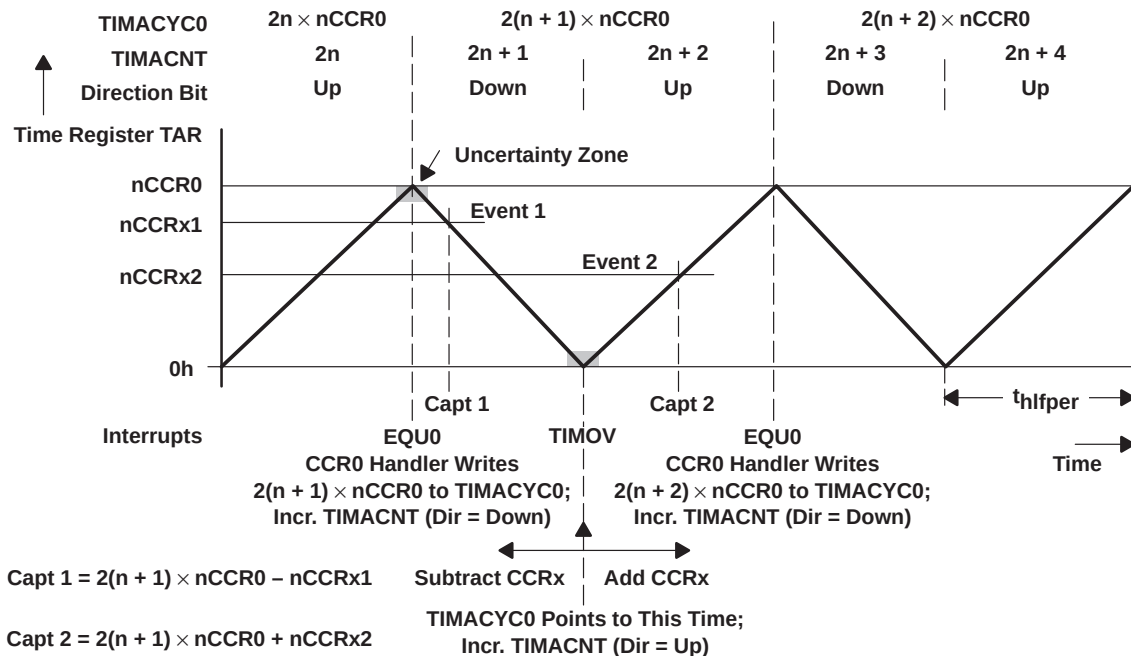
Figure 6–52. Capturing With the Up/Down Mode
