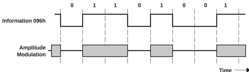
Figure 6–33. Amplitude Modulation
