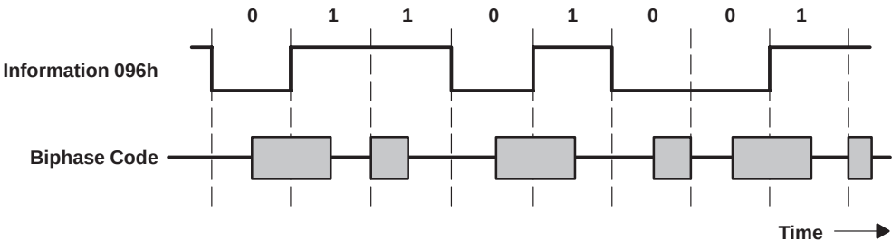
Figure 6–34. Biphase Code Modulation
