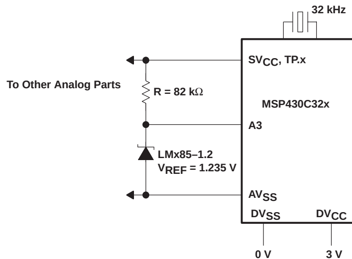
Figure 5–31. Connection of the Voltage Reference
