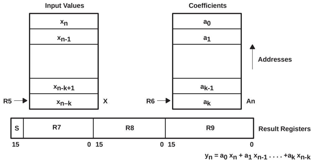
Figure 6–60. Storage for the Finite Impulse Response Filter
