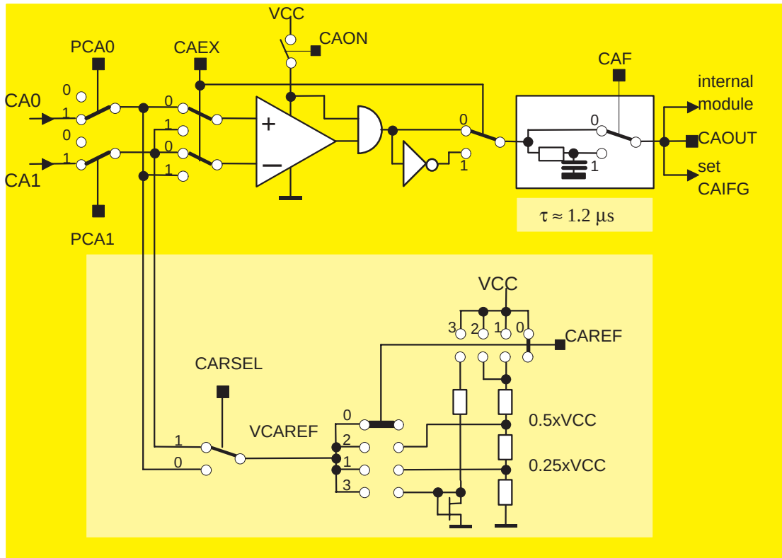
Figure 6–97. Comparator_A Hardware
