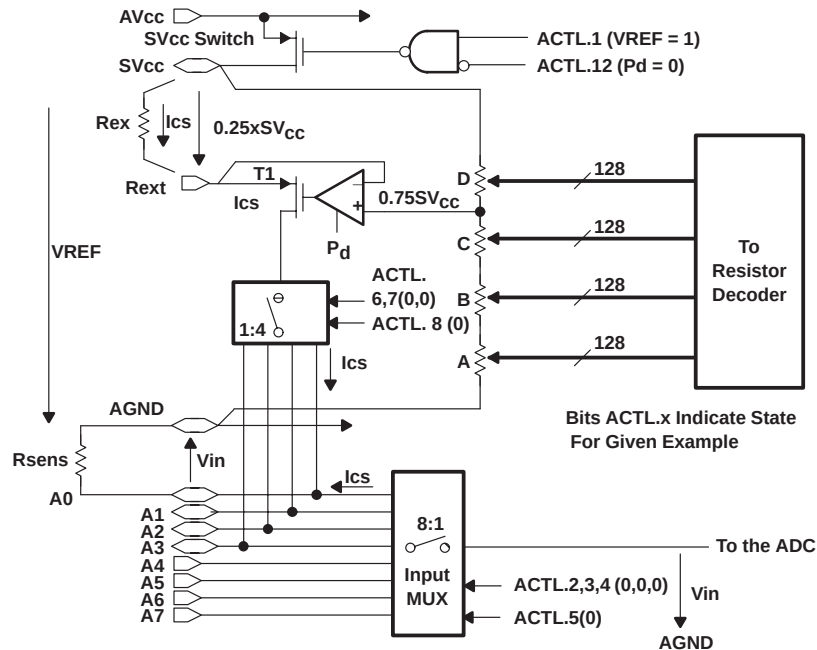
Figure 26. The Current Source
