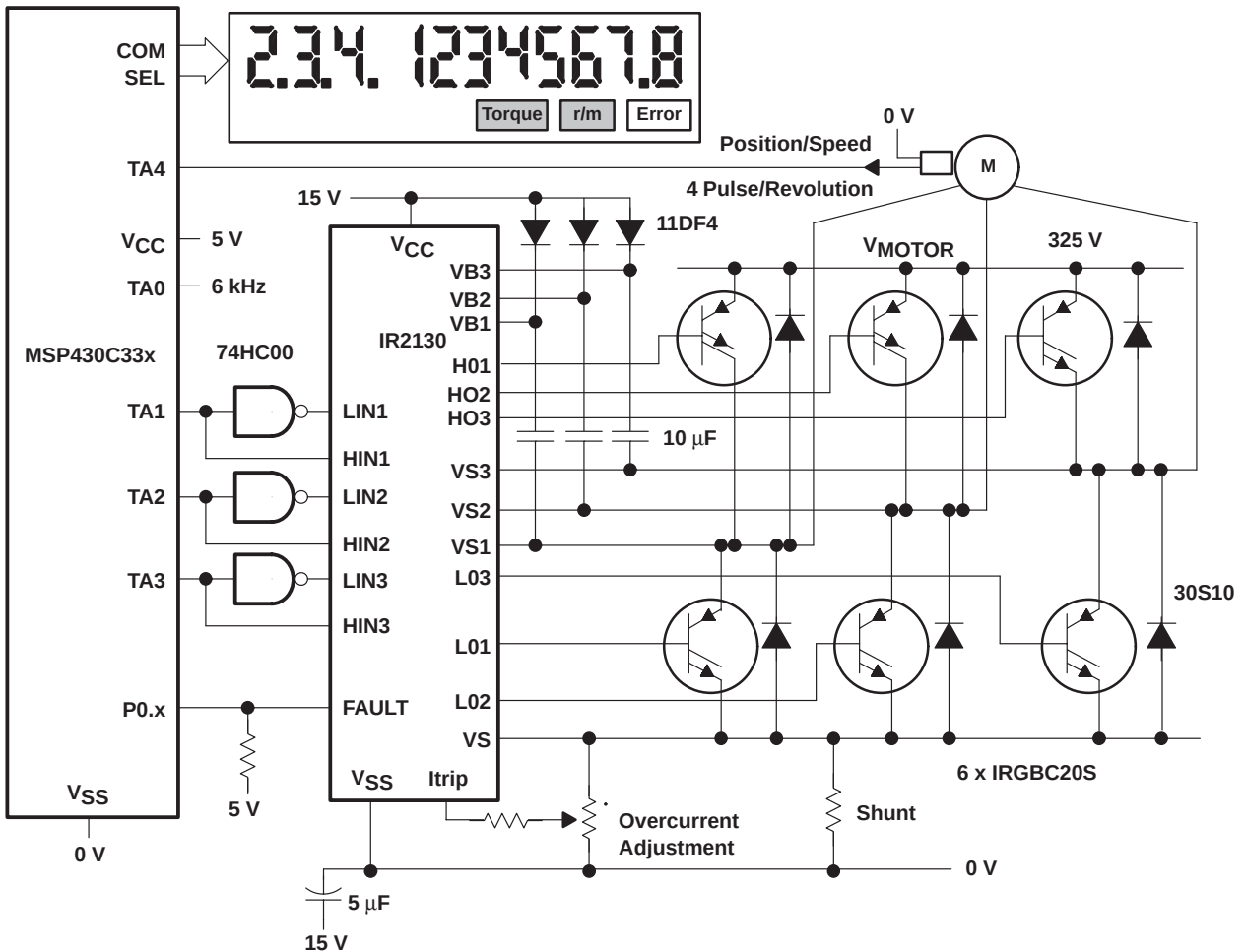
Figure 6–47. PWM Motors Control for High Motor Voltages
