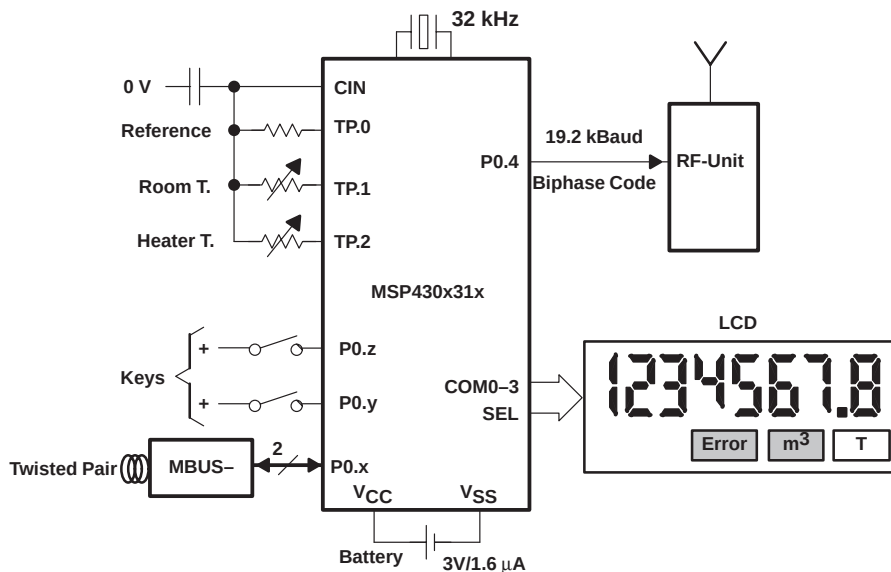
Figure 4–33. Electronic Heat Allocation Meter With MSP430C31x
