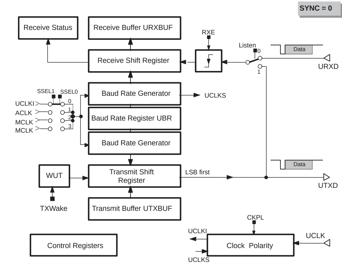
Figure 6–80. The USART Switched to the UART Mode
