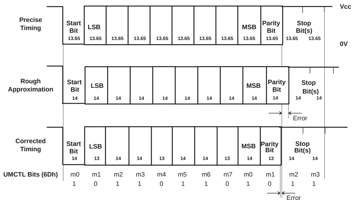
Figure 6–85. Baud Rate Correction Function
