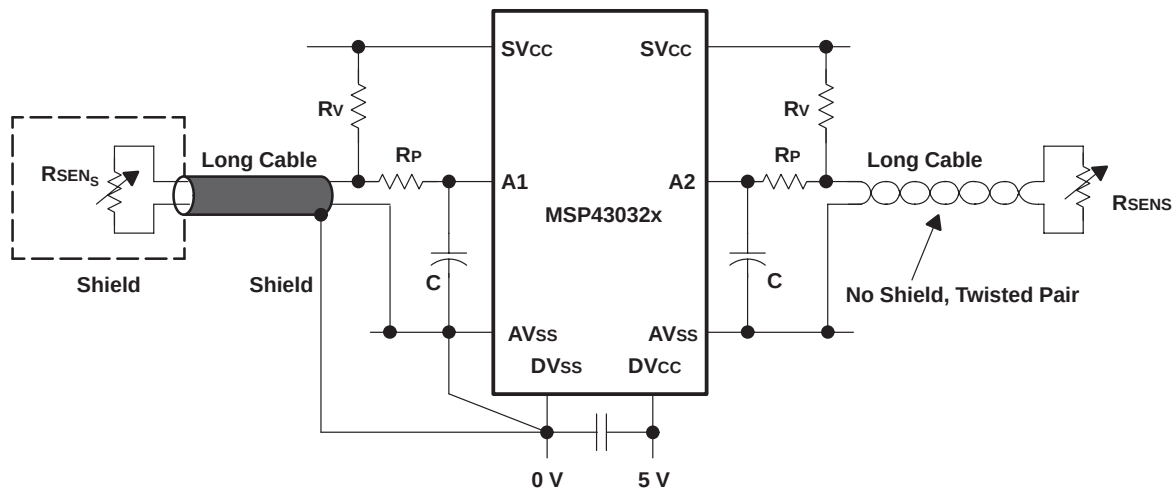
Figure 18. Sensor Connection via Long Cables With Voltage Supply
