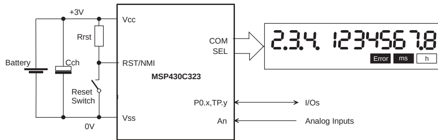
Figure 6–66. Battery-Powered System With RESET Switch
