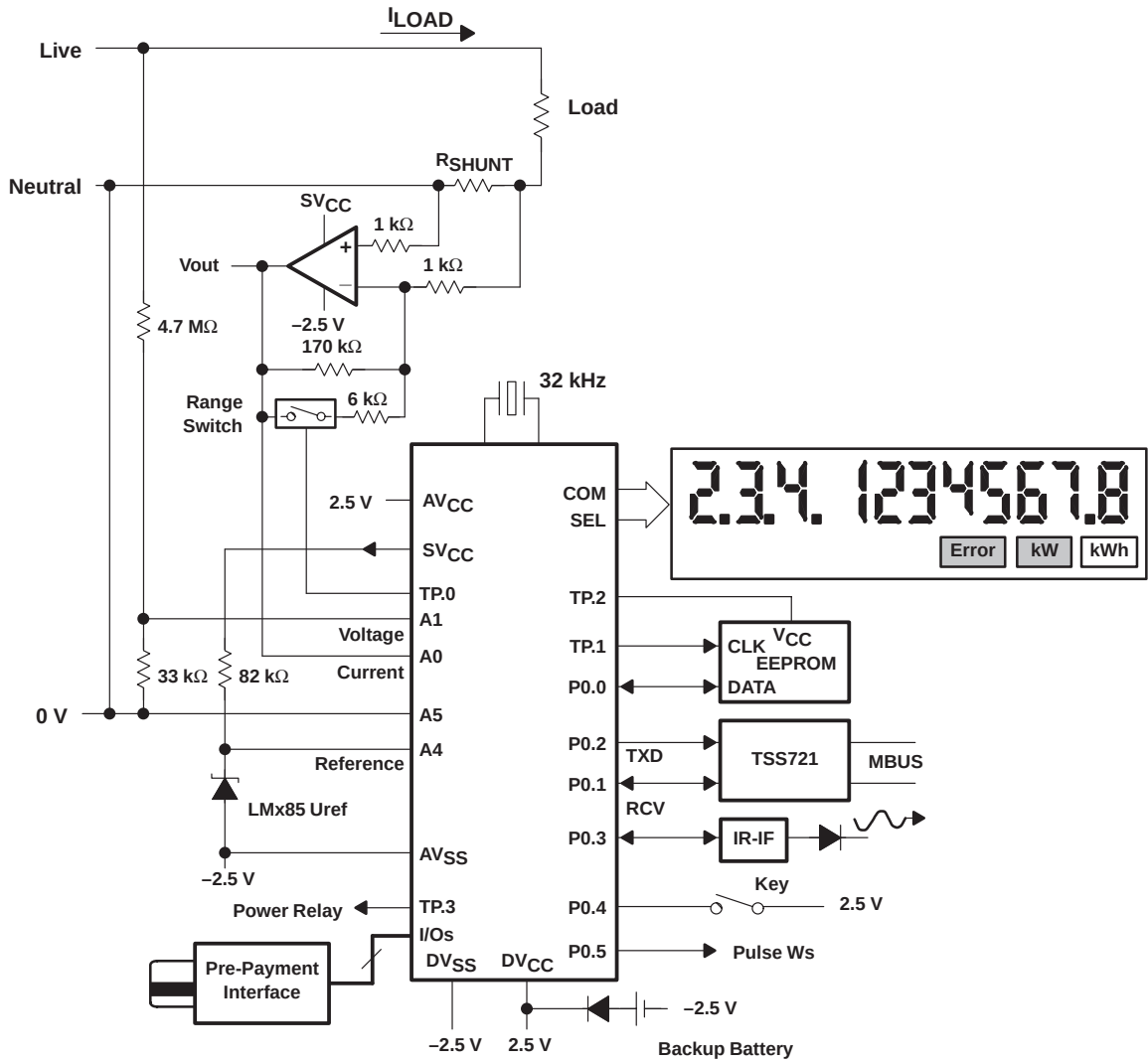
Figure 4–15. Single-Phase Electricity Meter With Shunt Resistor
