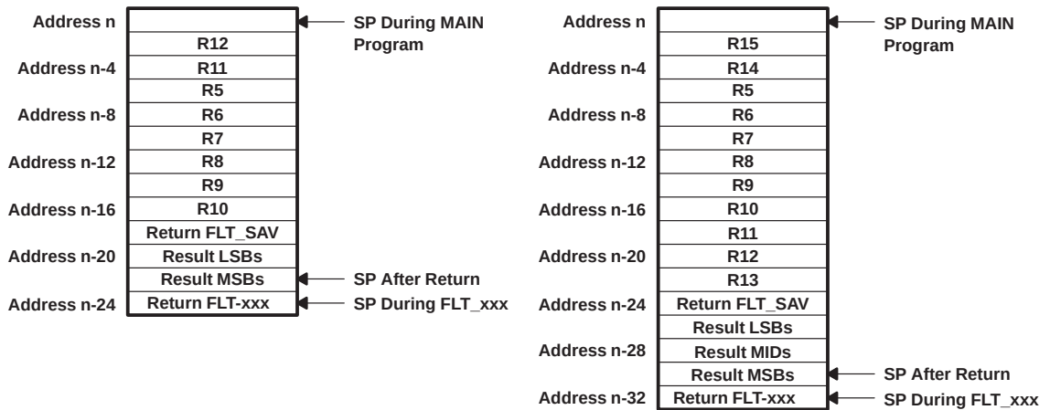
Figure 5–19. Stack Allocation for .FLOAT and .DOUBLE Formats
