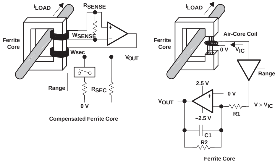
Figure 4–13. Current Measurement With a Ferrite Core
