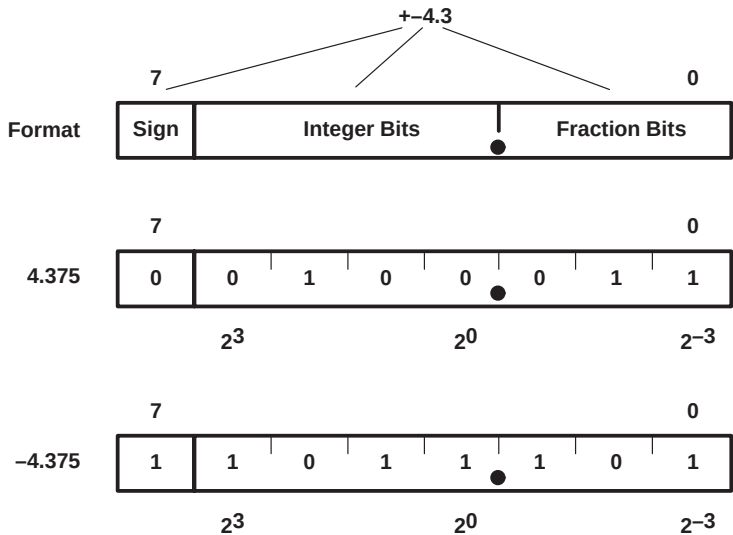
Figure 7. Number Format With Integers for 8-Bit Calculations
