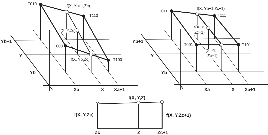
Figure 5–9. Algorithm for a Three-Dimensional Table
