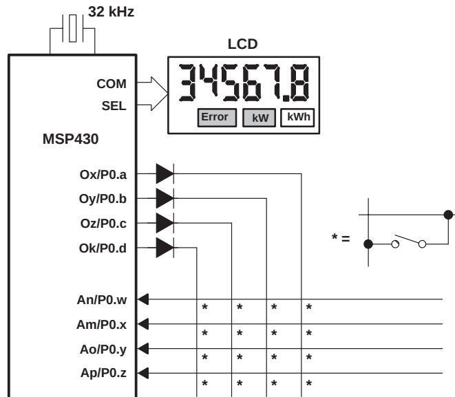
Figure 5–13. Keyboard Connection to MSP430
