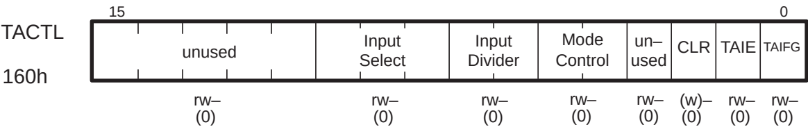
Figure 6–5. Timer Control Register (TACTL)
