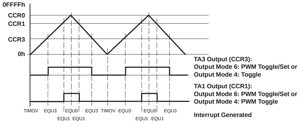
Figure 3–19. PWM Generation with Up-Down Mode
