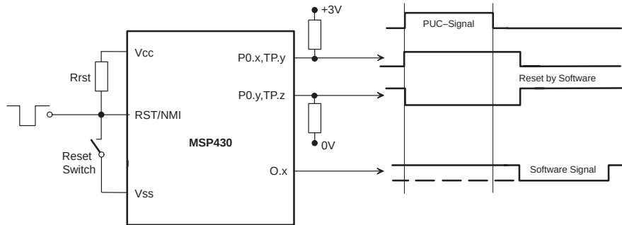
Figure 6–65. Generation of RESET–Signals for External Peripherals
