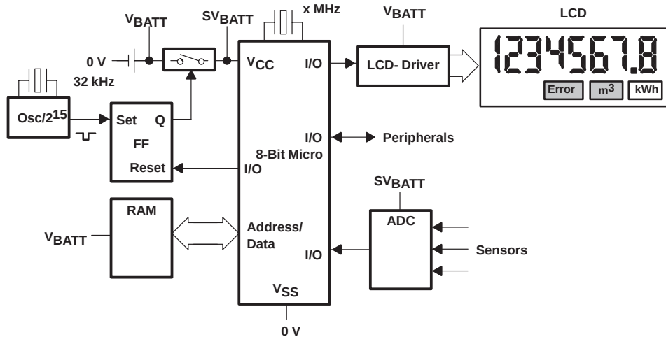
Figure 4–55. Conventional Solution for a Battery-Driven System
