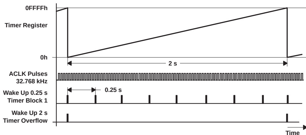
Figure 6–36. Real Time Clock Application of the Timer_A
