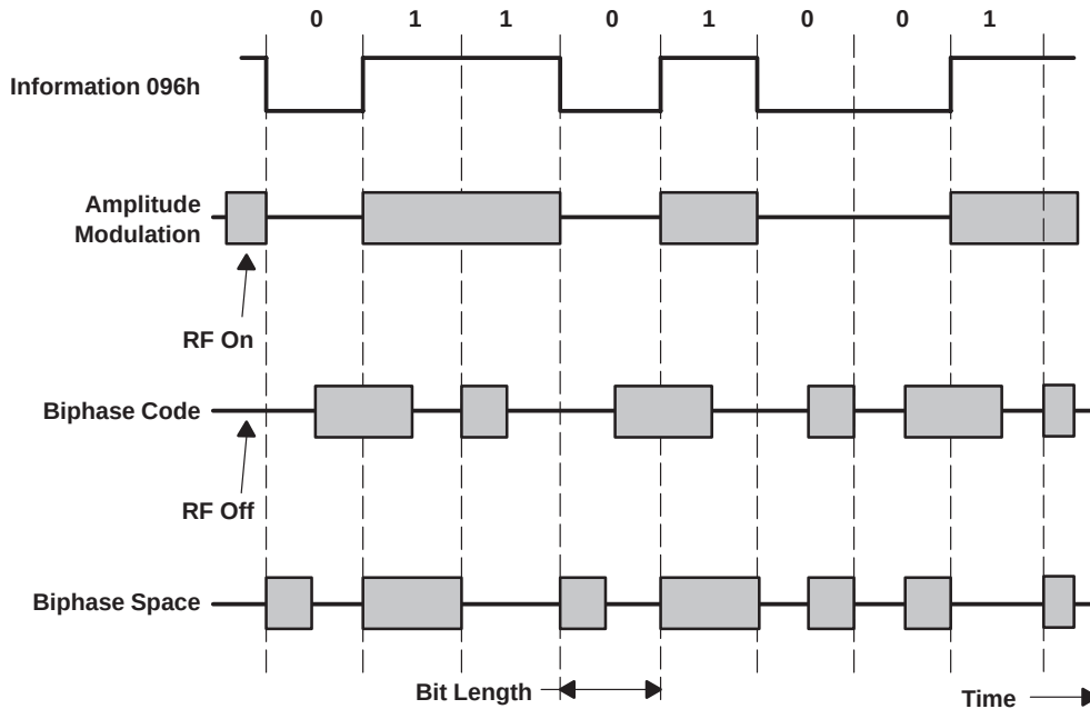
Figure 6–32. RF Modulation Modes
