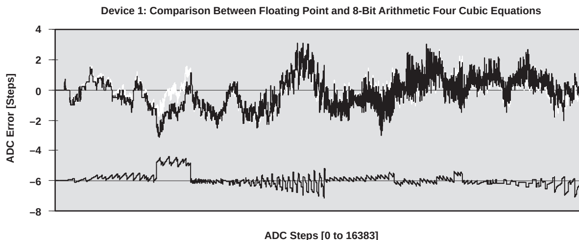
Figure 11. Comparison of Corrected ADC Characteristics. 8-Bit Results Before Rounding
