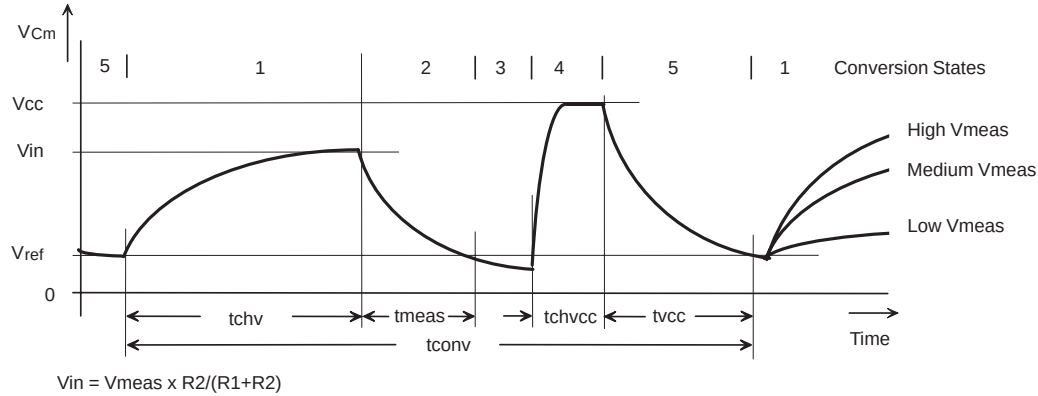
Figure 11. Voltage Measurement
