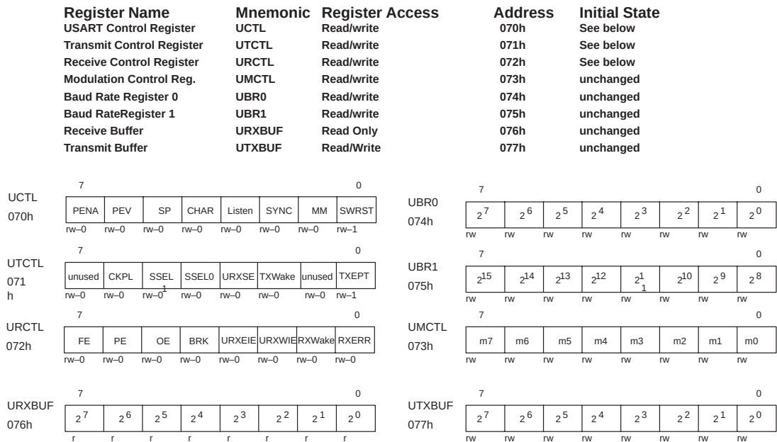
Figure 6–83. USART Control Registers Used for the UART Mode
