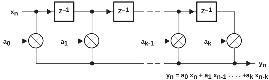
Figure 6–59. Finite Impulse Response Filter
