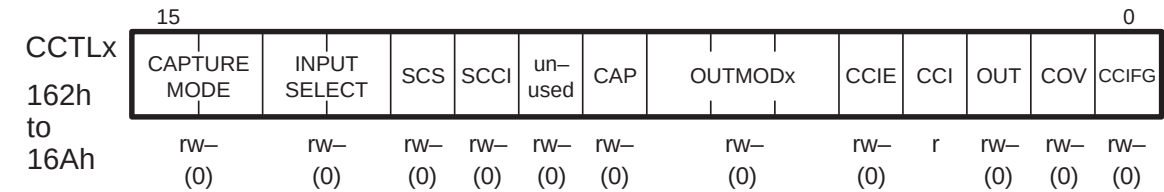
Figure 6–11. Timer Control Registers (CCTLx)
