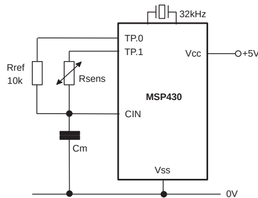
Figure 15. Temperature Measurement
