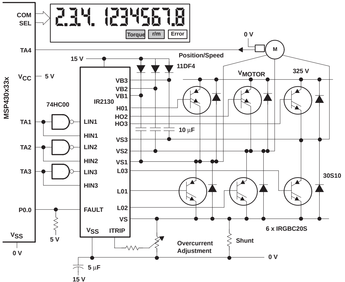
Figure 4–82. PWM Motors Control for High Motor Voltages
