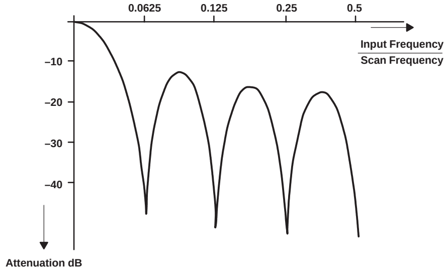
Figure 5-10. Frequency Response of the Continuous Averaging Filter
