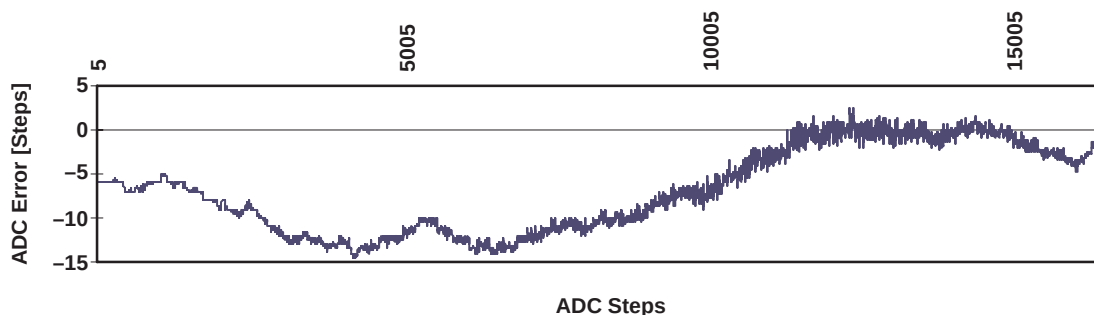
Figure 35. Error Characteristic Device 1
