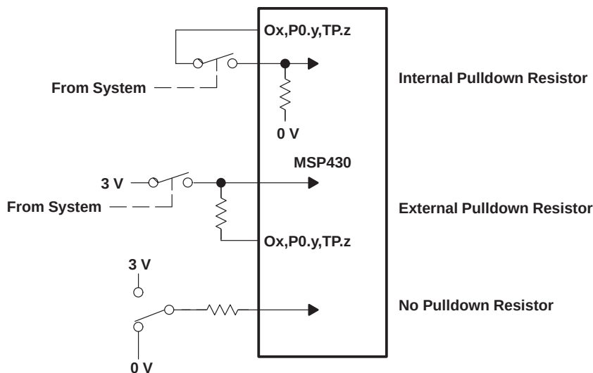
Figure 4–59. Connection of Keys to Inputs
