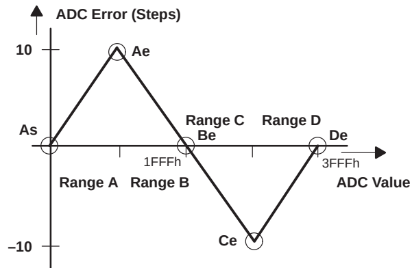
Figure 4–27. Explanation of the ADC Deviation
