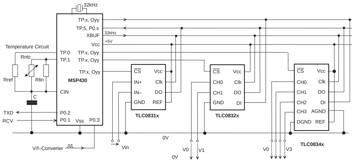
Figure 21. Analog-to-Digital Conversion With External ADCs
