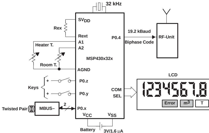
Figure 4–32. Electronic Heat Allocation Meter With MSP430C32x
