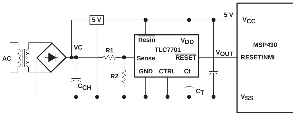
Figure 5–40. Power-Fail Detection with a Supply Voltage Supervisor
