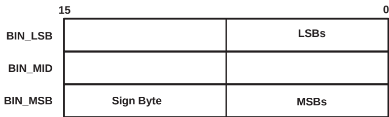
Figure 5–26. Binary Number Format 48 Bit
