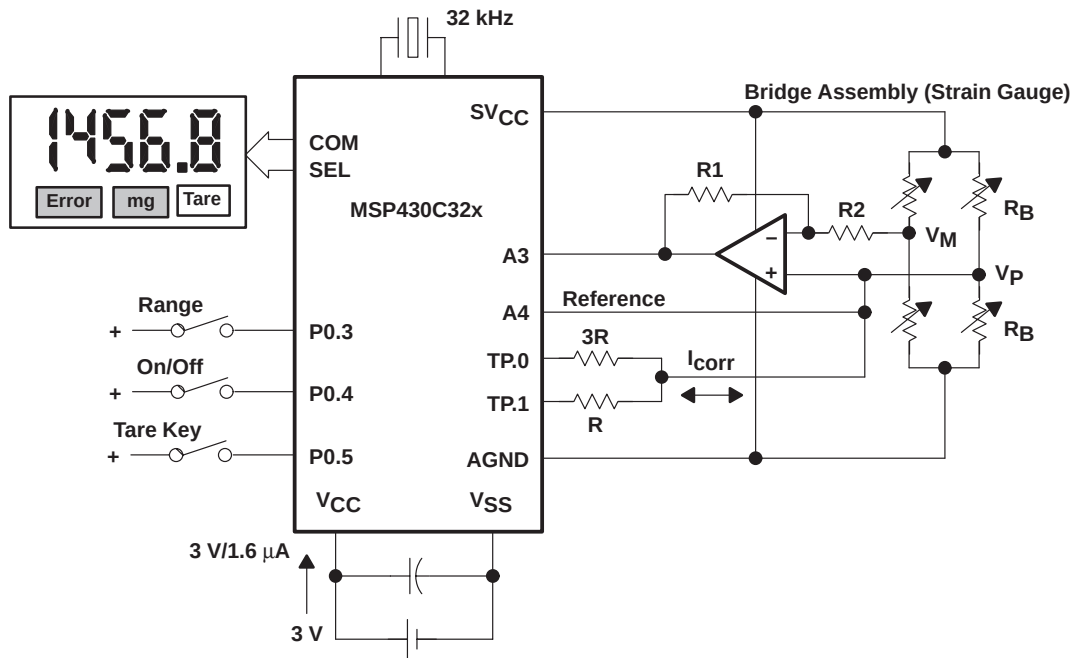
Figure 4-63. Simple Battery Driven Scale
