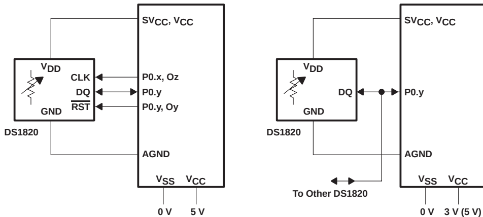
Figure 4–44. Connection of Digital Sensors (Thermometer)
