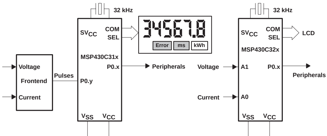
Figure 4–1. Two Measurement Methods for Electronic Electricity Meters
