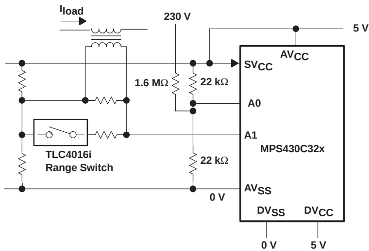
Figure 4–10. Resistor Interface Without Current Source
