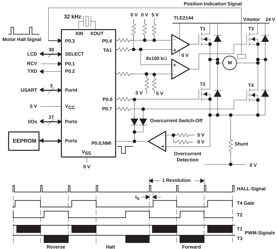
Figure 4-77. PWM Motor Control for Brushless DC Motor
