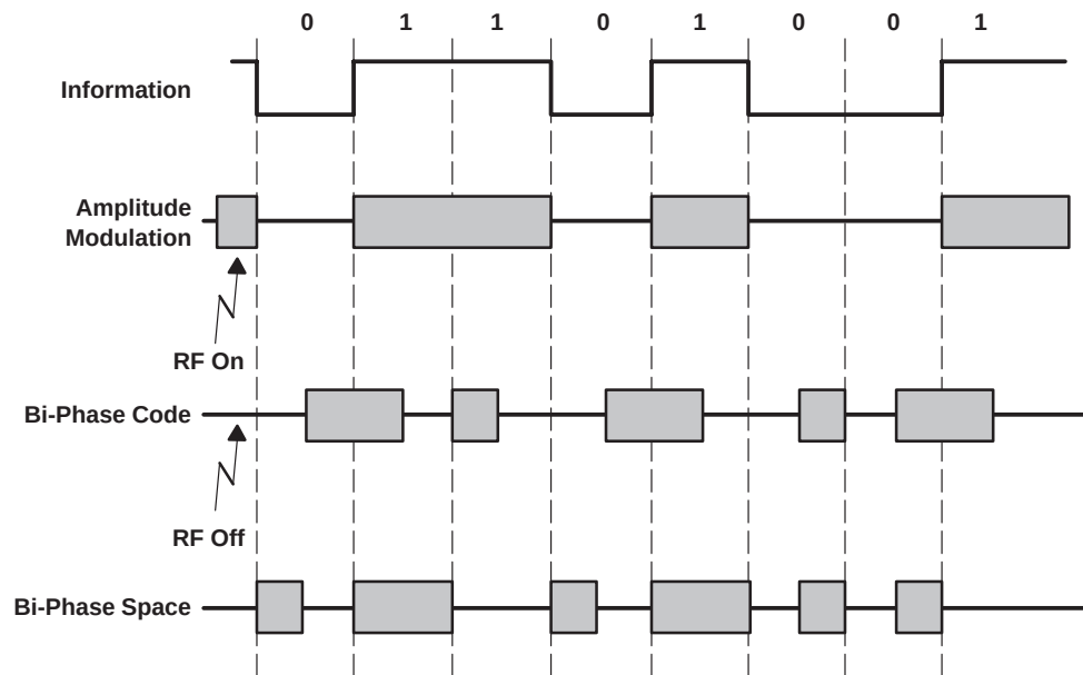
Figure 4–52. RF-Modulation Modes
