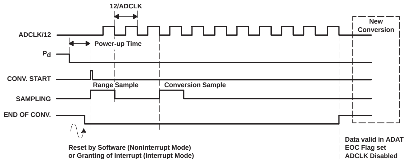
Figure 9. Timing for the 14-bit Analog-to-Digital Conversion
