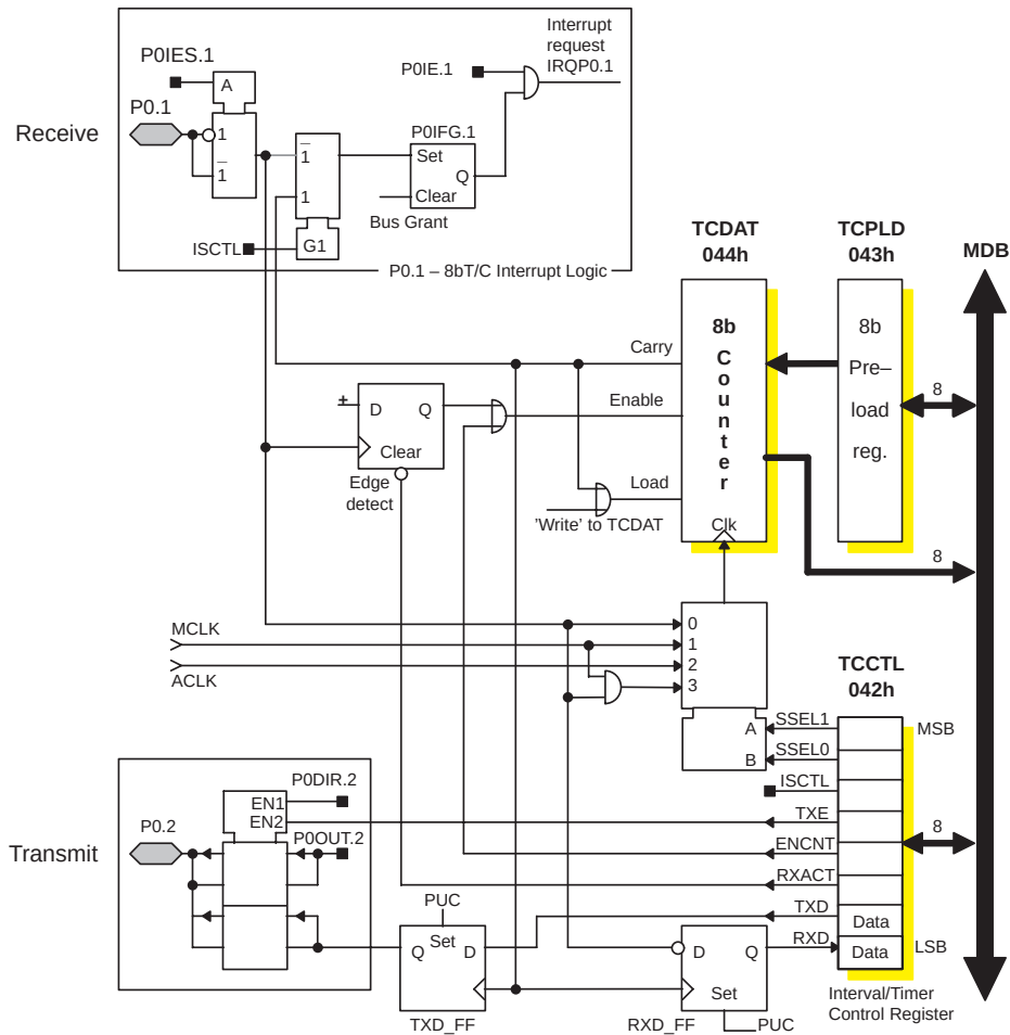
Figure 6–86. MSP430 8-Bit Interval Timer/Counter Module Hardware
