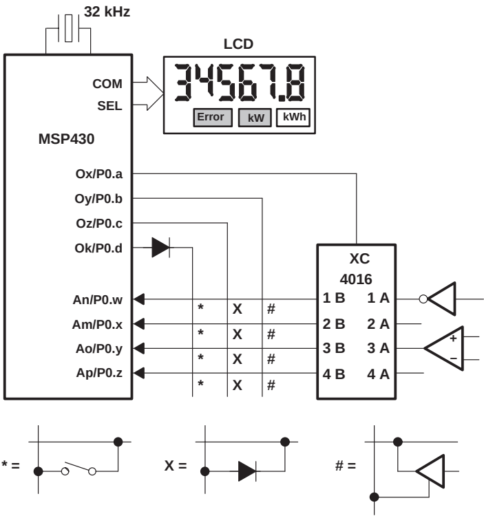
Figure 5–14. Connection of Different Input Signals
