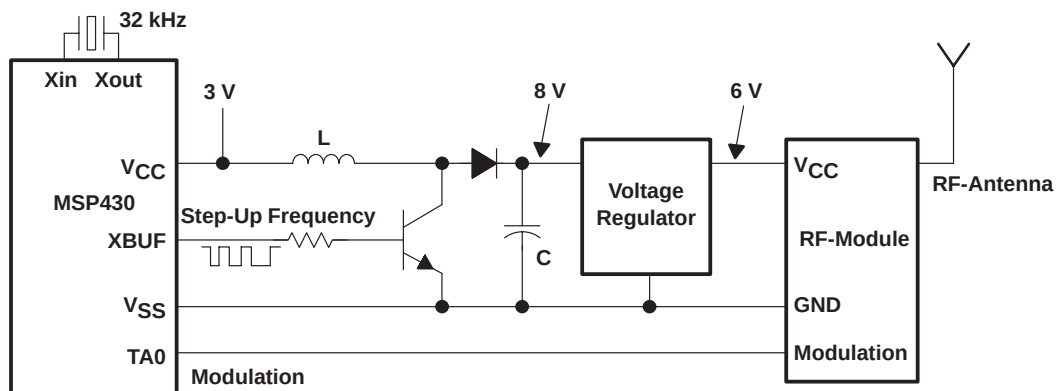
Figure 6–31. RF Interface Module Connection to the MSP430
