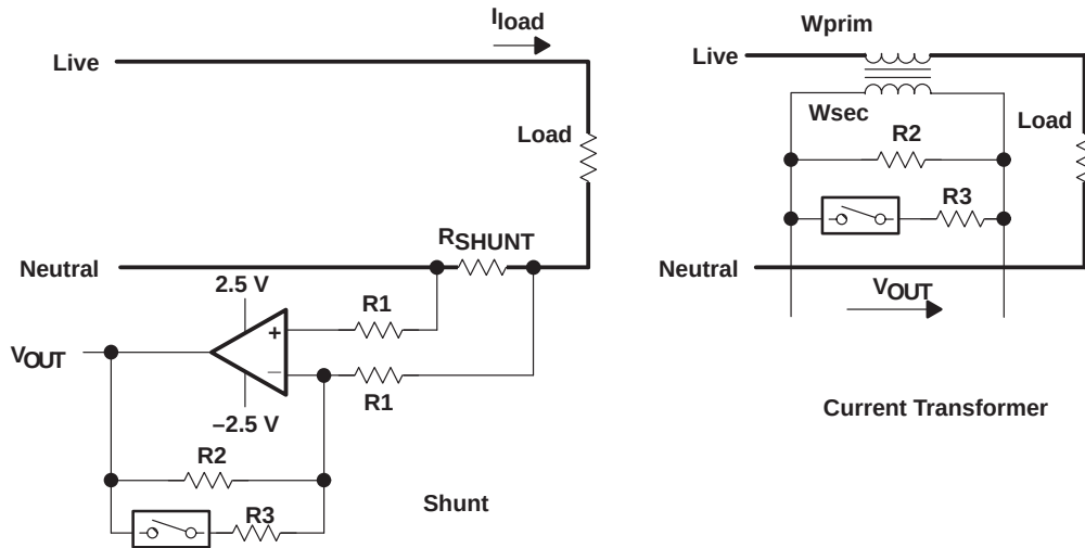
Figure 4-12. Current Measurement
