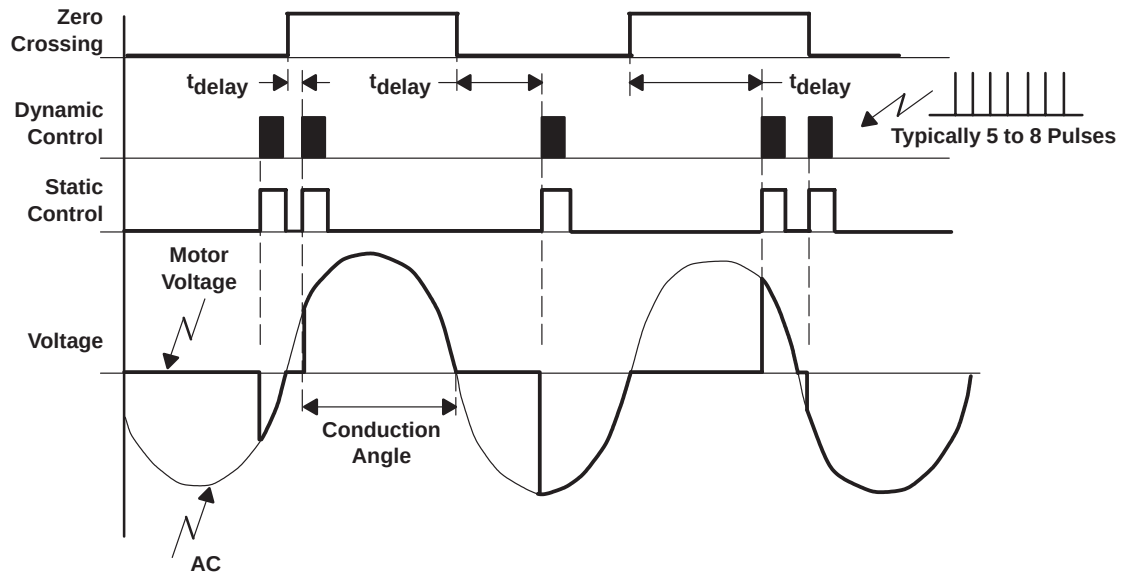
Figure 4–86. Static and Dynamic TRIAC Gate Control
