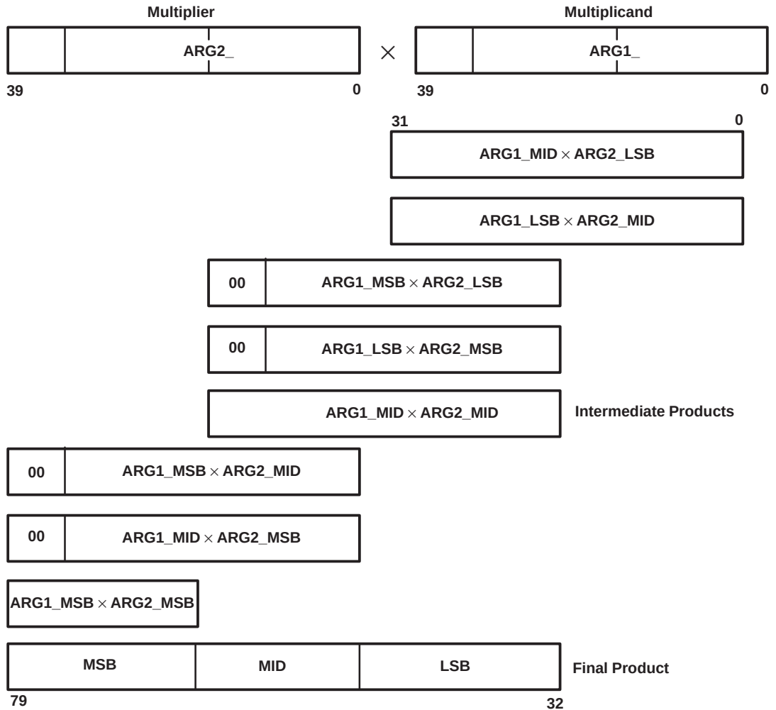
Figure 6–57. 40 × 40-Bit Unsigned Multiplication MPYU40
