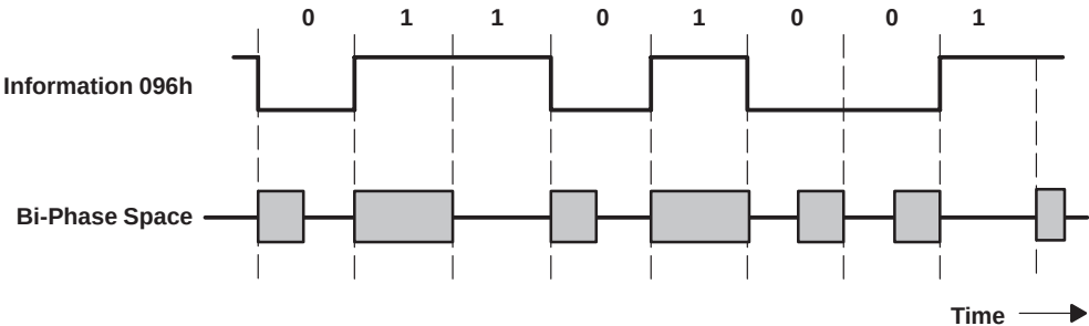
Figure 6–35. Biphas Space Modulation
