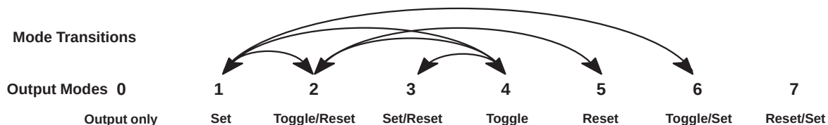
Figure 6–15. Unsafe Output Mode Changes
