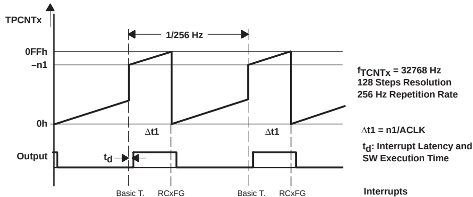
Figure 3–16. PWM Timing by Universal Timer/Port Module and Basic Timer
