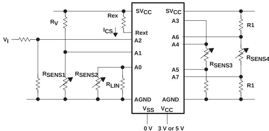
Figure 4–38. Resistive Sensors Connected to MSP430C32x
