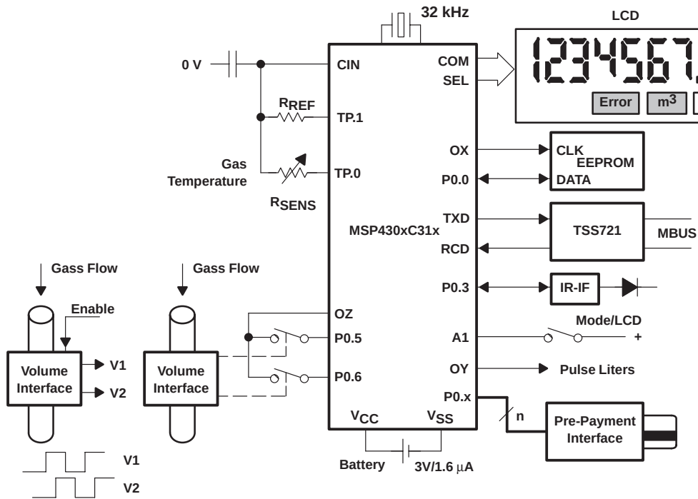
Figure 4–29. Gas Meter With MSP430C31x
