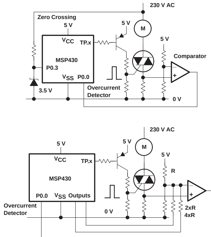
Figure 4–89. Overcurrent Detection With Single and Multiple Thresholds
