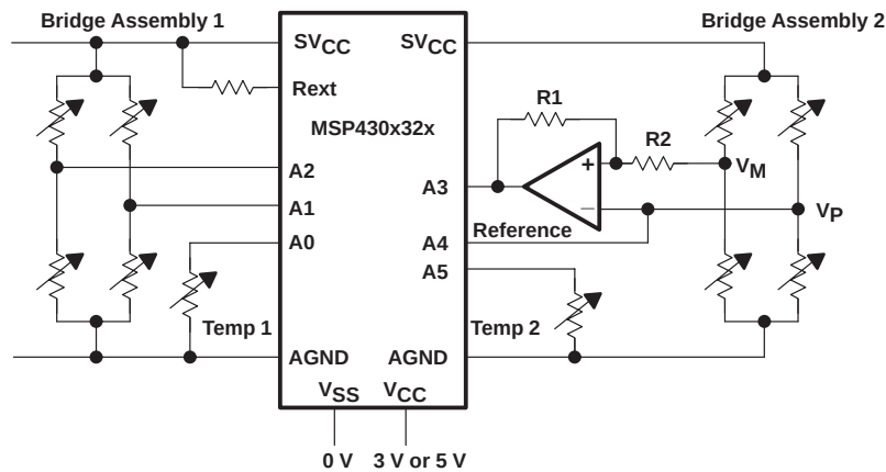
Figure 4–40. Connection of Bridge Assemblies
