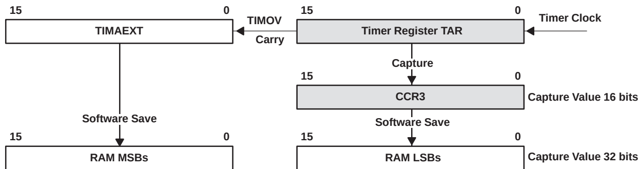
Figure 6–28. Capture Mode With Timer Values Greater than 16 Bit (shown for CCR3)
