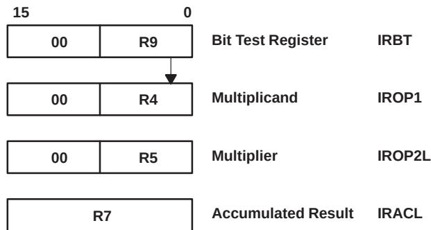
Figure 5–2. 8 x 8 Bit Multiplication – Register use
