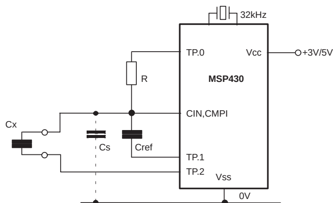
Figure 19. Measurement of a Capacitor C_x
