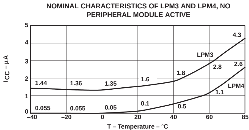
Figure 4–57. Approximated Characteristics for the Low Power-Supply Currents
