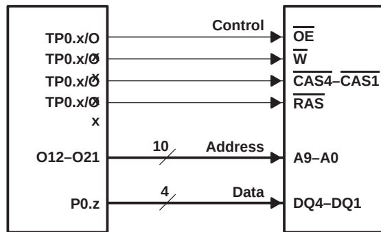
Figure 3–20. External Memory Control With MSP430 Ports
