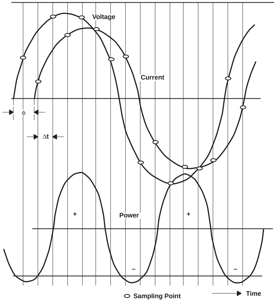
Figure 4–3. Reduced Scan Measurement Principle
