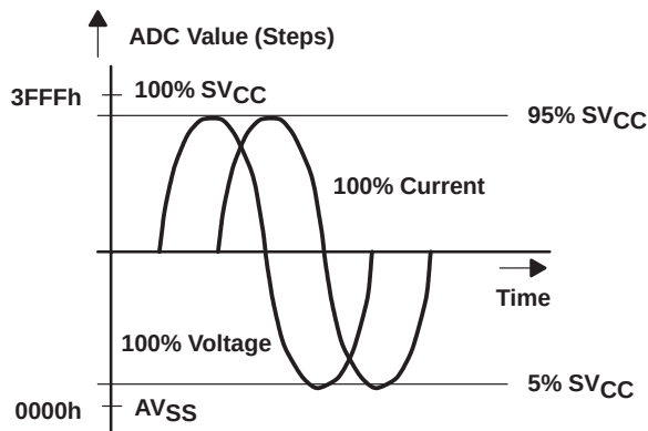
Figure 4–4. Allocation of the ADC Range
