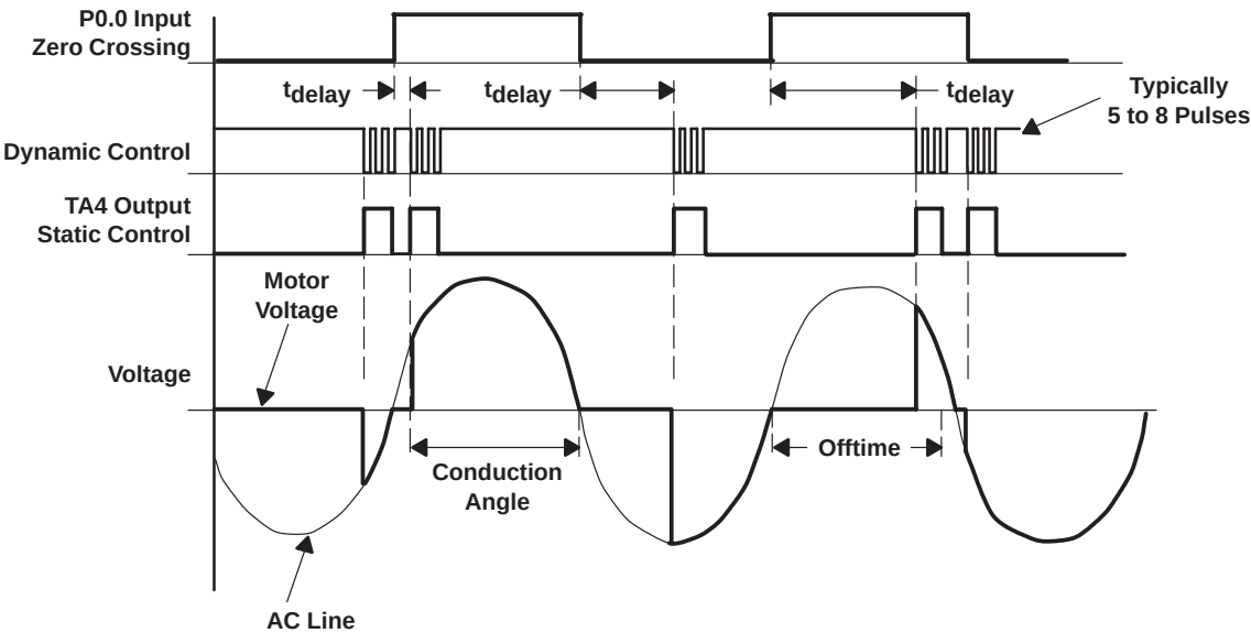
Figure 6–25. Static and Dynamic TRIAC Gate Control
