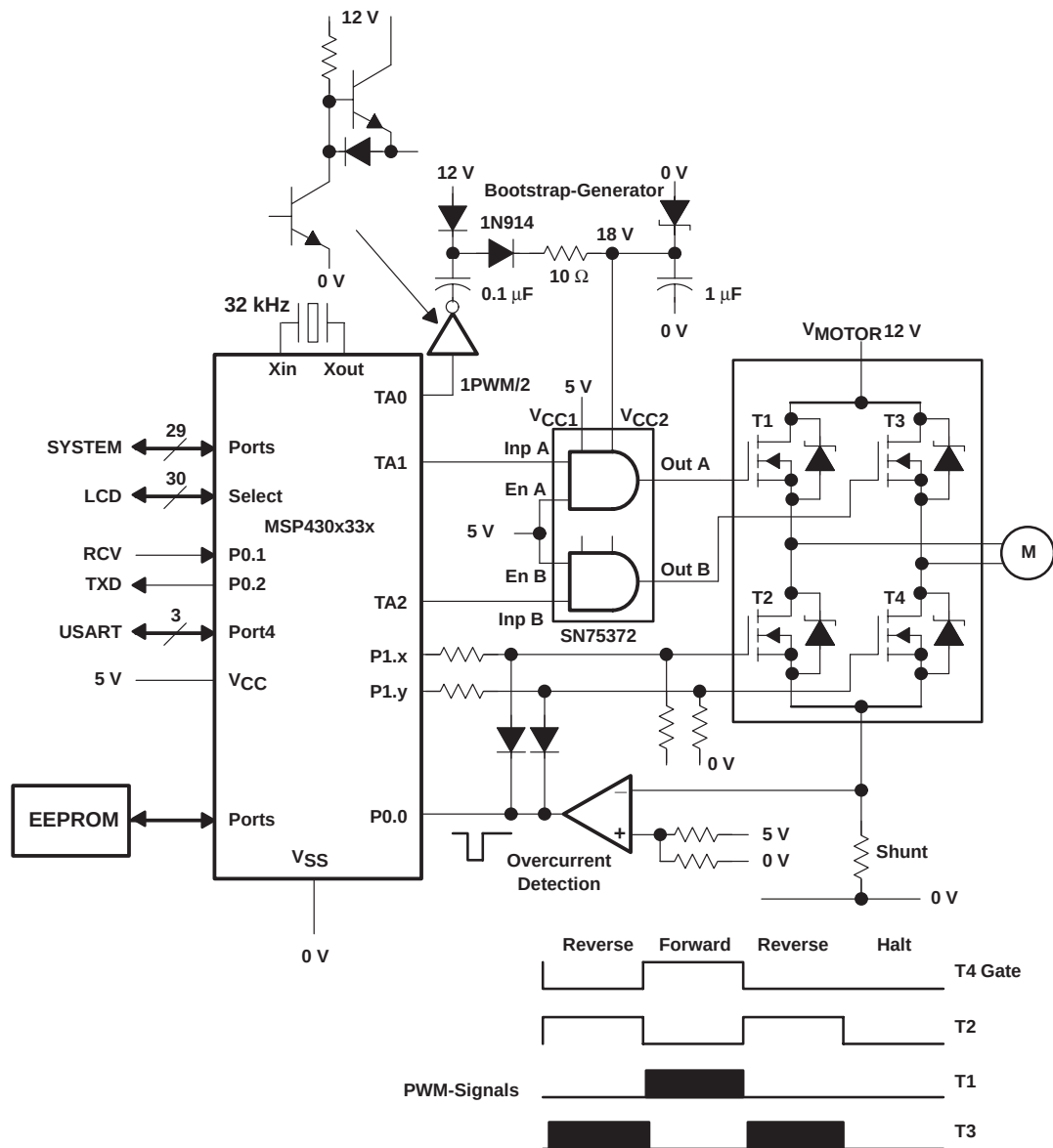
Figure 4–76. PWM Motor Control With a MOSFET H-Bridge
