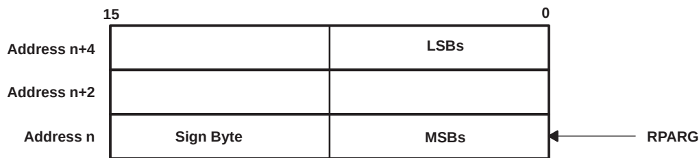
Figure 5–25. Binary Number Format 48 Bit
