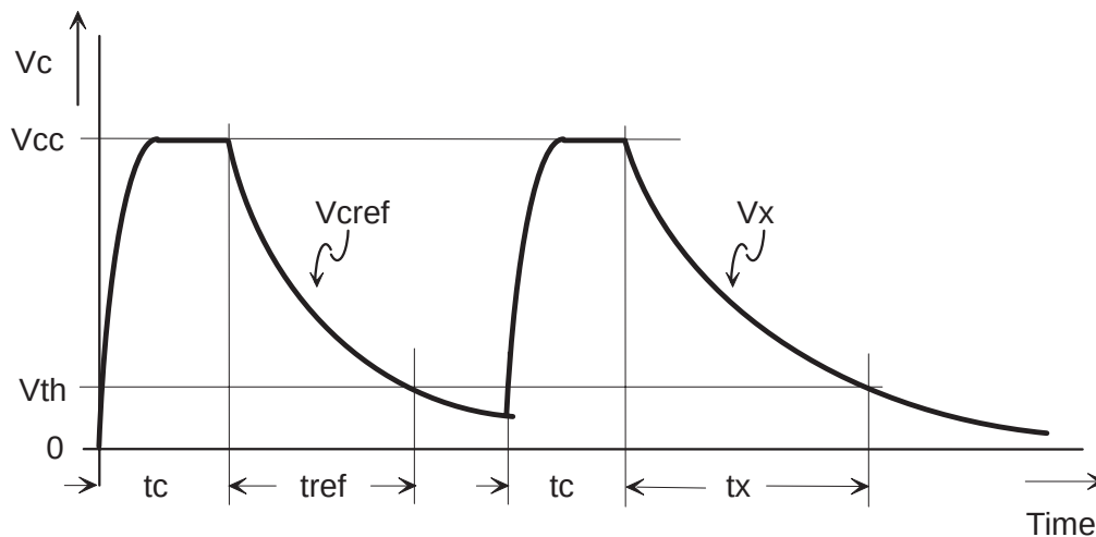
Figure 20. Timing for the Capacity Measurement
