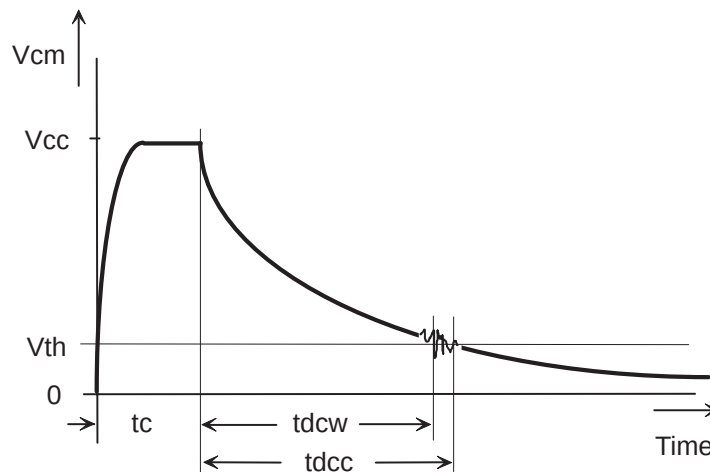
Figure 5. Noise Influence During Measurement
