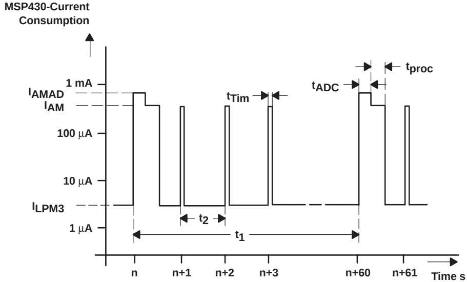
Figure 4–58. Current Consumption Characteristic
