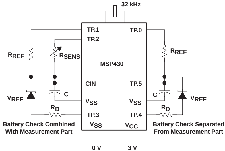
Figure 5–34. Battery Check With the Universal Timer/Port Module
