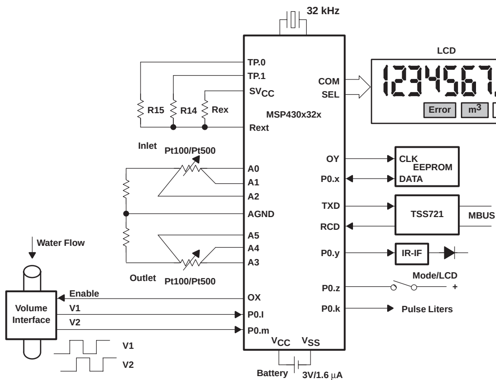
Figure 4–36. Heat Volume Counter With 16 Bits Resolution MSP430C32x
