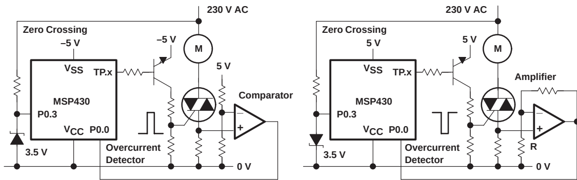
Figure 4–85. Positive and Negative TRIAC Gate Control
