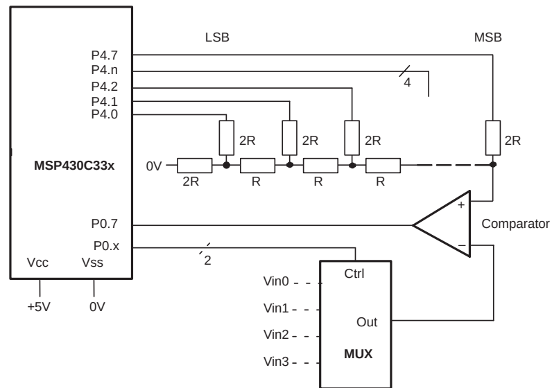
Figure 22. R/2R Method for Analog-to-Digital Conversion
