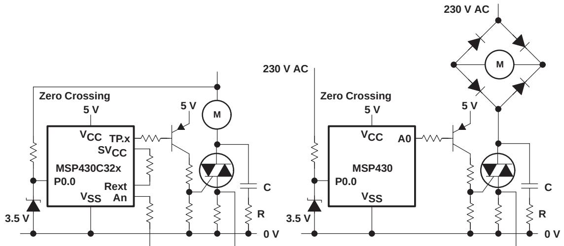
Figure 4–84. TRIAC Control for AC Motors and DC Motors
