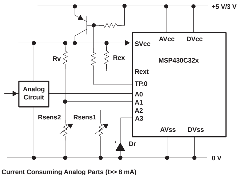
Figure 34. Connection of Current Consuming Loads to SVcc
