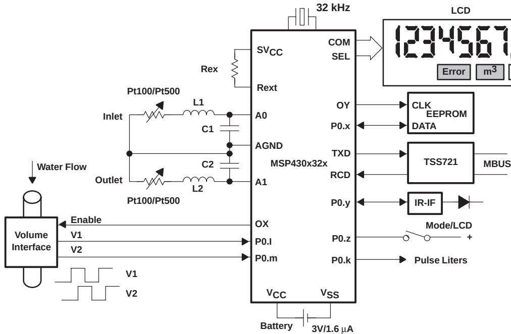
Figure 4–34. Heat Volume Counter MSP430C32x
