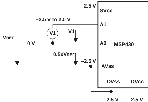
Figure 9. Split Power Supply for Signed Voltage Measurement
