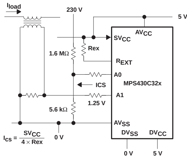
Figure 4–11. Resistor Interface With Current Source
