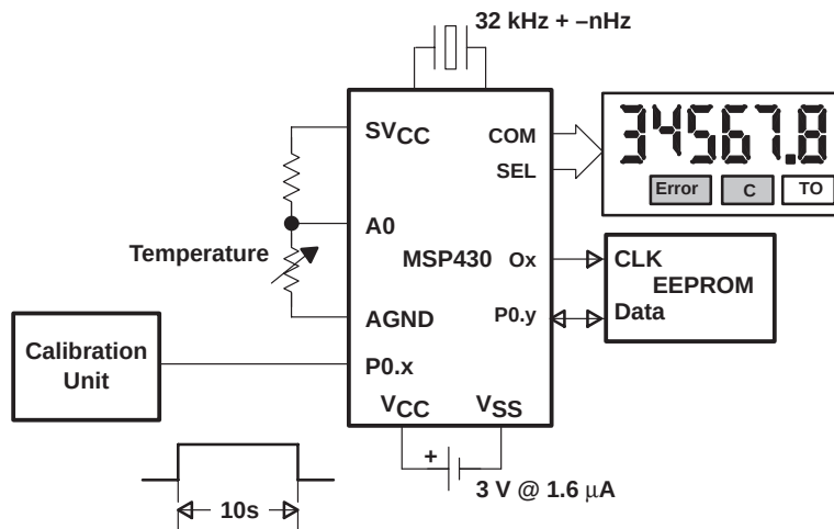
Figure 6–1. Crystal Calibration
