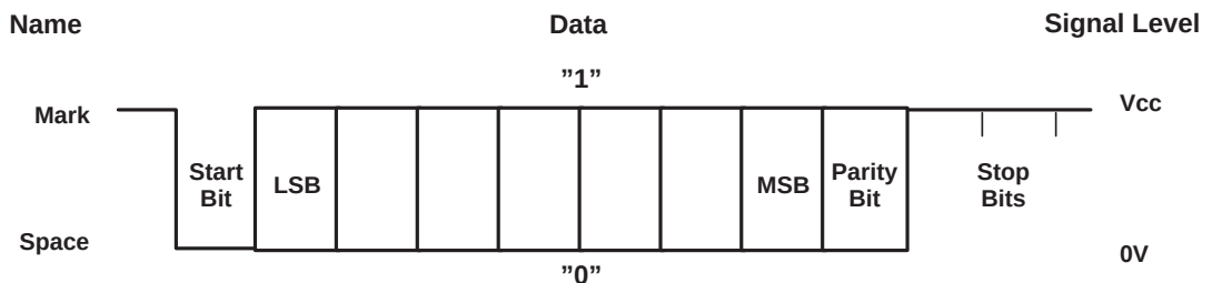
Figure 6–87. RS232 Format (Levels at the MSP430)
