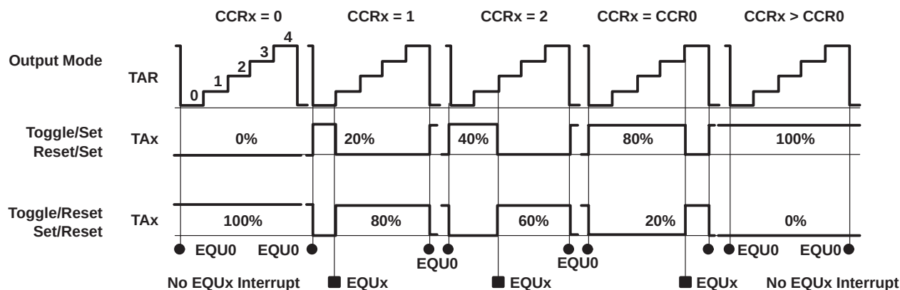
Figure 6–20. PWM Signals at TAx in the Up Mode (CCR0 contains 4)
