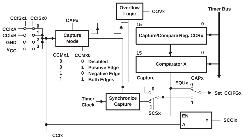
Figure 6–10. Function of the Capture/Compare Registers (CCRx)
