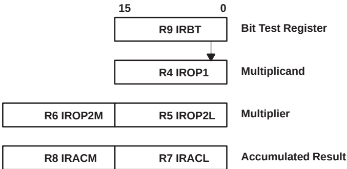
Figure 5–1. 16 x 16 Bit Multiplication – Register Use
