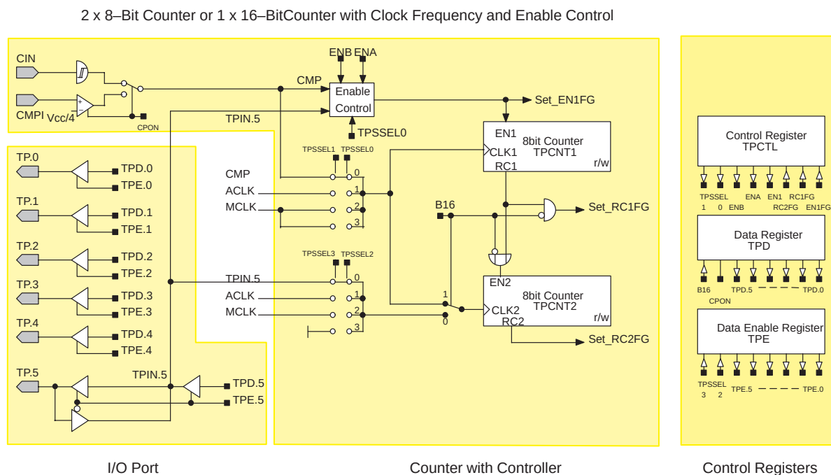
Figure 1. Block Diagram of the Universal Timer/Port Module
