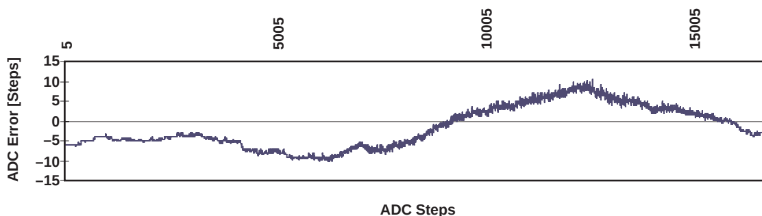
Figure 36. Error Characteristic Device 2
