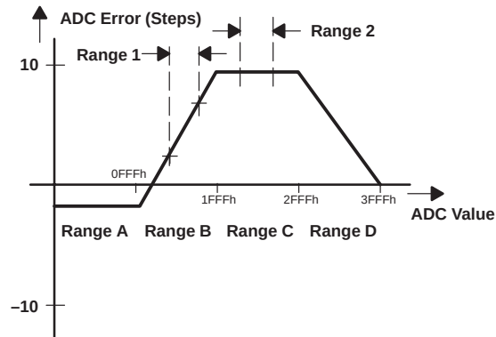
Figure 4–41. Simplified ADC Characteristic
