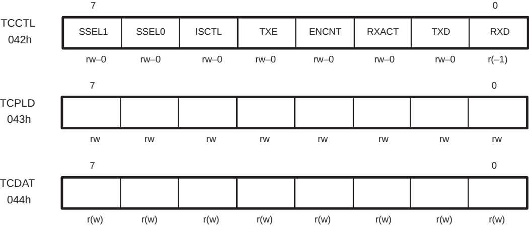
Figure 6–89. UART Hardware Registers
