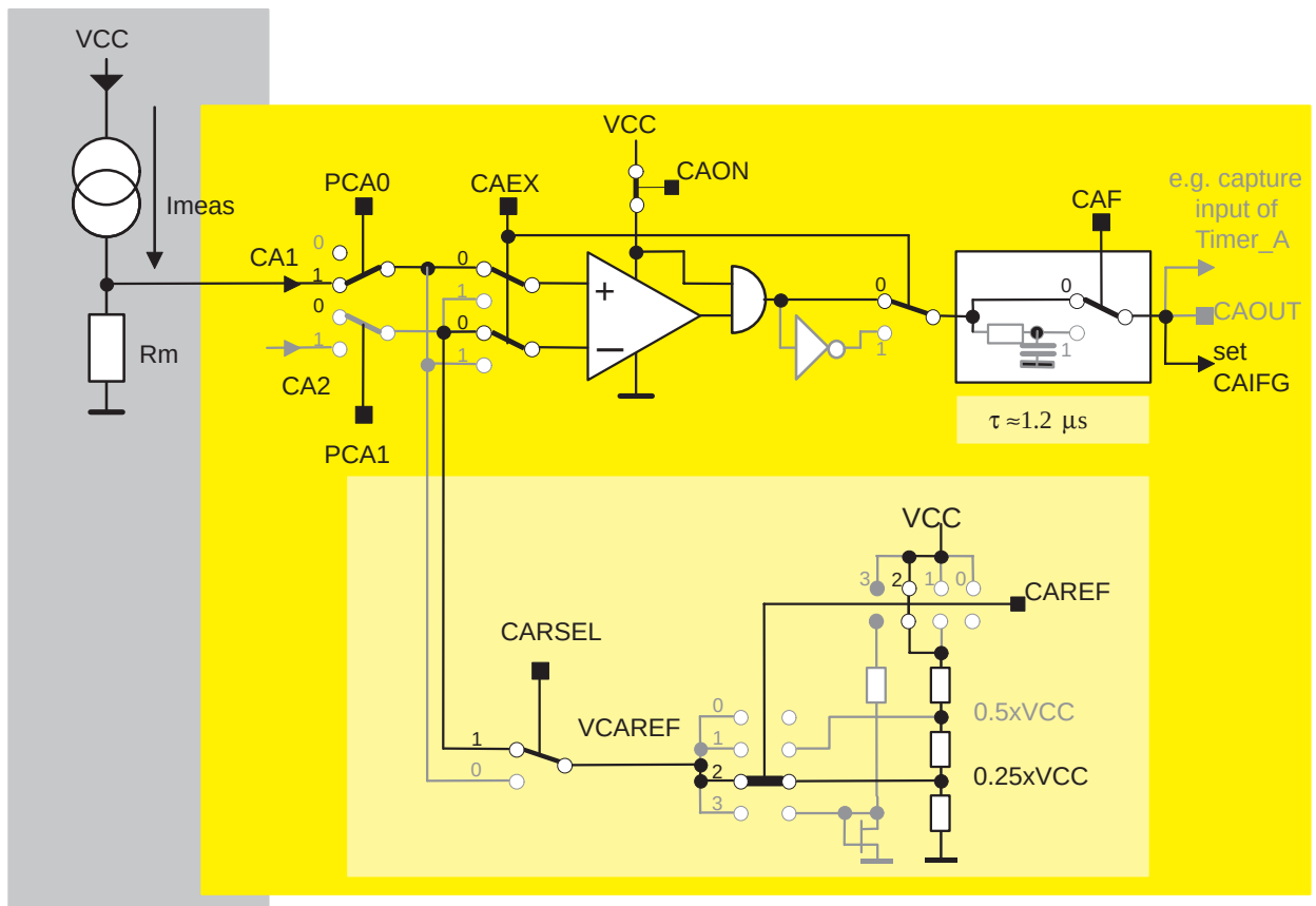
Figure 6–98. Fast Comparator Input Check Circuitry
