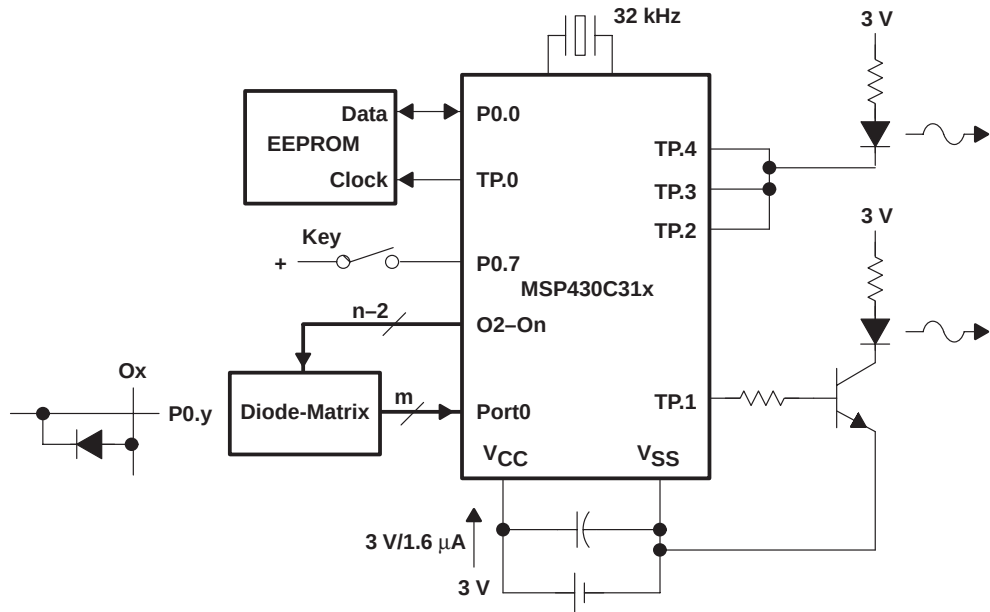
Figure 4–64. Remote Control Transmitter for Security Applications
