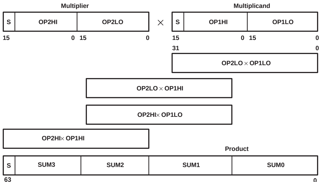
Figure 6–58. 32 × 32-Bit Signed Multiplication MPYS32
