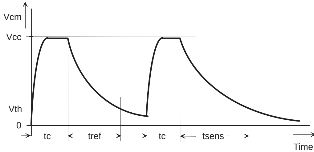
Figure 3. Timing for the Universal Timer/Port Module ADC
