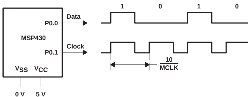
Figure 3–5. Connections for Fast Serial Transfer
