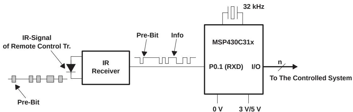
Figure 4–66. Remote Control Receiver With the MSP430
