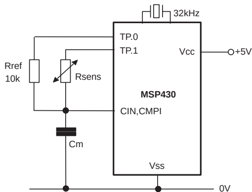
Figure 2. Minimum Sensor Circuit
