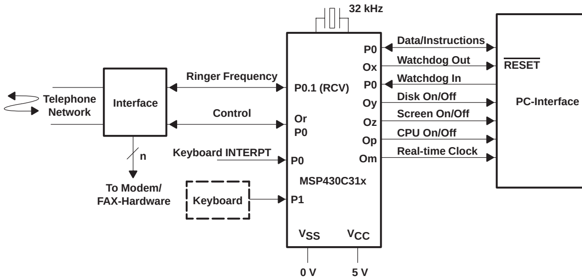
Figure 4–68. MSP430 in an AC-Powered Personal Computer
