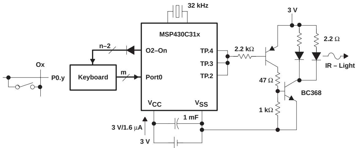
Figure 4–65. Remote Control Transmitter for Audio/Video
