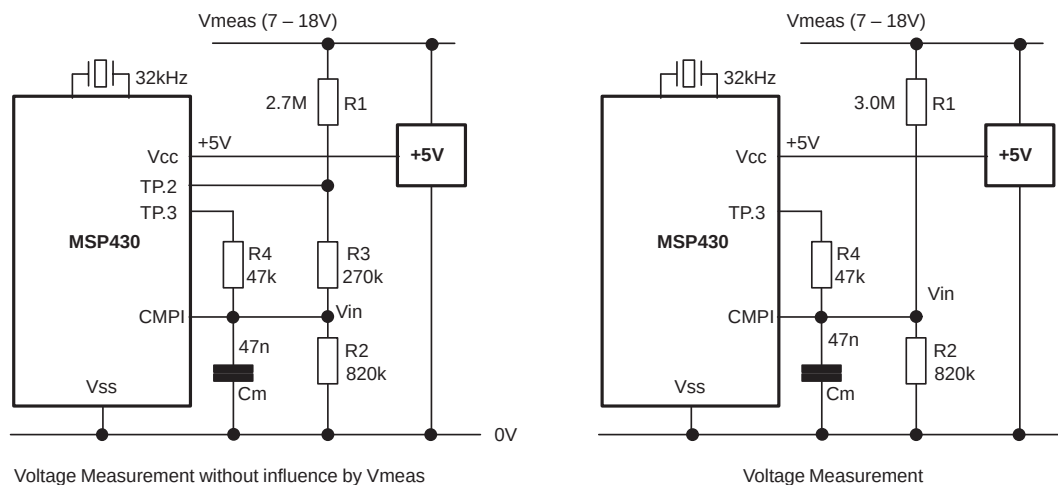
Figure 12. Voltage Measurement of a Voltage Source
