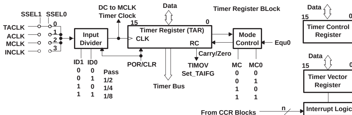
Figure 6–4. The Timer Register Block
