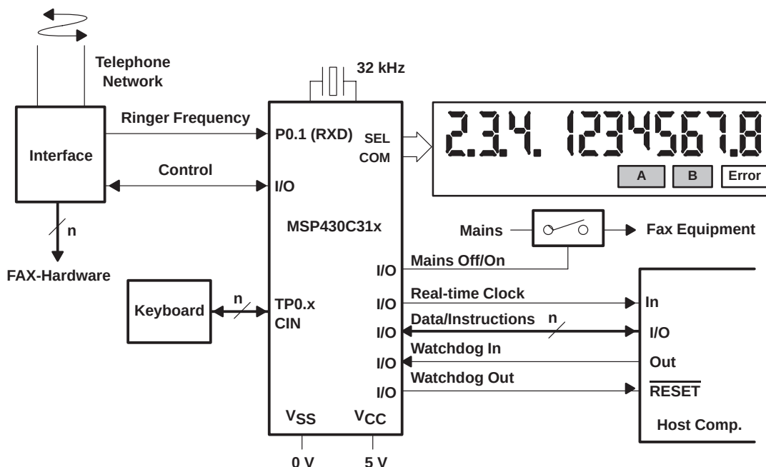
Figure 4–70. MSP430-Controlled FAX Device
