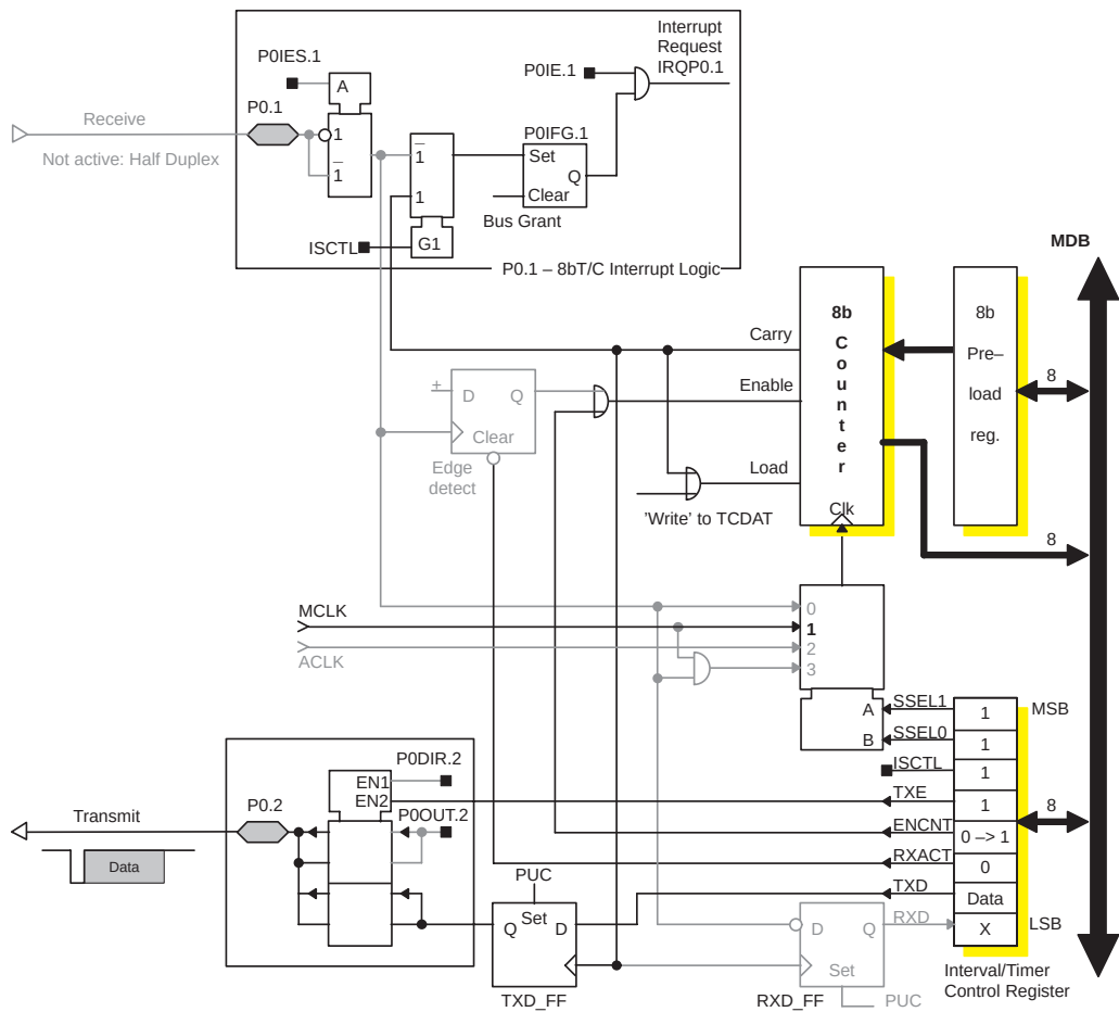
Figure 6–90. The 8-Bit Timer/Counter Transmit Mode
