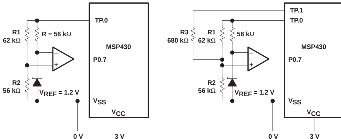
Figure 5–32. Battery Check With an External Comparator
