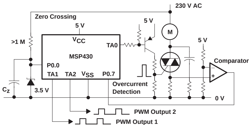
Figure 6–39. TRIAC Control with Timer A
