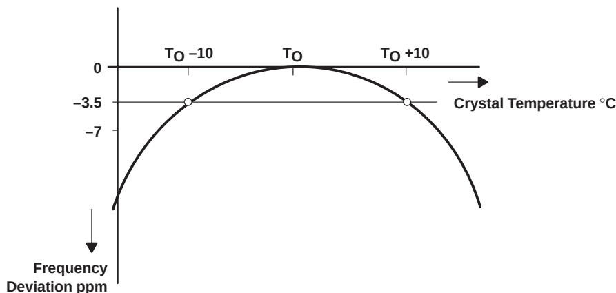
Figure 6–2. Crystal Frequency Deviation With Temperature
