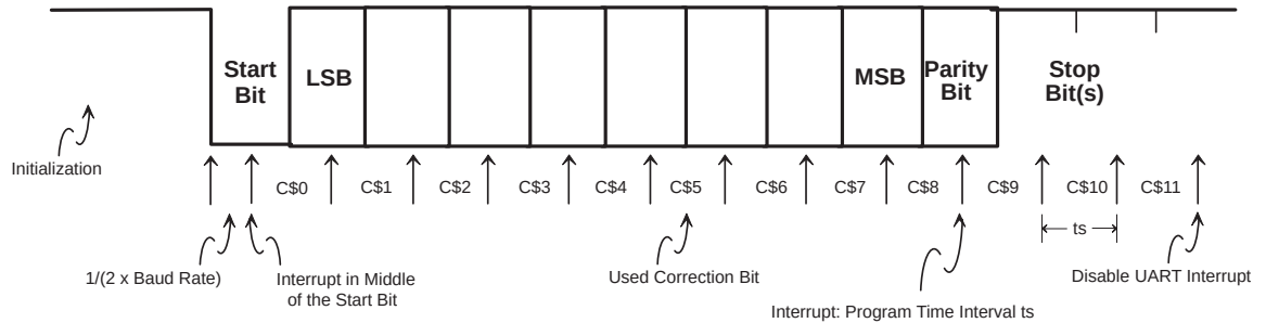
Figure 6–93. Interrupt Timing for the Receive Mode
