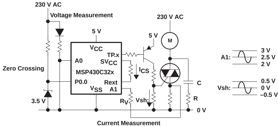
Figure 4–90. Motor Voltage Measurement and Current Measurement
