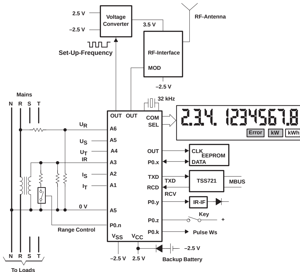
Figure 4–48. MSP430C32x EE Meter With RF Readout
