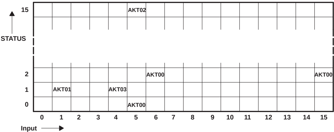
Figure 5–18. Matrix for Few Valid Combinations
