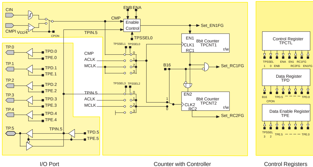
Figure 6–74. Block Diagram of the Universal Timer/Port Module
