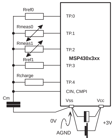
Figure 6. Hardware Schematic for Interrupt Example
