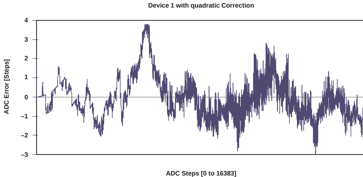
Figure 3. Error Correction With Four Quadratic Equations
