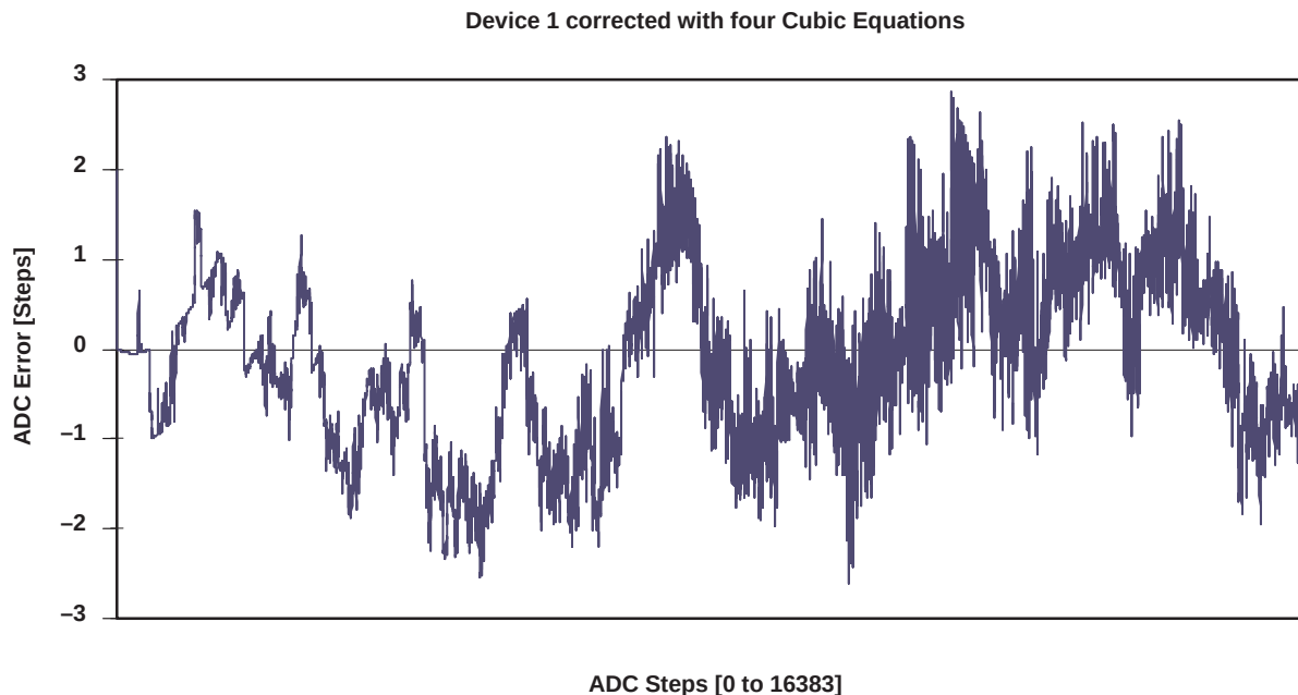
Figure 5. Error Correction With Four Cubic Equations
