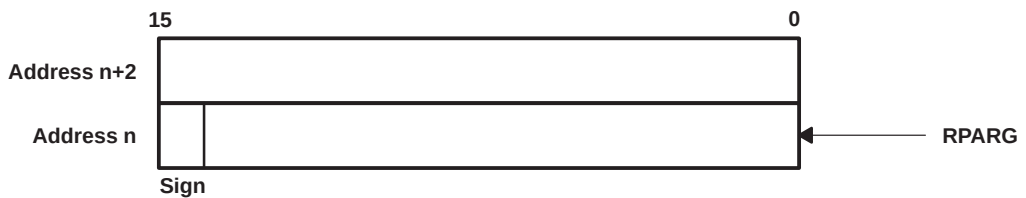
Figure 5–23. Signed Binary Input Buffer Format 32 Bits
