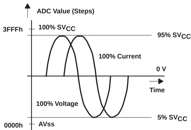
Figure 4–26. Allocation of the ADC Range
