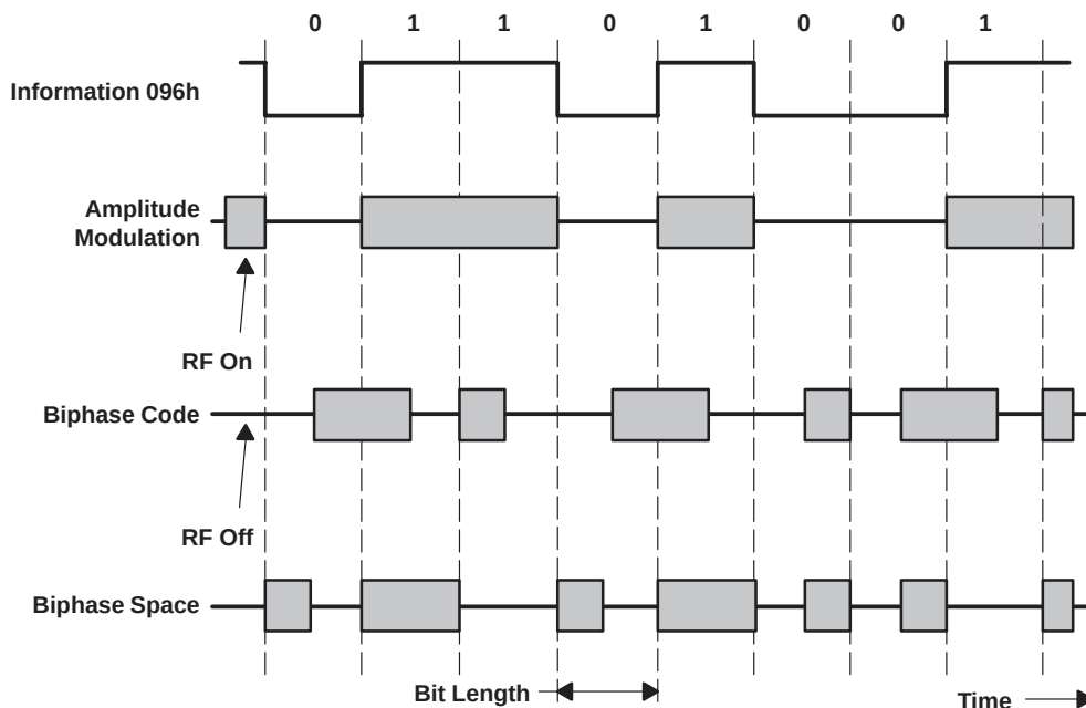
Figure 6–41. RF Modulation Modes
