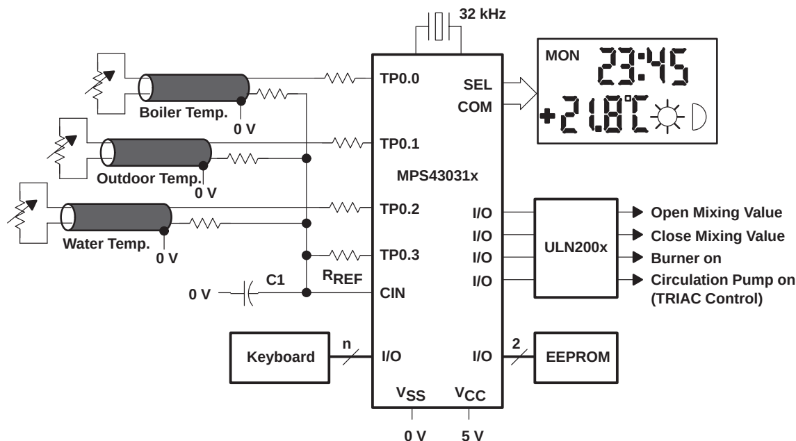
Figure 4–61. Intelligent Heating Installation Control With the MSP430
