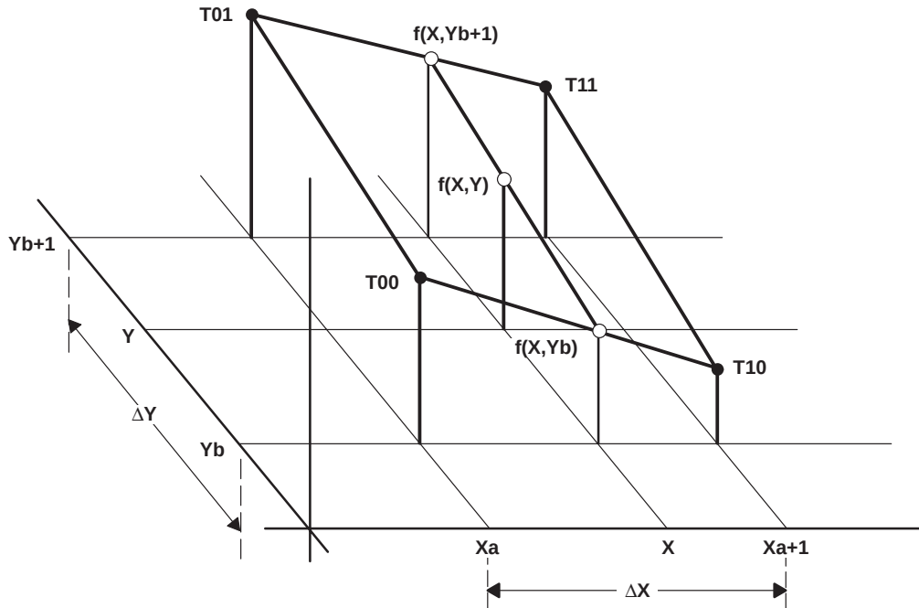
Figure 5-7. Algorithm for Two-Dimensional Tables
