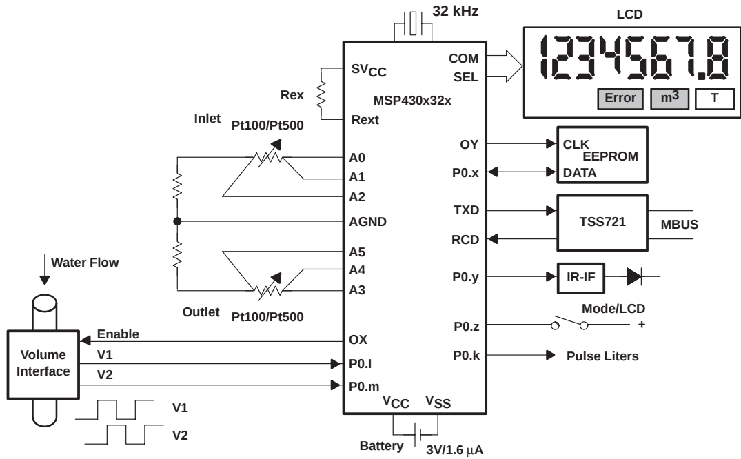
Figure 4–35. Heat Volume Counter With 4-Wire-Circuitry MSP430C32x
