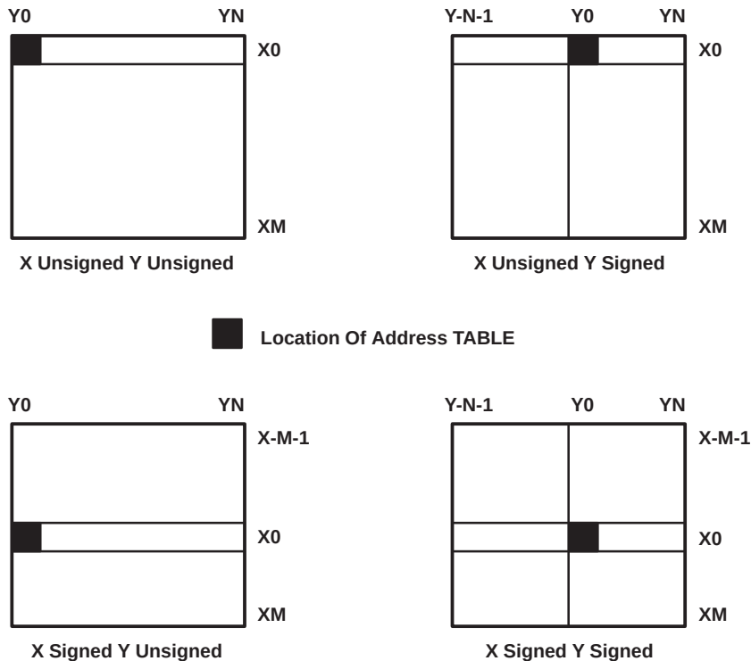
Figure 5–8. Table Configuration for Signed X and Y
