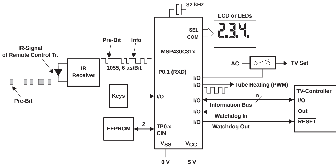
Figure 4–67. MSP430 in a TV Set
