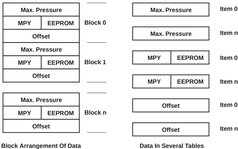
Figure 5–5. Data Arrangement in Tables
