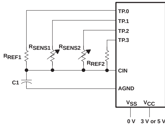
Figure 4–39. Measurement With Reference Resistors
