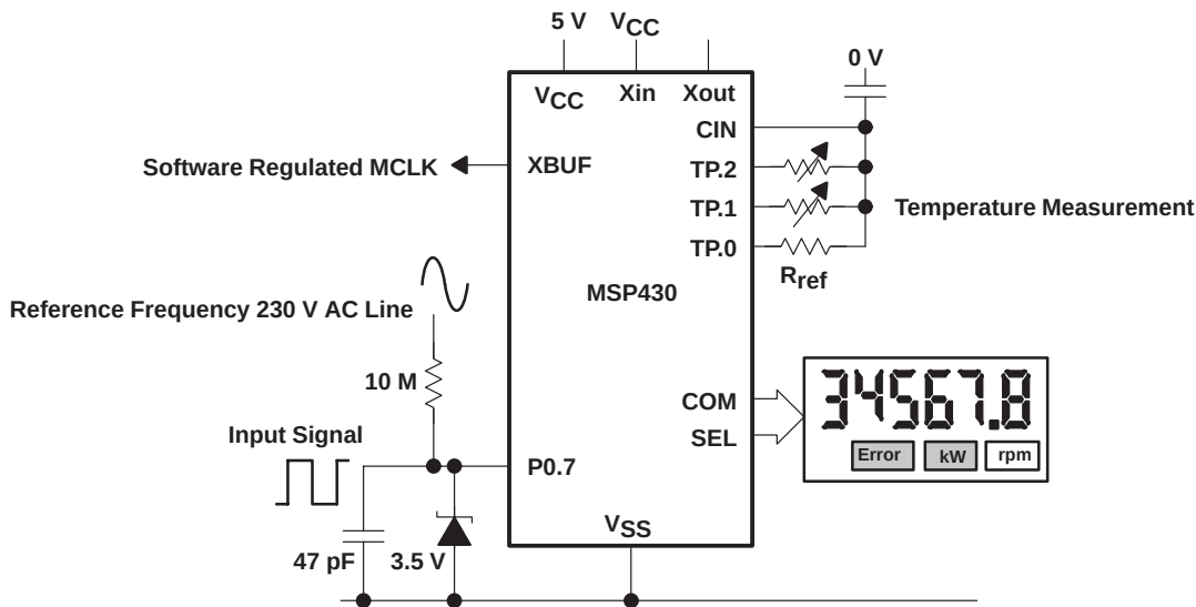
Figure 6–30. MSP430 Operation Without Crystal
