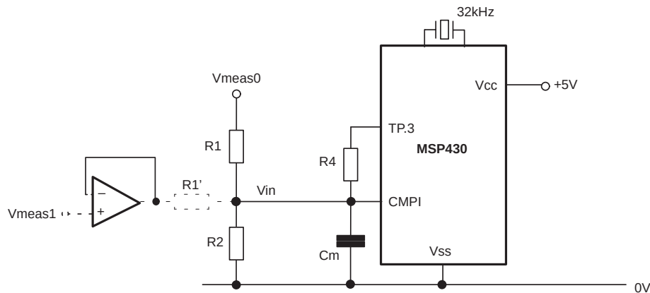
Figure 10. Voltage Measurement With the Universal Timer/Port Module
