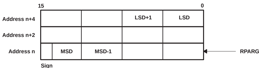
Figure 5–27. BCD Buffer Format
