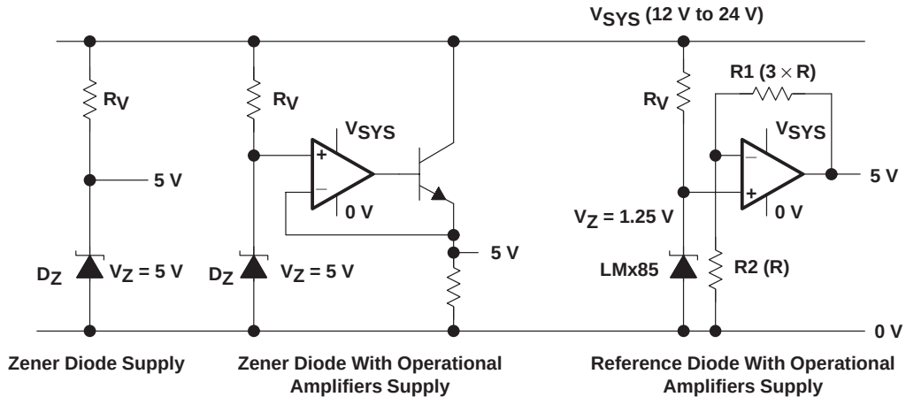
Figure 3–39. Simple Power Supply From Other DC Voltages
