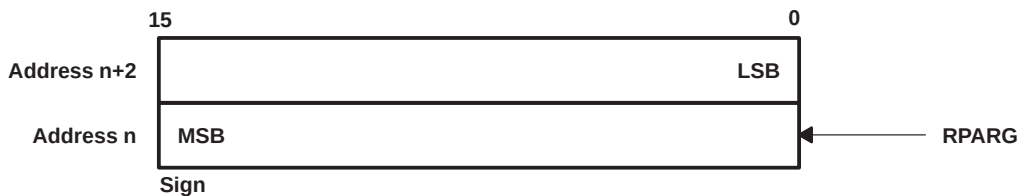
Figure 5–24. Unsigned Binary Input Buffer Format 32 Bits
