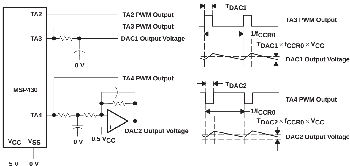
Figure 6–38. Digital-to-Analog Conversion
