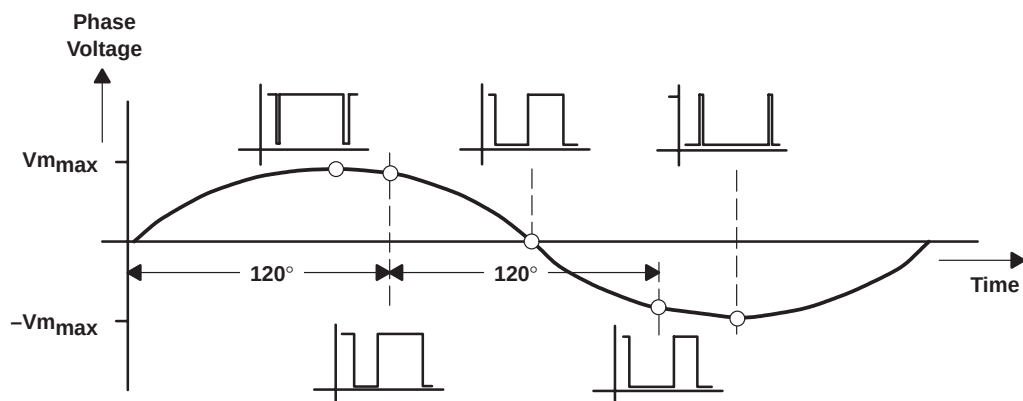
Figure 4–81. PWM Outputs for Different Phase Voltages
