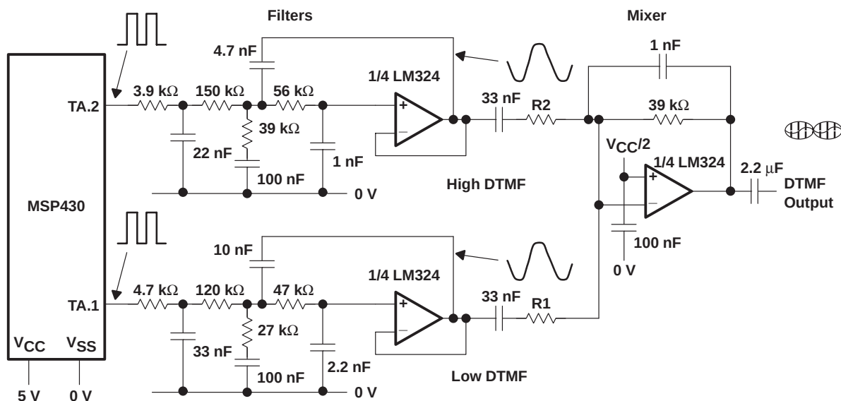
Figure 6–23. DTMF Filters and Mixer
