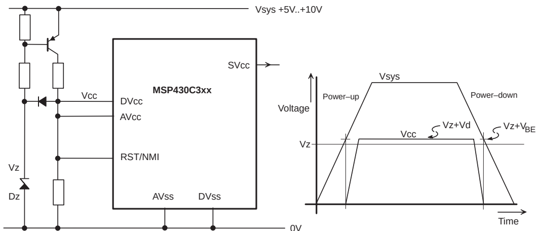
Figure 6–67. Simple RESET Circuit With a PNP Transistor
