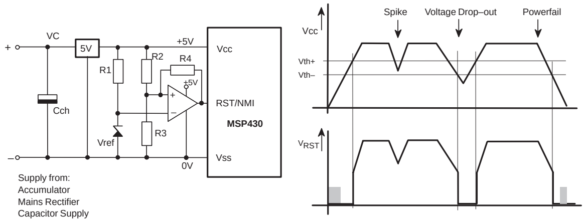
Figure 6–69. RESET Circuit With a Schmitt Trigger and a Reference Diode
