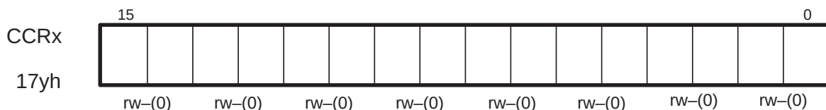
Figure 6–9. The Capture/Compare Registers CCRx
