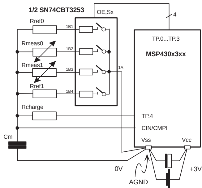
Figure 18. Solution With a Low-Resistive Multiplexer
