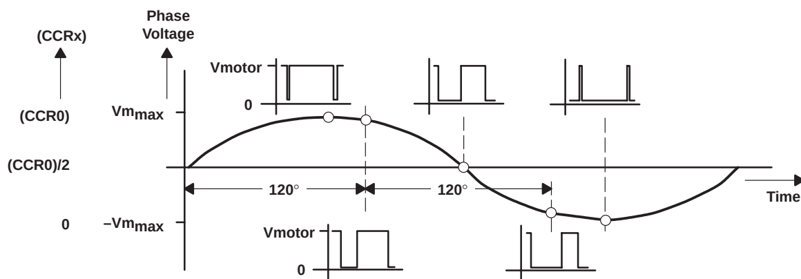
Figure 6–46. PWM Outputs for Different Phase Voltages
