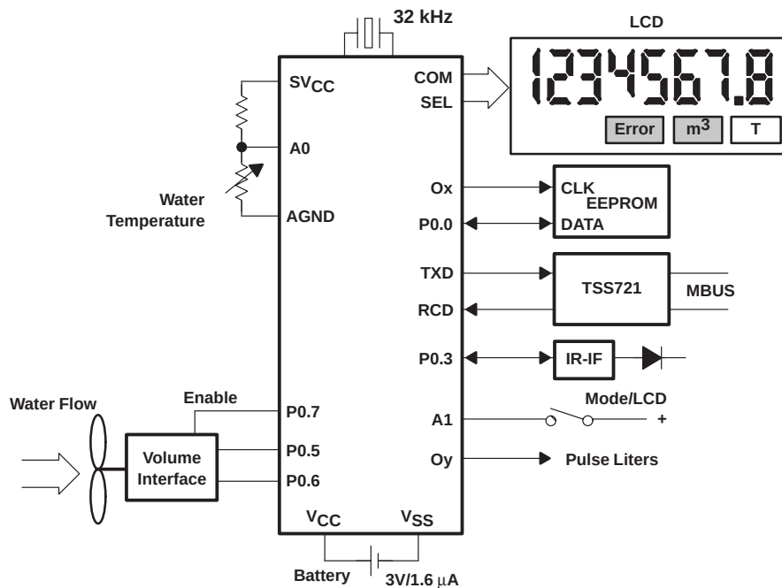
Figure 4–31. Electronic Water Flow Meter
