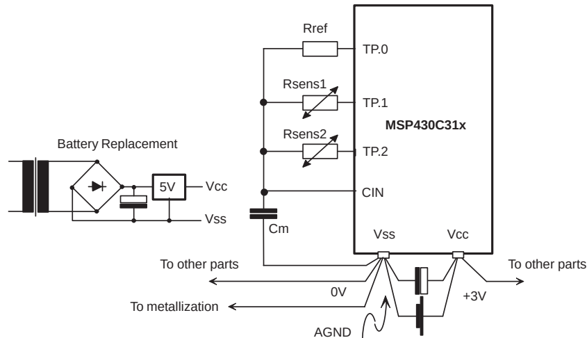
Figure 9. Grounding for the Universal Timer/Port ADC
