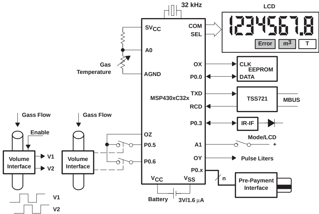
Figure 4–28. Gas Meter With MSP430C32x
