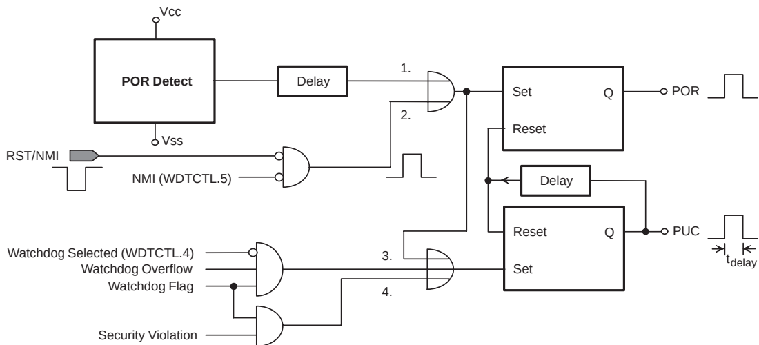
Figure 6–64. Simplified MSP430 RESET Circuitry
