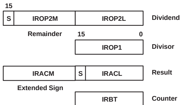
Figure 5–4. Signed Division – Register Use
