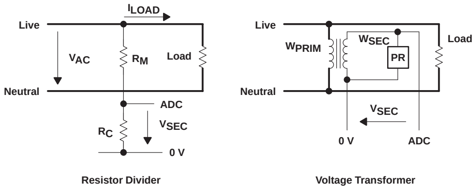
Figure 4–14. Voltage Measurement
