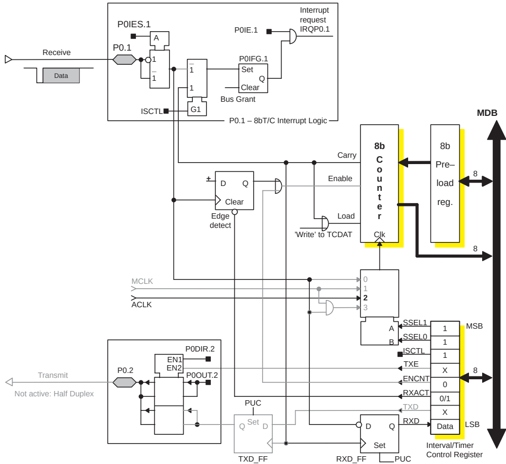
Figure 6–92. The 8–Bit Timer/Counter in Receive Mode
