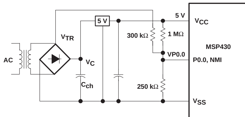
Figure 5–38. Power-Fail Detection With the Watchdog
