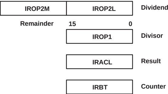
Figure 5–3. Unsigned Division – Register Use
