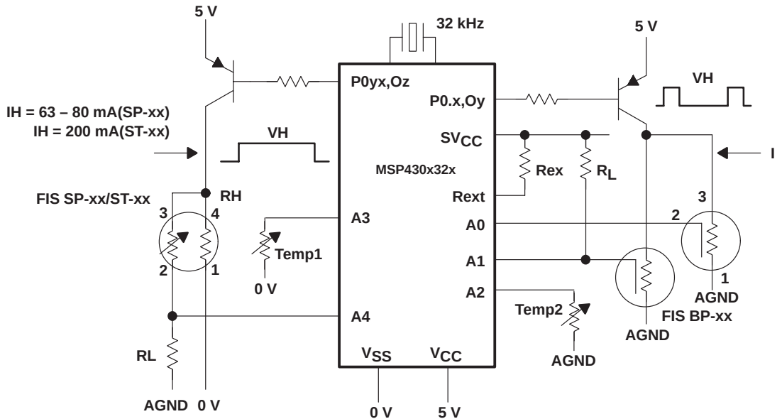
Figure 4–43. Gas Sensor Connection to the MSP430C32x
