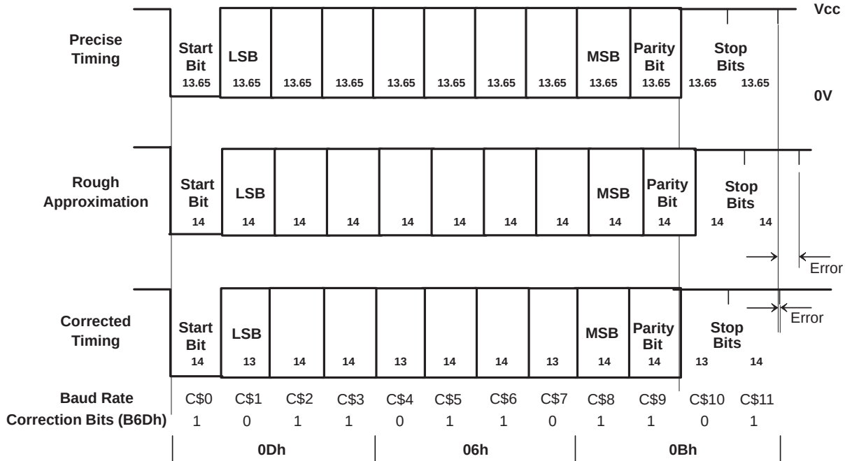
Figure 6–94. Baud Rate Correction
