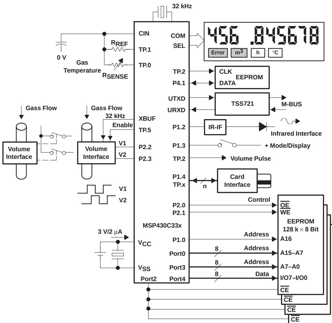
Figure 4–30. MSP430C336 Gas Meter
