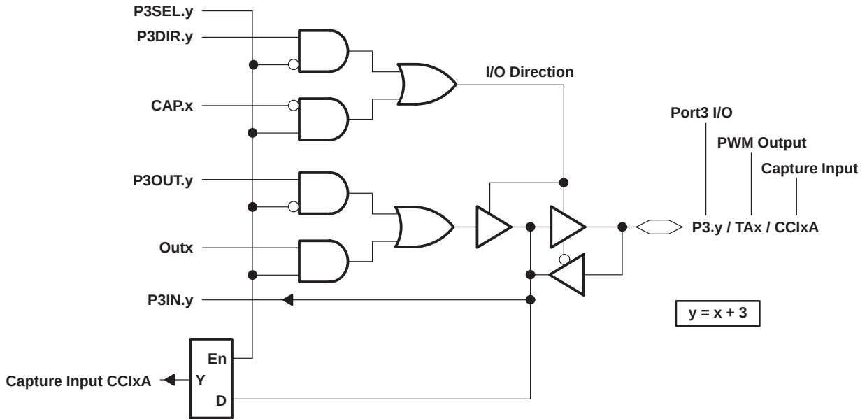
Figure 6–17. Connection of the Port3 Terminals to the Timer_A (MSP430C33x Configuration)
