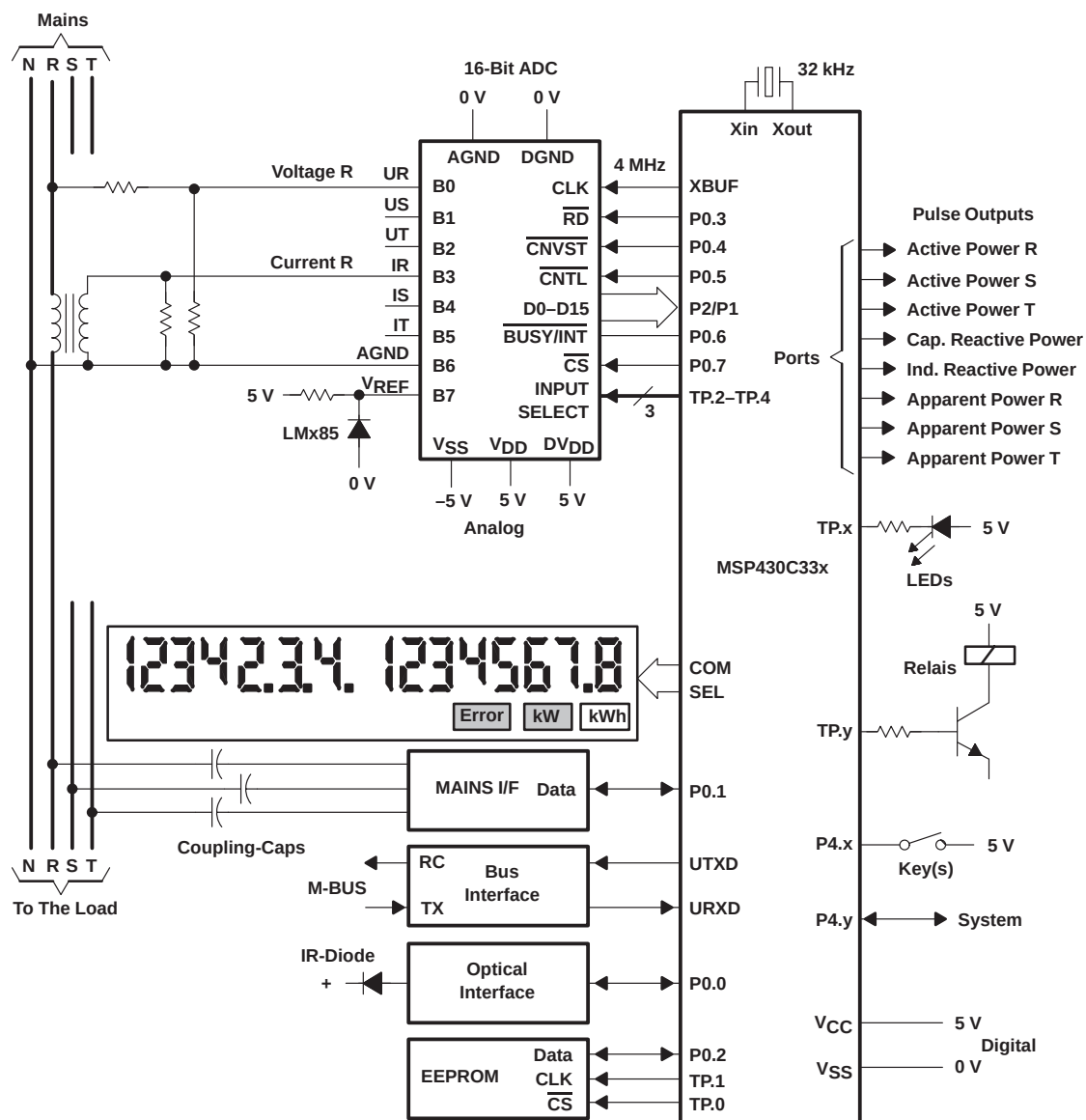
Figure 4–25. Electricity Meter With an External 16-Bit ADC
