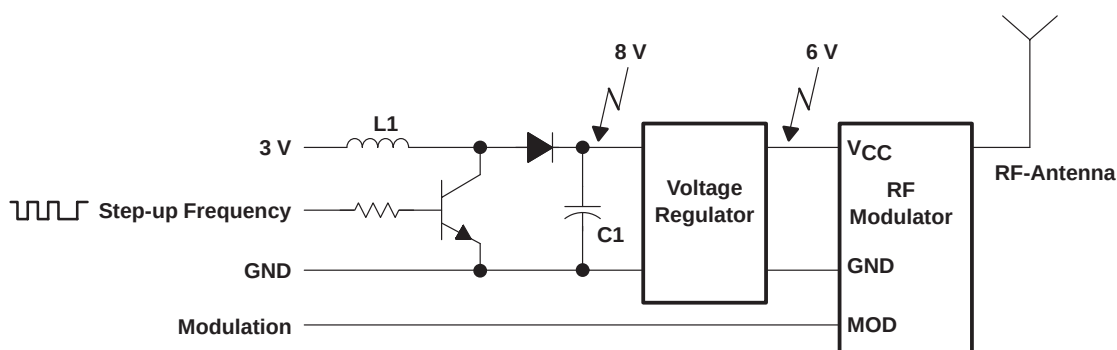
Figure 4–51. RF-Interface Module
