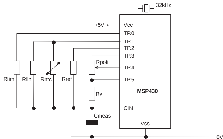
Figure 16. Measurement of a Potentiometer's Position
