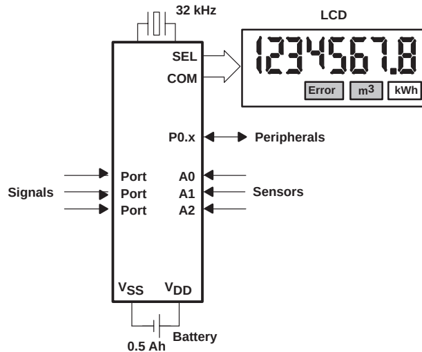
Figure 4–56. Solution With MSP430 for a Battery-Driven System
