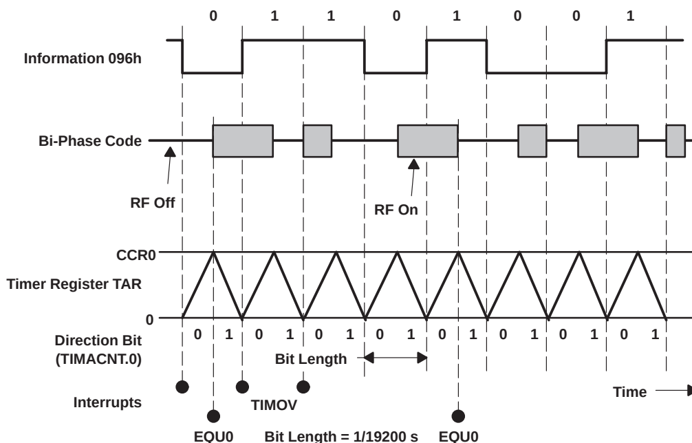
Figure 6–51. Biphase Code Modulation With the Up/Down Mode
