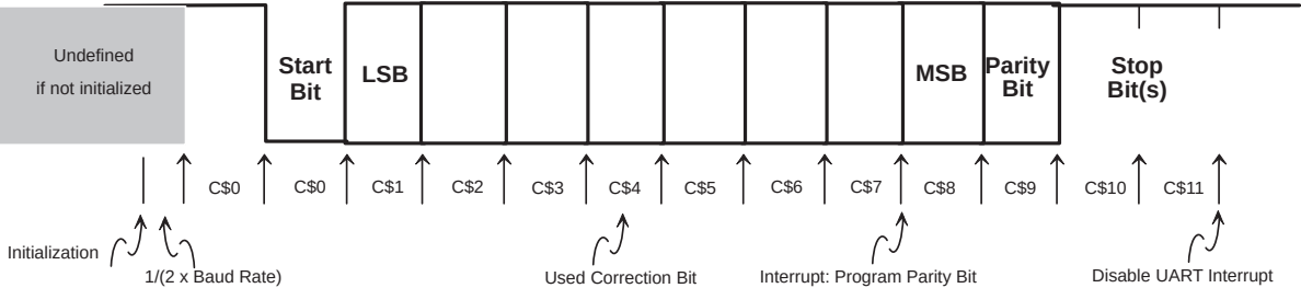
Figure 6–91. Interrupt Timing for the Transmit Mode
