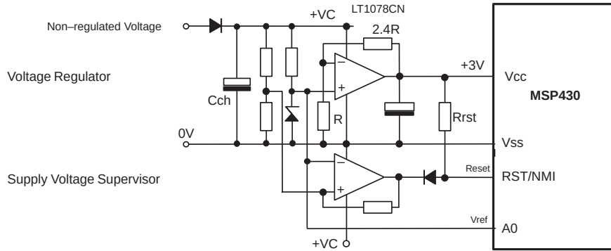
Figure 6–70. RESET Generation With a Comparator
