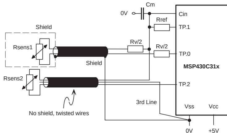
Figure 8. Connection of Long Sensor Lines
