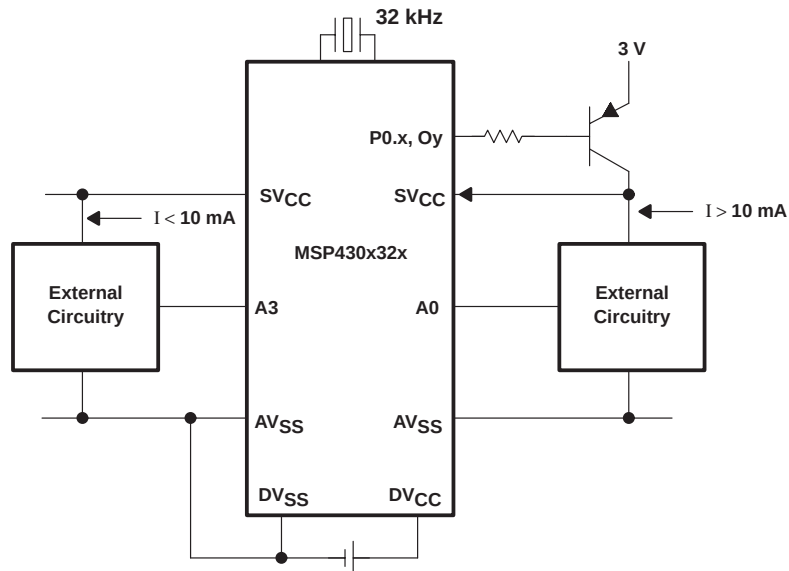
Figure 4–60. Turnoff of External Circuits
