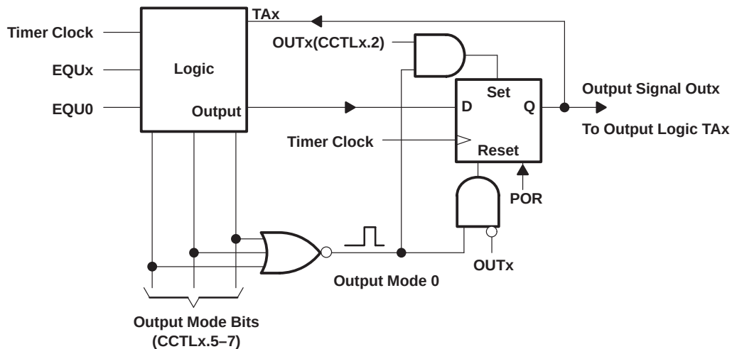
Figure 6–16. Simplified Logic of the Output Units
