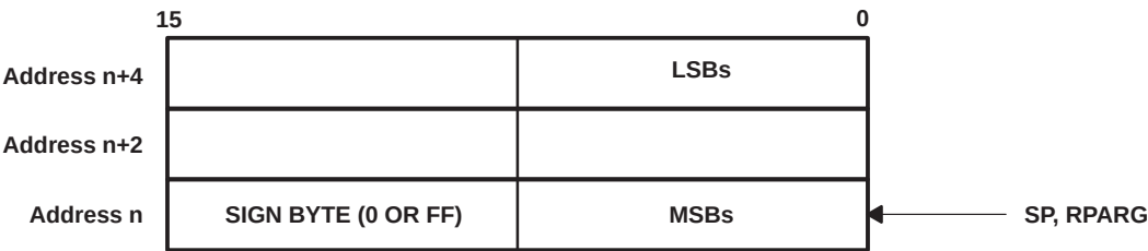
Figure 5–28. Binary Number Format
