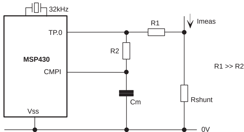
Figure 13. Circuit for the Current Measurement
