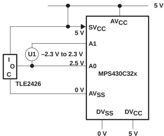
Figure 4–9. Virtual Ground IC for Level Shifting
