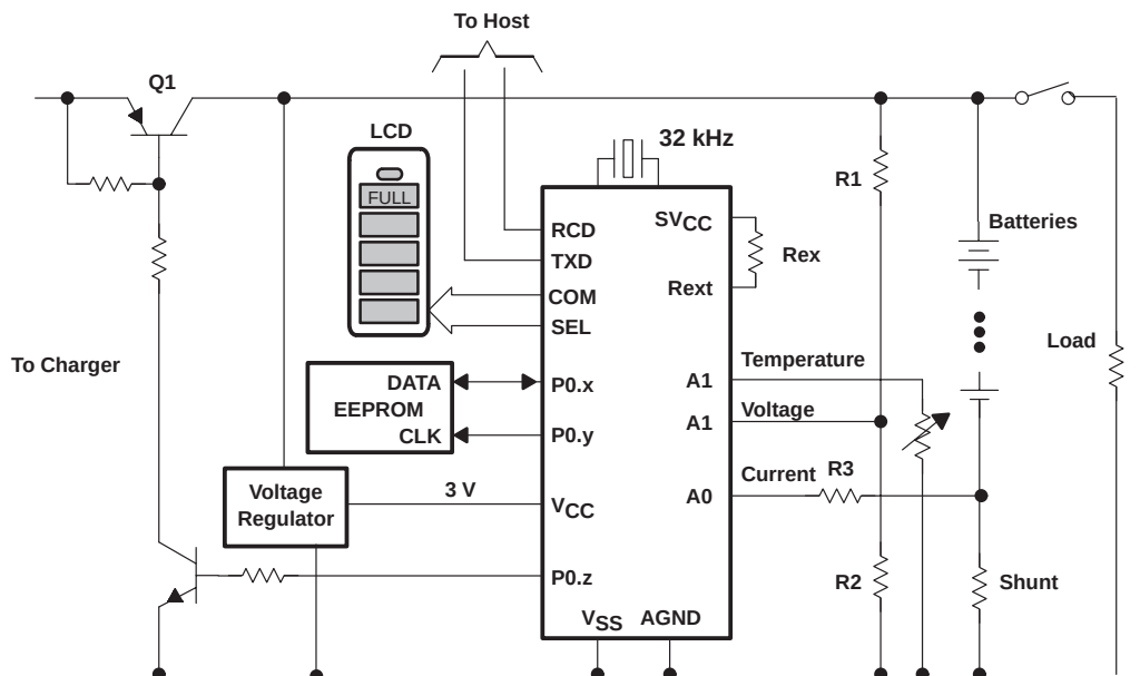
Figure 4–37. Battery Charge Meter MSP430C32x
