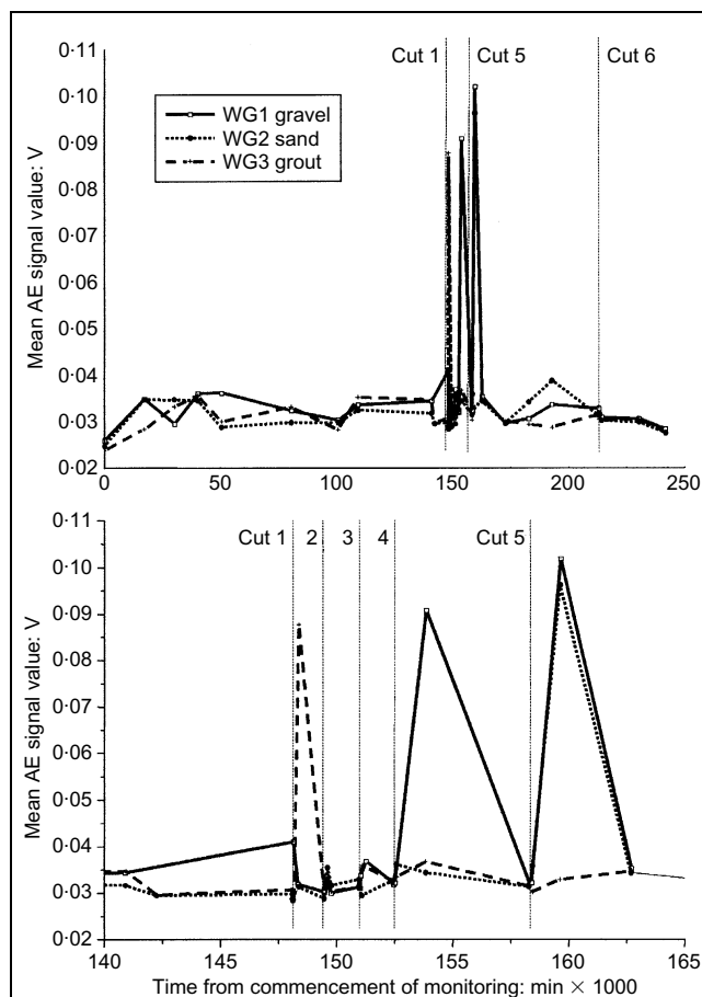
Fig. 15. Arlesey: mean AE signal value for waveguides 1, 2 and 3
