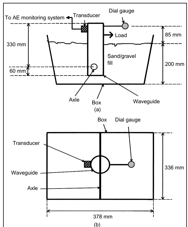
Fig. 5. Waveguide/backfill test apparatus: (a) cross-section; (b) plan
