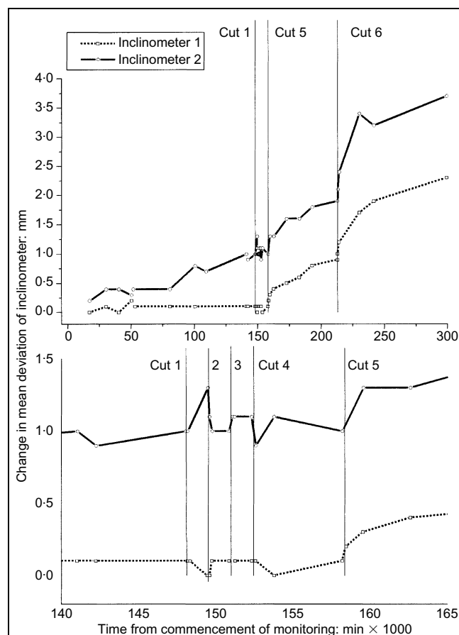
Fig. 14. Arlesey: change in mean deviation for inclinometers 1 (1.5 mbgl) and 2 (0.0 mbgl)
