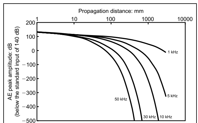
Fig. 3. Relationship between AE attenuation in sand and frequency 9
