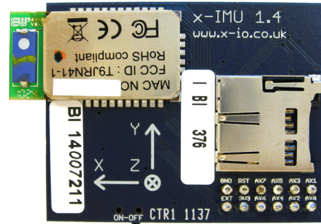
Figure 3: x-IMU bottom
