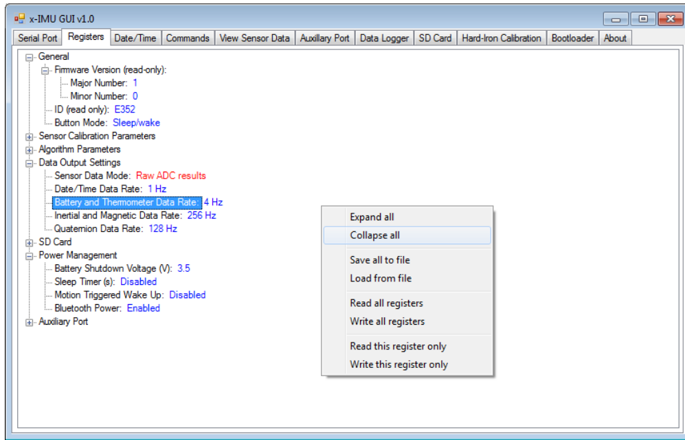
Figure 5: x-IMU GUI registers tab page with (right click) action menu
