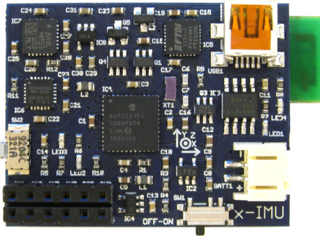
Figure 2: x-IMU top
