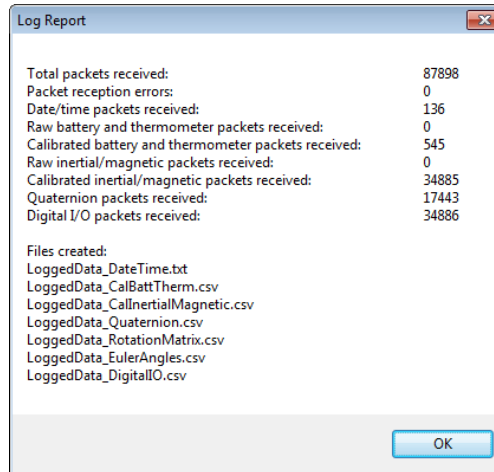
Figure 14: x-IMU GUI data logger report
