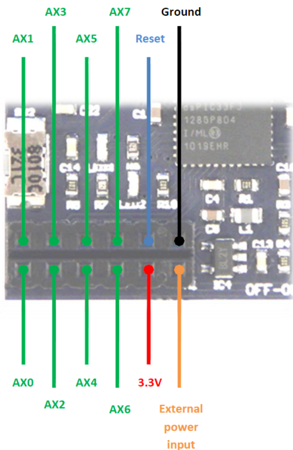
Figure 22: Auxiliary port pins
