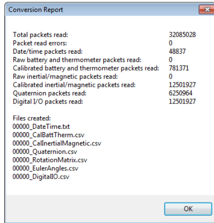
Figure 16: x-IMU GUI binary file conversion report
