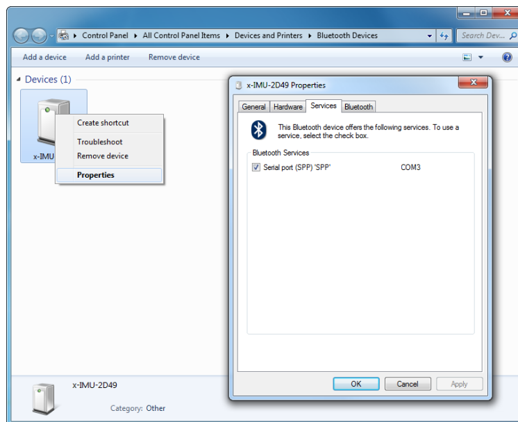
Figure 21: Confirming the port name assigned to the x-IMU Bluetooth pairing
