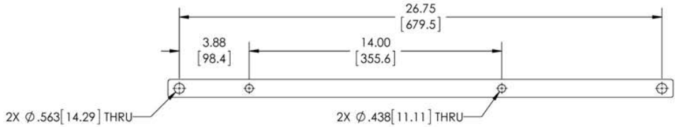
SIDE BAR DETAIL
