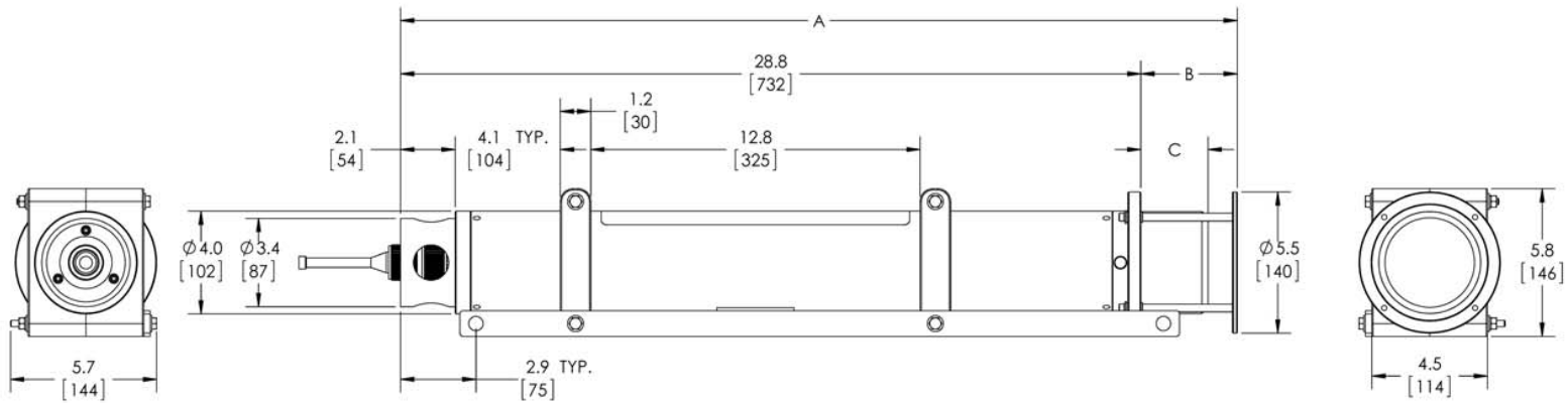
SIDE BAR DETAIL
