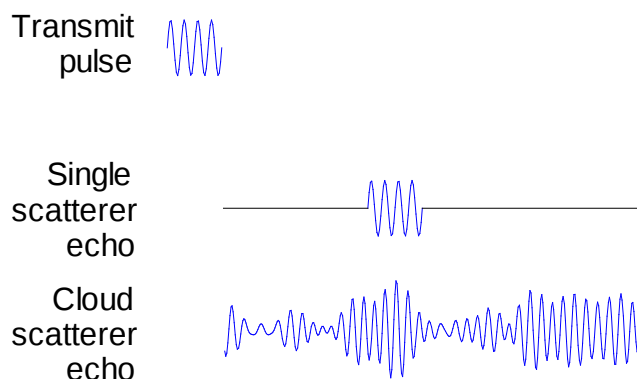
Figure 11. The echo from a single scatterer looks just like the transmit pulse, but the echo from a cloud of scatterers is complicated.
