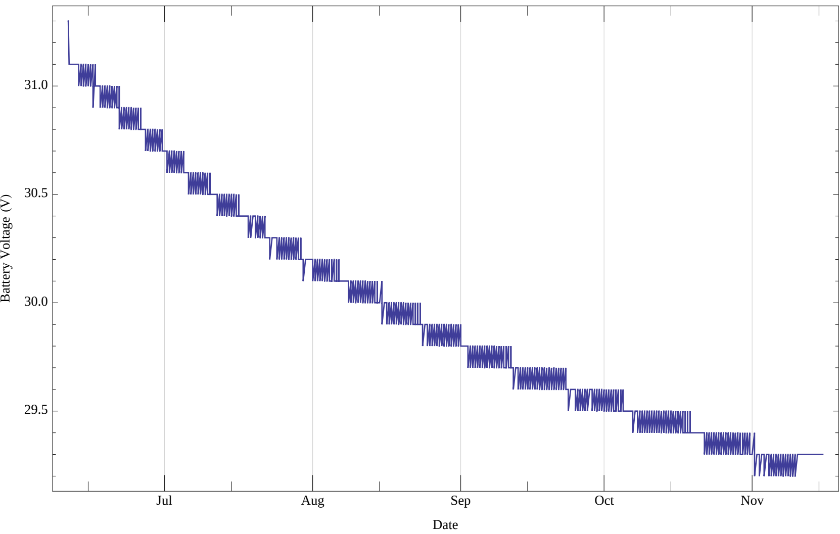
SES Battery Voltage on Pulse 60
