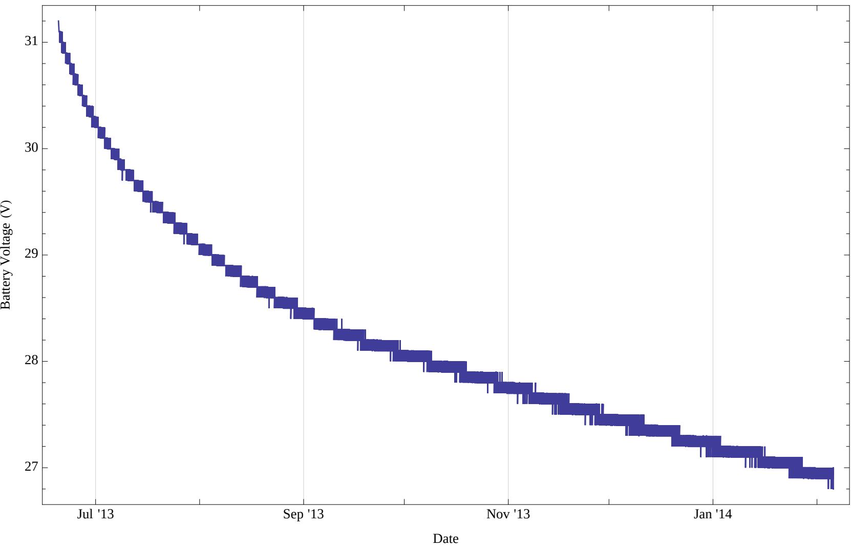
SES Battery Voltage on Pulse 62
