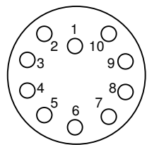
MCOM10M SOCKETS, FACE VIEW
