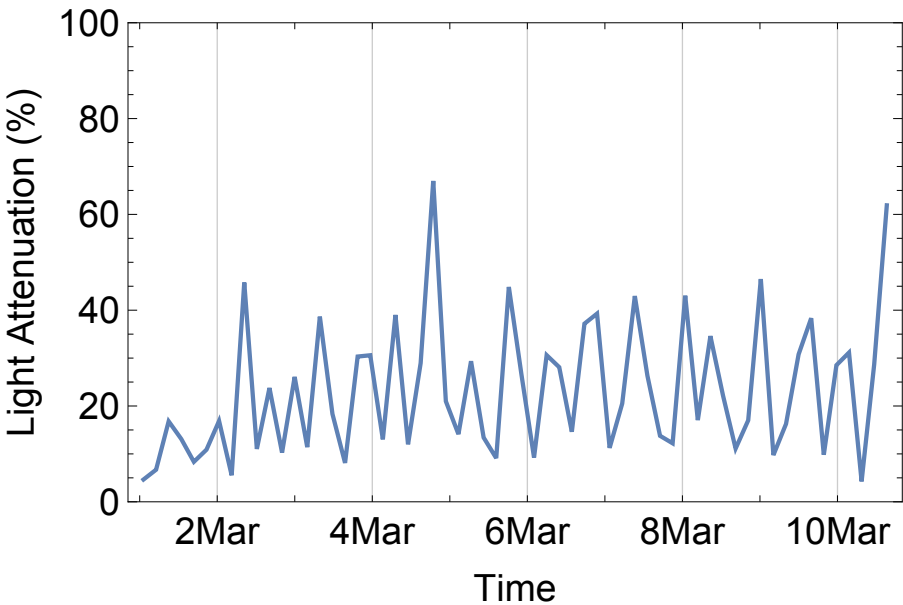
SES Sediment Quantity at Sta. M in March 2015
