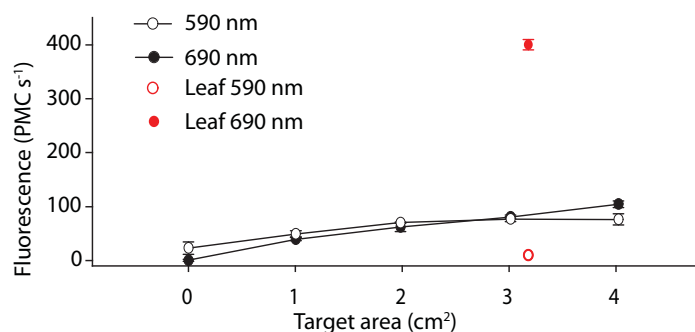
Fig. 4. Fluorescence readings (average \pm standard error) for reference targets of varying sizes [black; Plexiglas Satinice® plum 4H01 DC (polymethylmethacrylate)] and a leaf cutting (red) of varying size, based on a 1 s integration time. Open circles show readings at 590 nm, and dots show readings at 690 nm.
