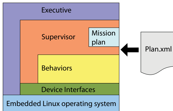
Fig. 5. Diagram of the software architecture, consisting of Ruby and C application code running on a Linux operating system. A mission plan file consisting of a list of Behaviors is read and executed by a Supervisor process.
