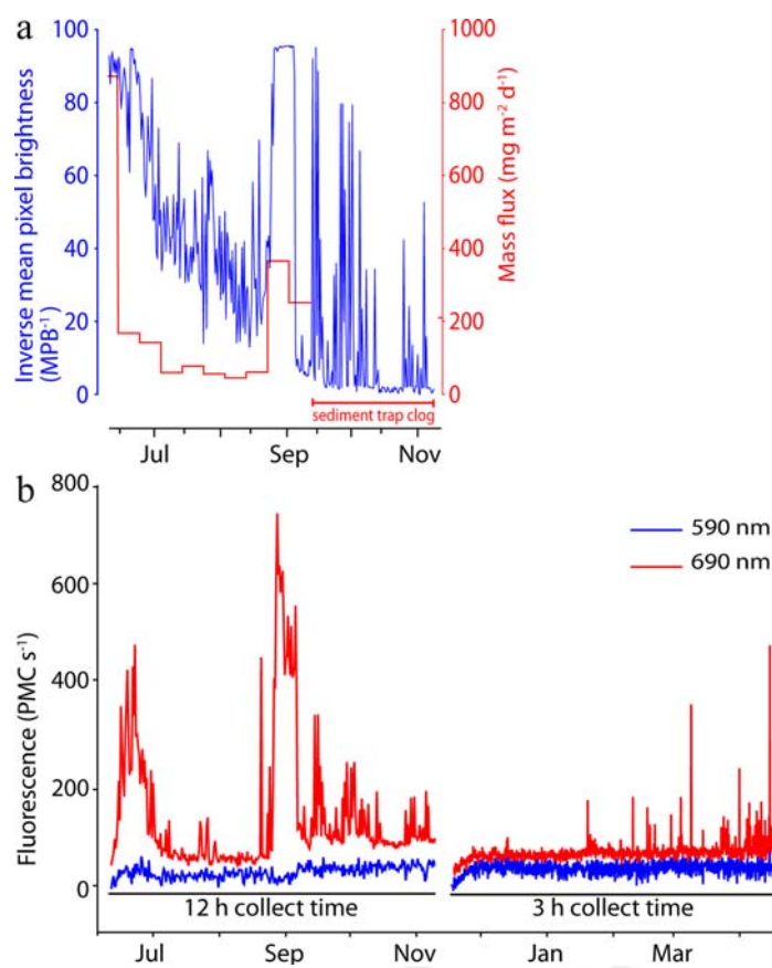
Fig. 8. SES data collected at Station M in 2012. Note different time periods in x-axes. (a) Relative sediment quantity collected by the SES determined by measuring the inverse mean brightness value of the sample plate images (blue line and axis) based on fluorescence readings. Sedimentation rates determined by the SES were comparable to mass flux measured by concurrently deployed sediment traps at the same station and depth (red axis and line). (b) Fluorometer readings during two consecutive deployments with different collect times. The vertical axis values are photomultiplier counts per second. Sustained periods of material fluorescent in the 690 nm band (Chl a ) were seen during the first deployment, but not during the second deployment.
