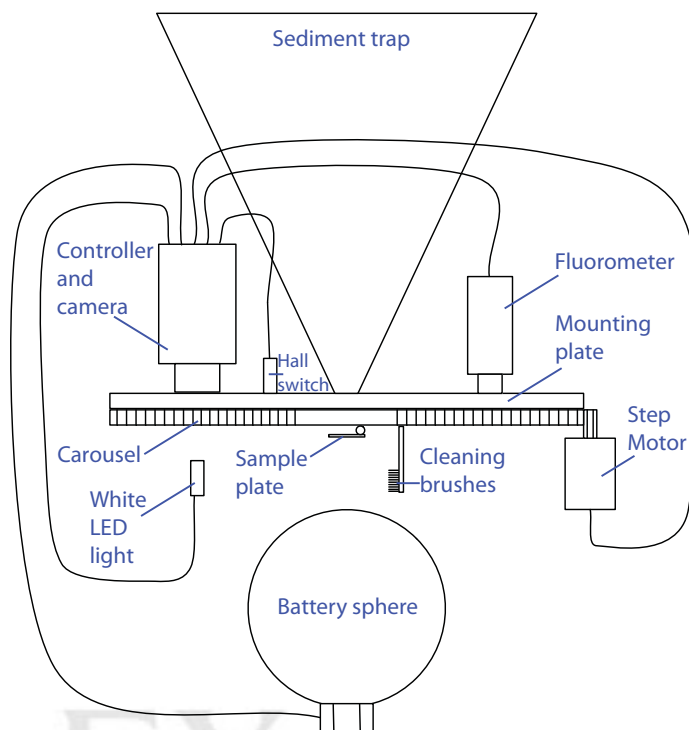
Fig. 2. Placement of major system components. A funnel collects sinking particulate matter, which is then imaged and analyzed by a downward-looking camera and a fluorometer. A large battery, in a titanium sphere, powers the system for more than a year. Components not drawn to scale.
