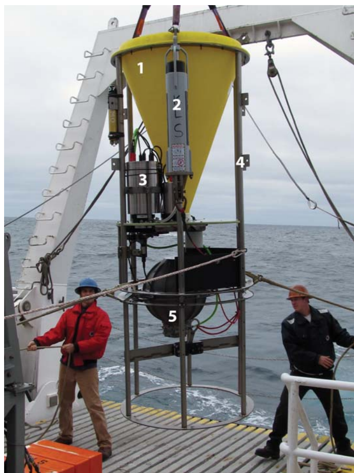
Fig. 1. The SES being prepared for deployment. The instrument is deployed as part of a 140-m-long mooring string. Components shown: (1) funnel, (2) acoustic release, (3) camera and controller housing, (4) titanium frame, (5) battery sphere.
