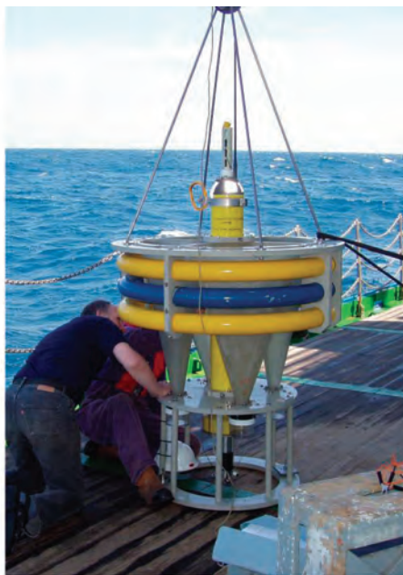
Figure 2.3. Photos of two neutrally buoyant traps used successfully to collect sinking particles in the ocean. (a) NBST (Valdes and Price, 2000; Valdes and Buesseler, 2006). (b) PELAGRA (Lampitt et al. , 2004).
