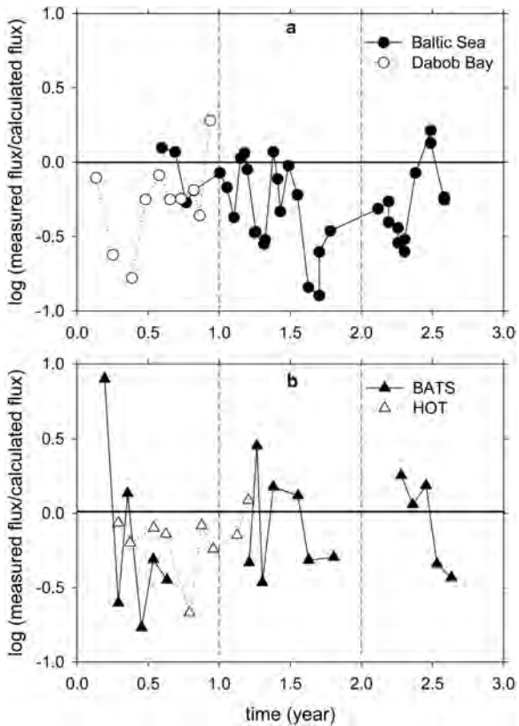
Figure 5.2. Time-series of sediment trap collection efficiency (measured trap 234 Th flux /calculated 234 Th flux plotted on log scale) vs. the relative time of year for two coastal ocean sites (a. upper panel) and two open ocean sites (b. lower panel). Note BATS winter data are not plotted since the comparison breaks down when the winter mixed layer is deeper than the 150 m trap.
