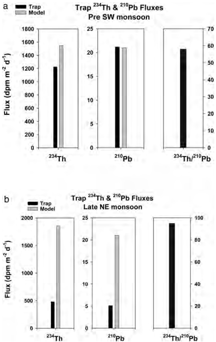
Figure 5.4. A comparison of measured (=Trap) vs. calculated (=Model) ^{234}\text{Th} and ^{210}\text{Pb} fluxes and ^{234}\text{Th}/^{210}\text{Pb} ratios during the early SW Monsoon (upper panels) and later NE Monsoon (lower panels) in the Arabian Sea.
