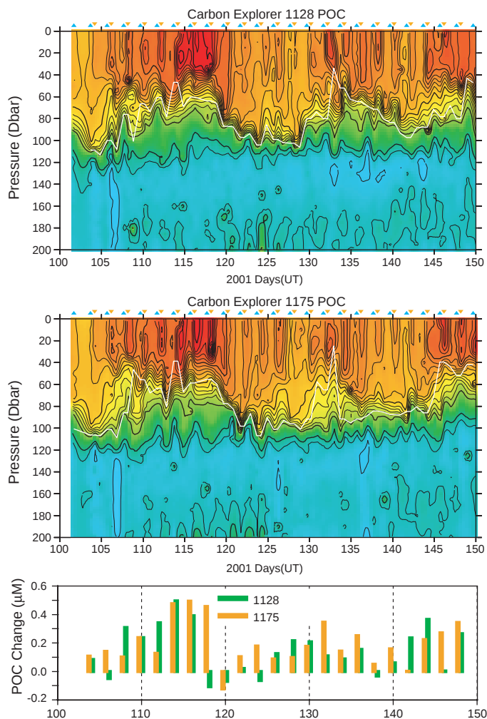
Fig. 2. (Top and middle) Time series of POC variability from SOLO1128 and SOLO1175 during the first 50 days of deployment. Cyan up-triangle and orange down-triangle at the top of each panel are plotted at the times of dawn and dusk profiles, respectively. On alternating days, a mid-day profile also contributes to the time series. Heavy black contours for cold to warm colors are drawn at 0.5, 1.0, 2.0, 3.0, and 4.0 \mu\text{M} POC levels. Light contours are at 0.2 \mu\text{M} spacing above 1.0 \mu\text{M} and at 0.1 \mu\text{M} spacing below 0.5 \mu\text{M} . White curve is mixed-layer depth calculated from the dawn Carbon Explorer profile using a potential density increase of 0.05 relative to the surface. Mixing variability was consistent with surface winds retrieved twice per day using the JPL/QUIKSCAT instrument. Storms with winds persistently exceeding 25 knots occurred on days 101 to 102 and on days 119 to 122 and on day 127. Data contoured using GRI software. The “lock-step” nature of both records indicates that observed POC variability is a response to large scale forcing. (Bottom) Daily net growth or loss of POC calculated as dusk minus dawn POC averaged between the surface and depth of the dawn “mixed layer.” Enhanced net growth rates occurred on days 114 through 118 approximately 2 weeks after Gobi desert dust passed over PAPA.
