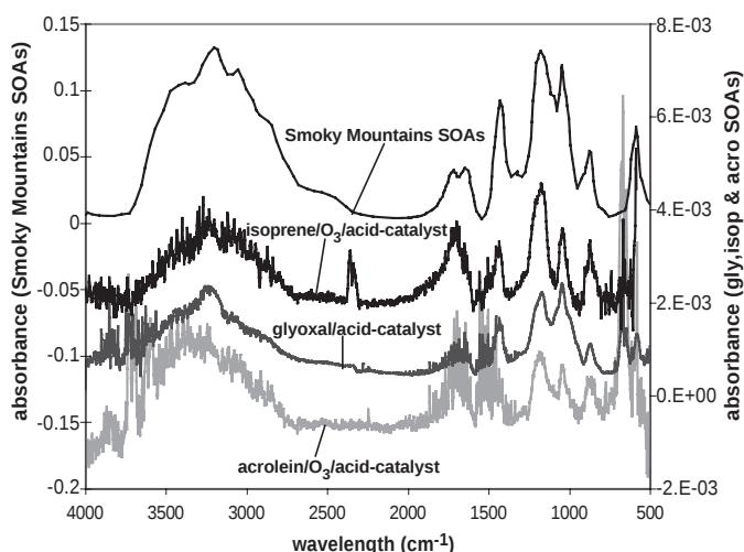
Fig. 4. FTIR spectra of organic aerosols impacted on an ungreaed ZnSe FTIR disk for the glyoxal-(NH 4 ) 2 SO 4 -H 2 SO 4 system and SOAs from the reaction of O 3 with isoprene and acrolein in the presence of an acid catalyst (H 2 SO 4 ). The FTIR spectrum for SOAs from the Smoky Mountains was obtained from Blando et al. (31): FTIR spectrum of 0.5- to 1.0-μm aerosols collected on 13 August 1995 at Look Rock, Smoky Mountains, Tennessee. Axis label E-03 indicates × 10 -3 .
