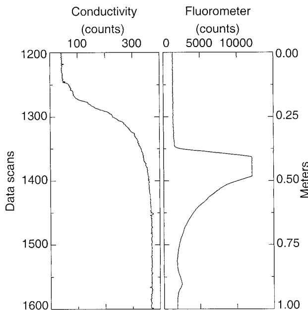
FIG. 6. Typical transient response measured during passage through a dye layer.
