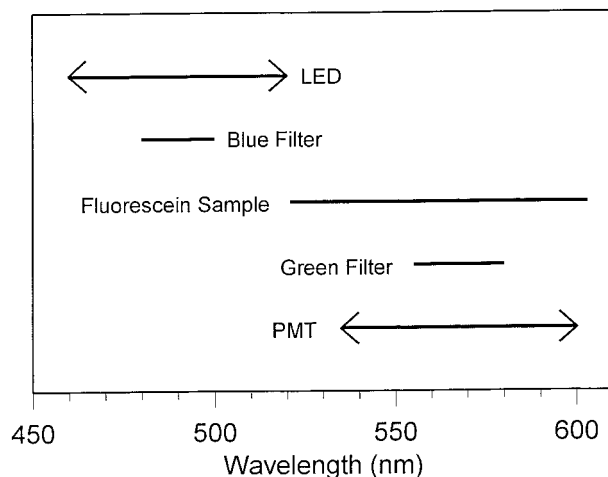
FIG. 2. Bands of emission, transmission, or response for components given in Fig. 1. Bands for the LED and PMT are greater than shown.
