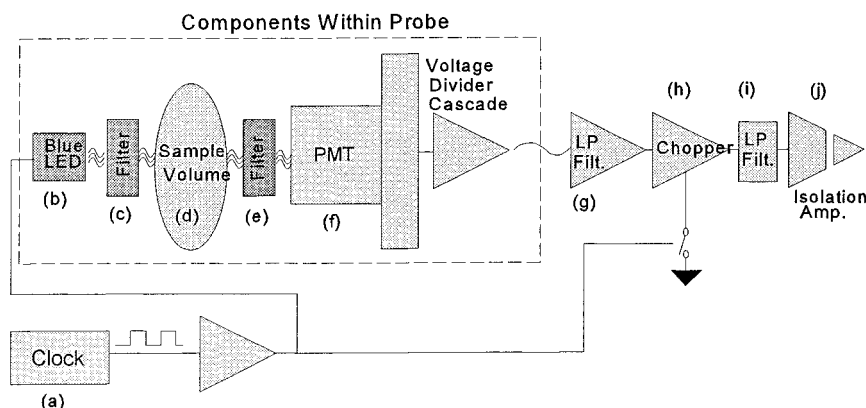
FIG. 1. Schematic of overall fluorometer design.
