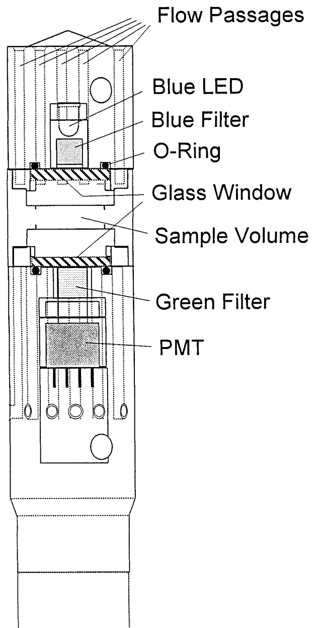
FIG. 4. Internal layout of major components.
