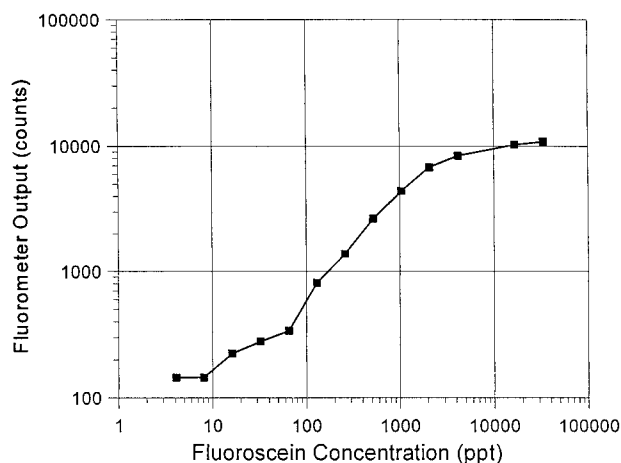
FIG. 5. Static calibration in a well-mixed bath with various dye concentrations.
