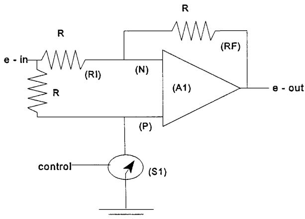
FIG. A1. Schematic of synchronous chopper circuit.
