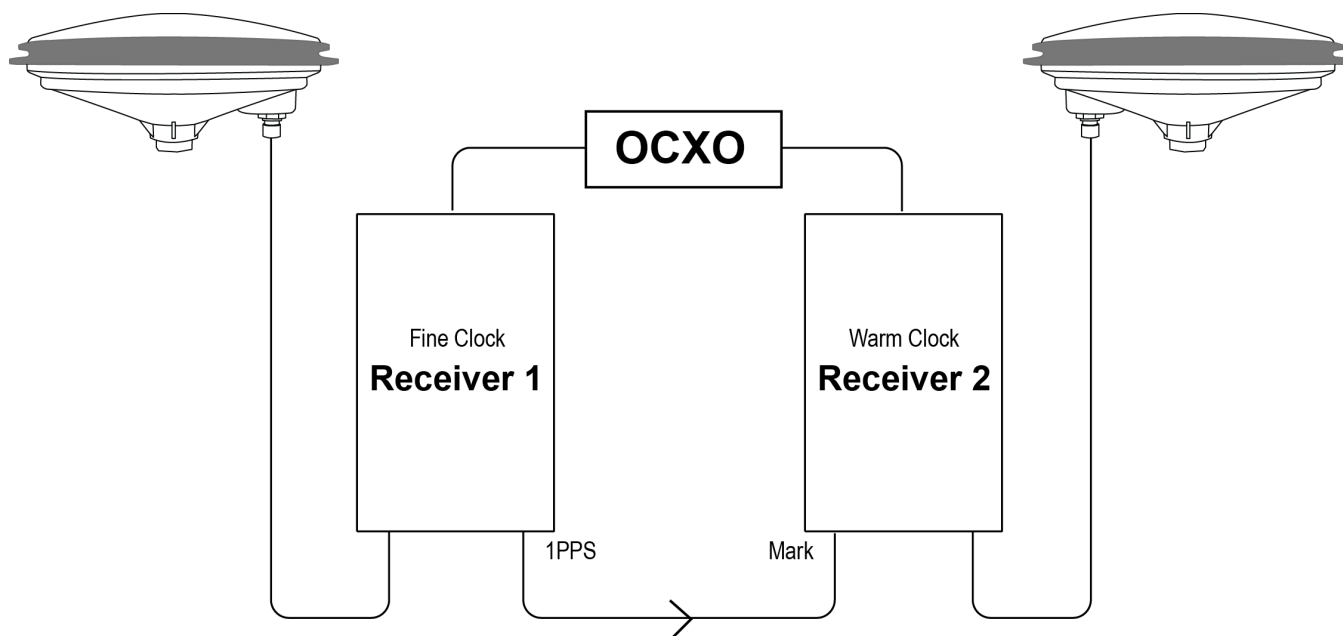
Figure 3: ADJUST1PPS Connections
