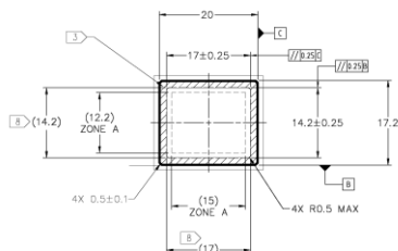
Figure 22: Cover Glass
