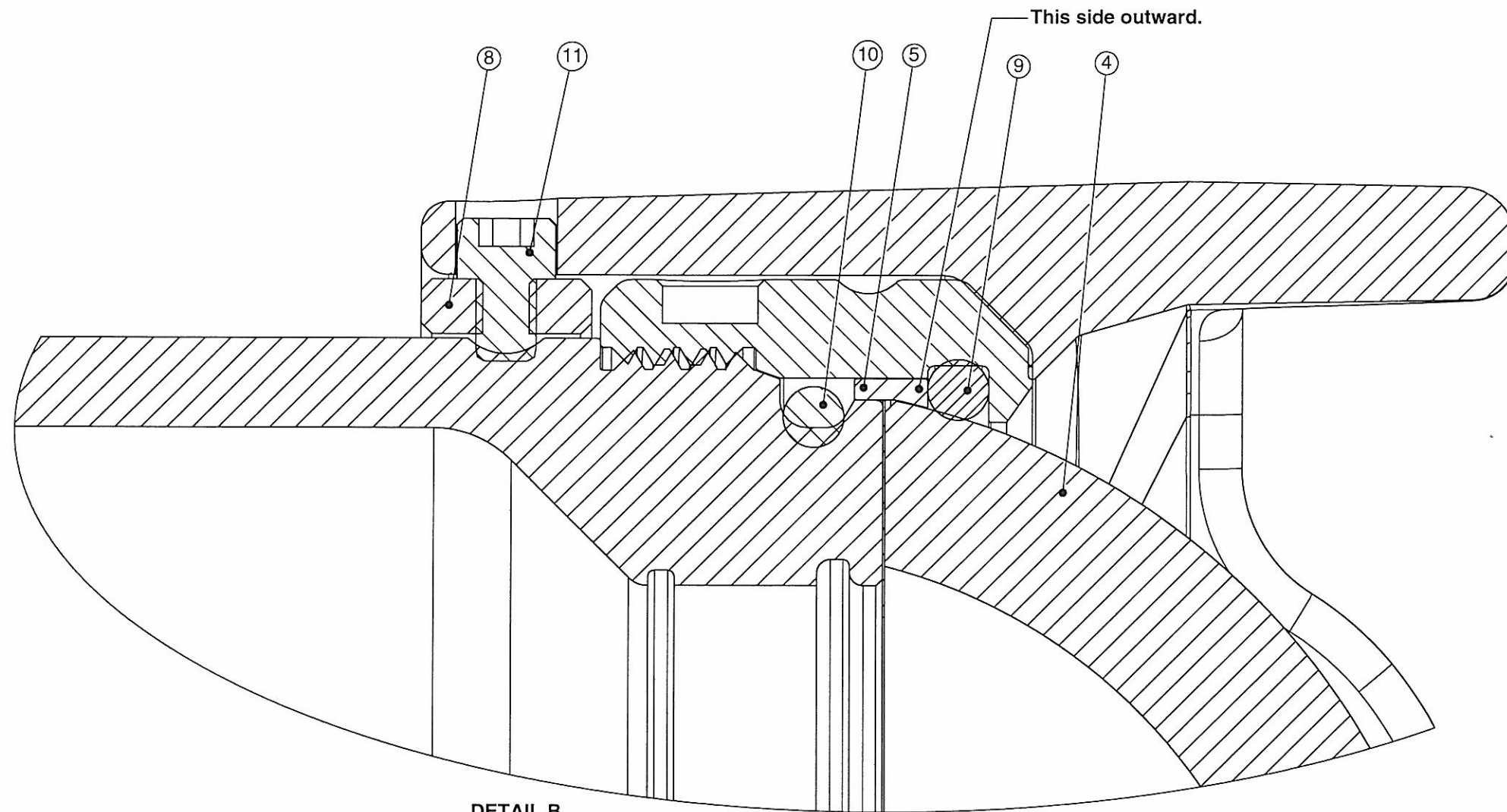
DETAIL B SCALE 3 : 1
