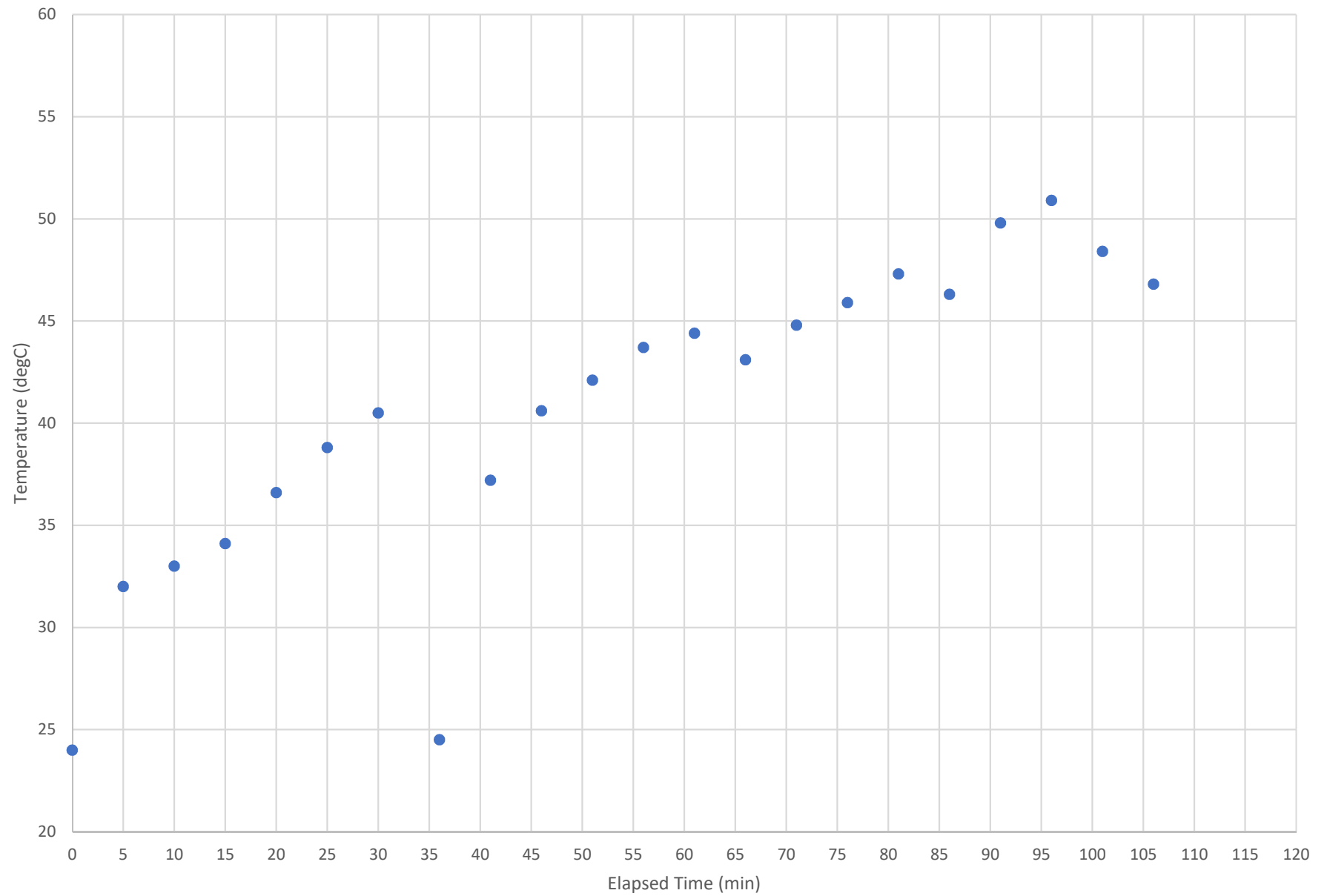
Charge Mosfet Temp vs. Time
