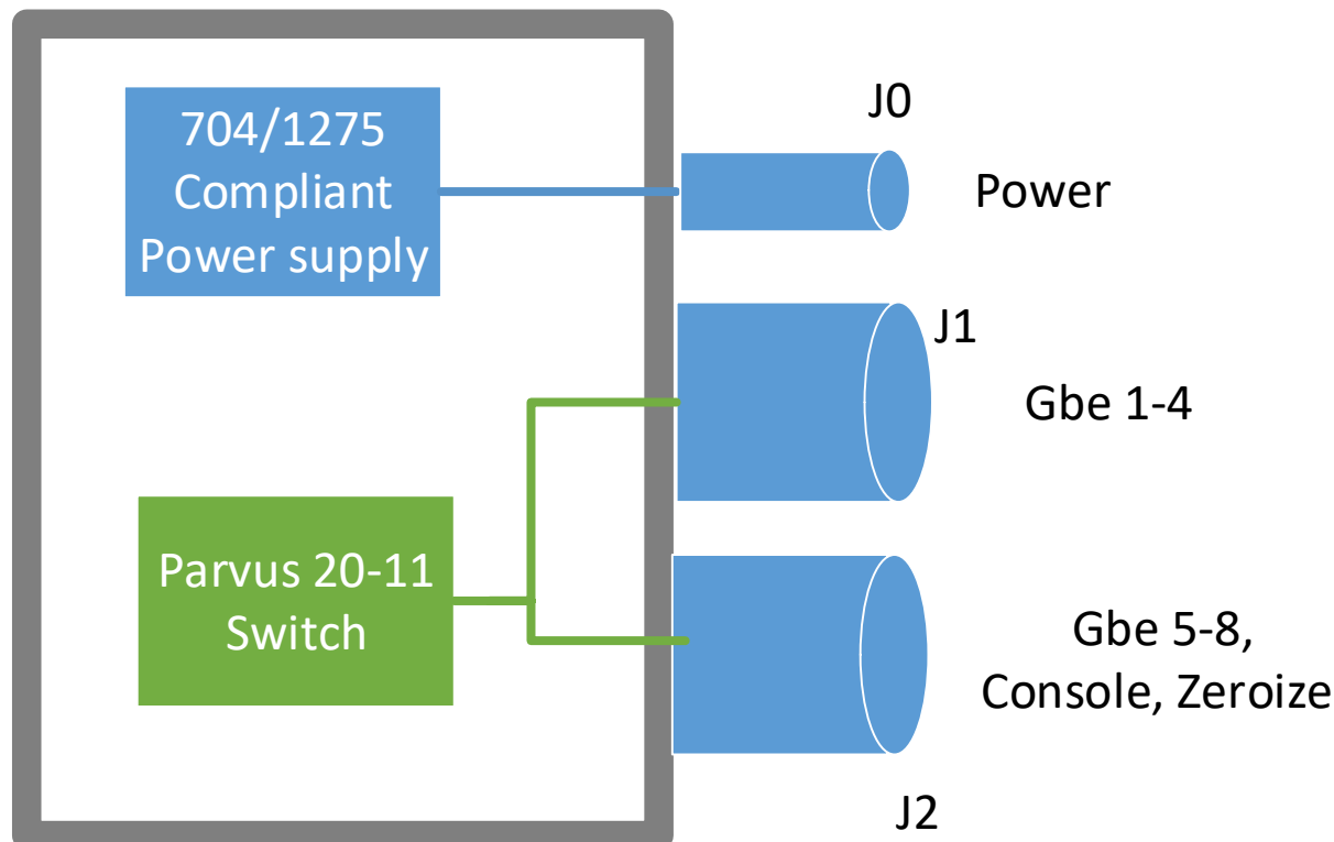
Figure 1. DuraNET 20-11 Block Diagram
