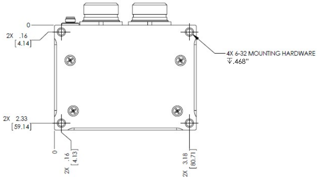
Figure 8. Bottom View
