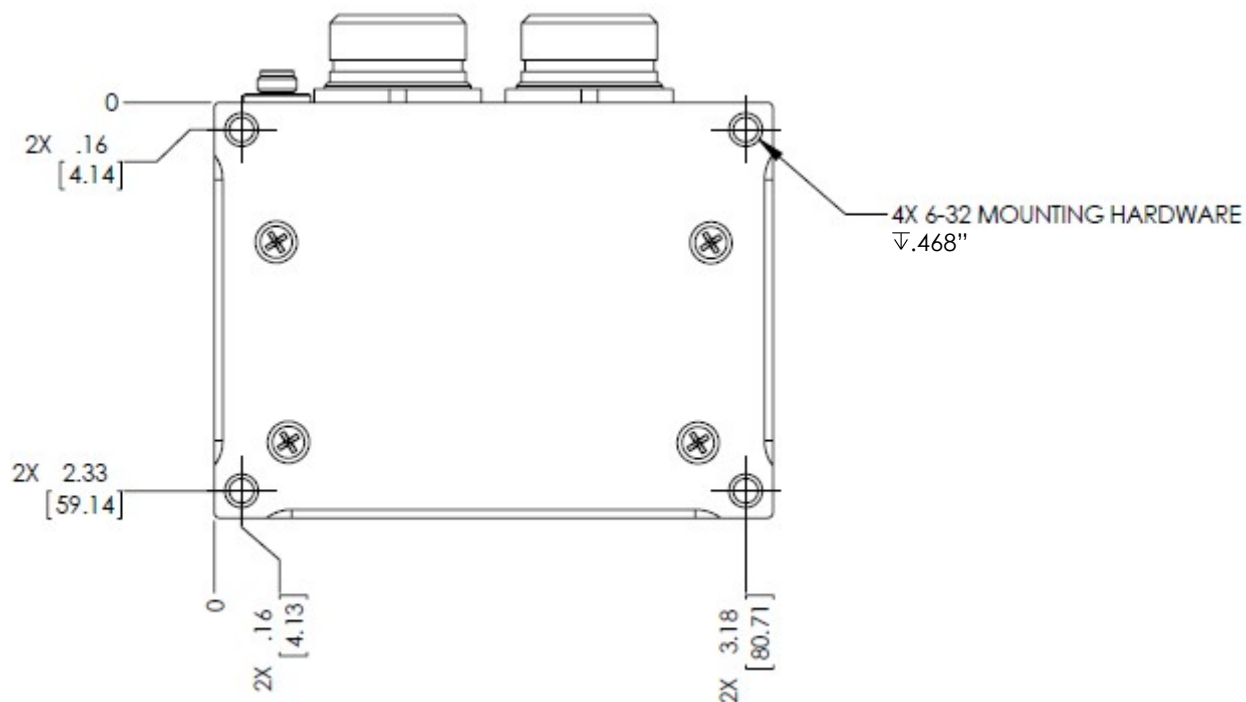
Figure 6. Mounting Holes
