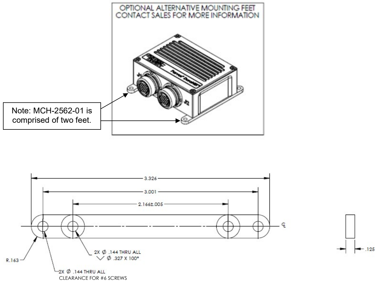
Figure 7 Alternate Mounting Feet
