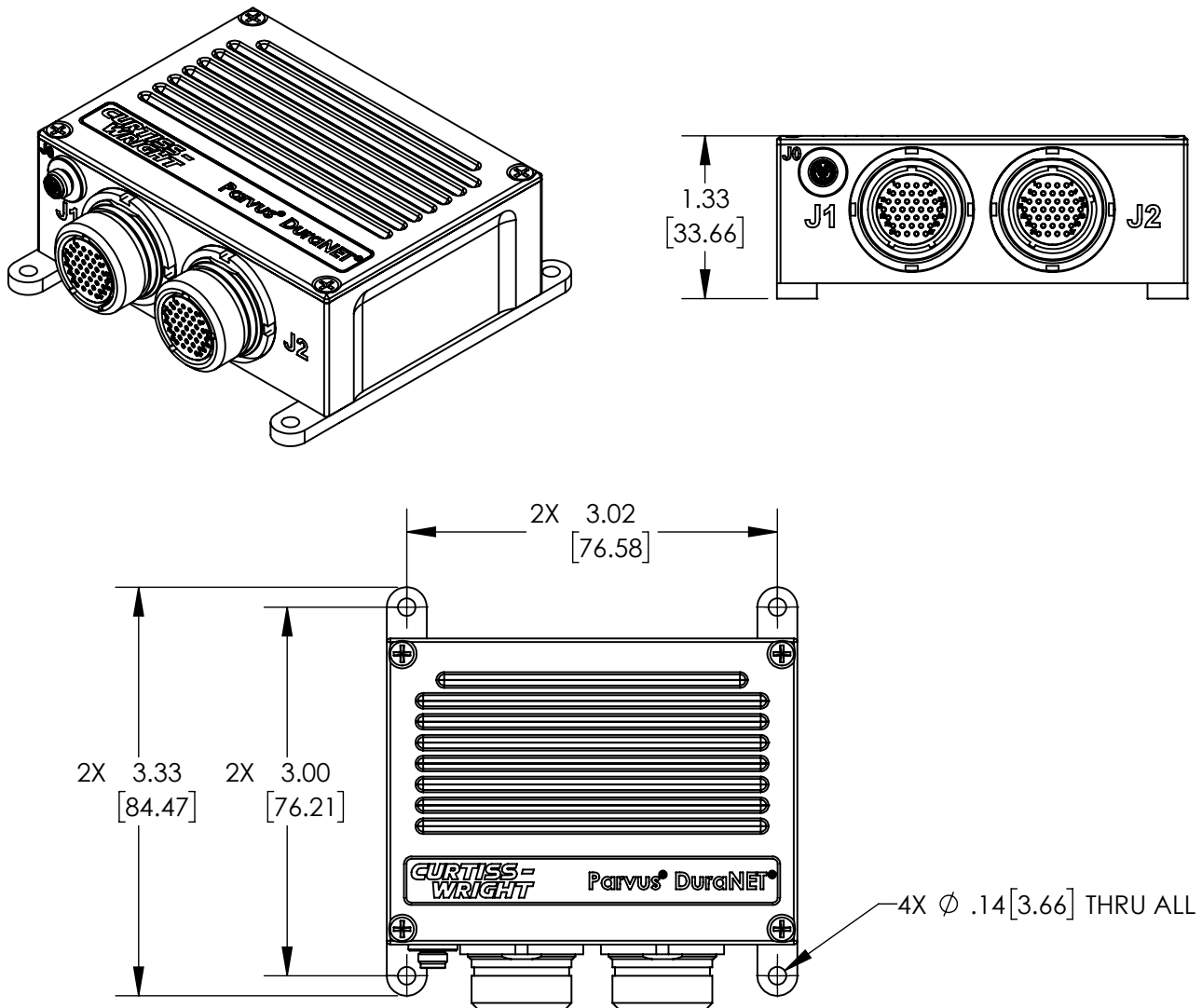
Figure 11: DuraNET 20-11 dimensional line drawings - with optional mounting brackets (measurements shown are in inches and [mm])
