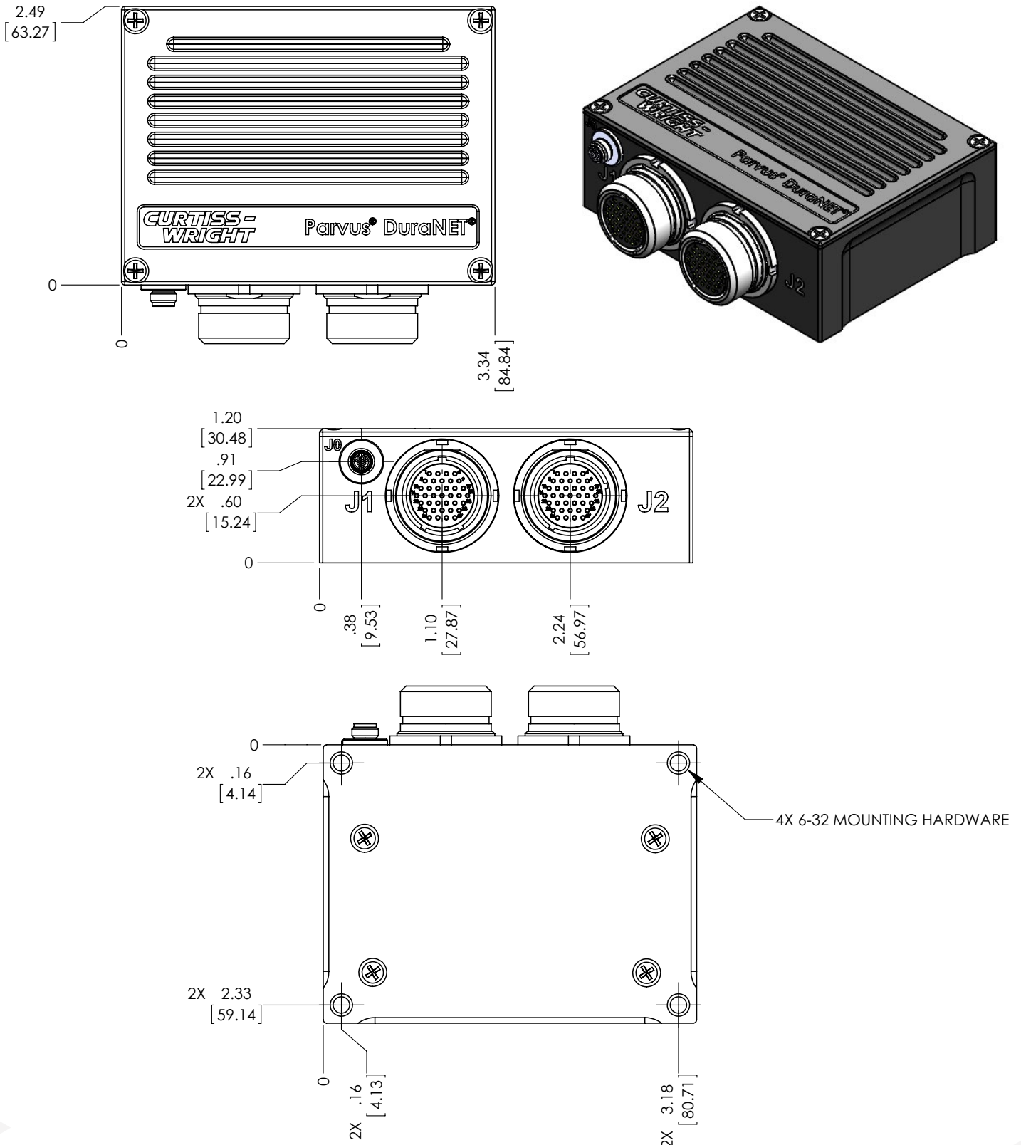
Figure 10: DuraNET 20-11 dimensional line drawings (measurements shown are in inches and [mm])
