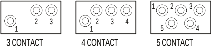
CONTACT CONFIGURATION (MP FACE VIEWS)
