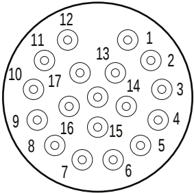
18 CONTACT
