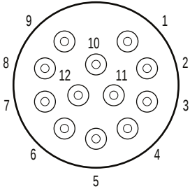
CONTACT CONFIGURATION (MP FACE VIEW)
