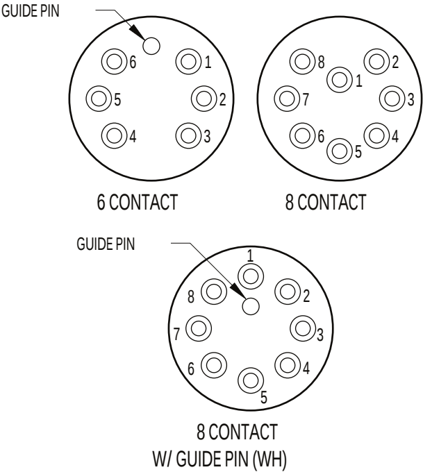
CONTACT CONFIGURATION (MP FACE VIEWS)
