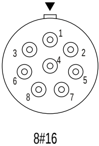
CONTACT CONFIGURATION (BCR FACE VIEW)
