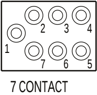
CONTACT CONFIGURATION (MP FACE VIEW)
