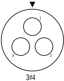
CONTACT CONFIGURATION (BCR FACE VIEWS)
