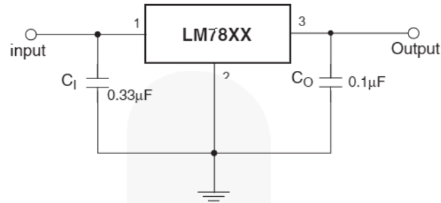
Figure 9. Fixed-Output Regulator
