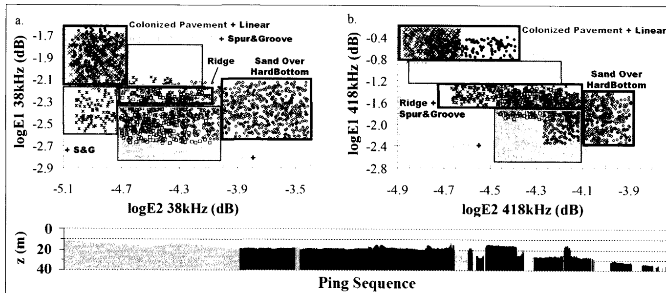
Figure 7. Depth-normalized and log-transformed values of the acoustic energy parameters E1 and E2, reduced to a 20–80 percentile sub-set, plotted in the XY Cartesian space of the E1:E2 bottom ratio classification method for the (a) 38 kHz signal and (b) 418 kHz signal. Boxes denote E1:E2 boundaries used for accuracy assessment of training dataset, with corresponding labels denoting lidar-delineated benthic habitat class membership within each. (Below) Depth profile of the eight lidar-delineated benthic habitat classes in order of acquisition and belonging to the 20–80 percentile sub-set.
