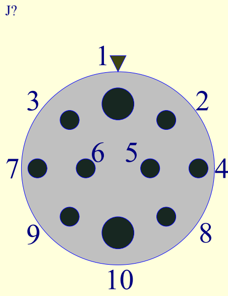
MINK-10-CCPL Cable Female Face
