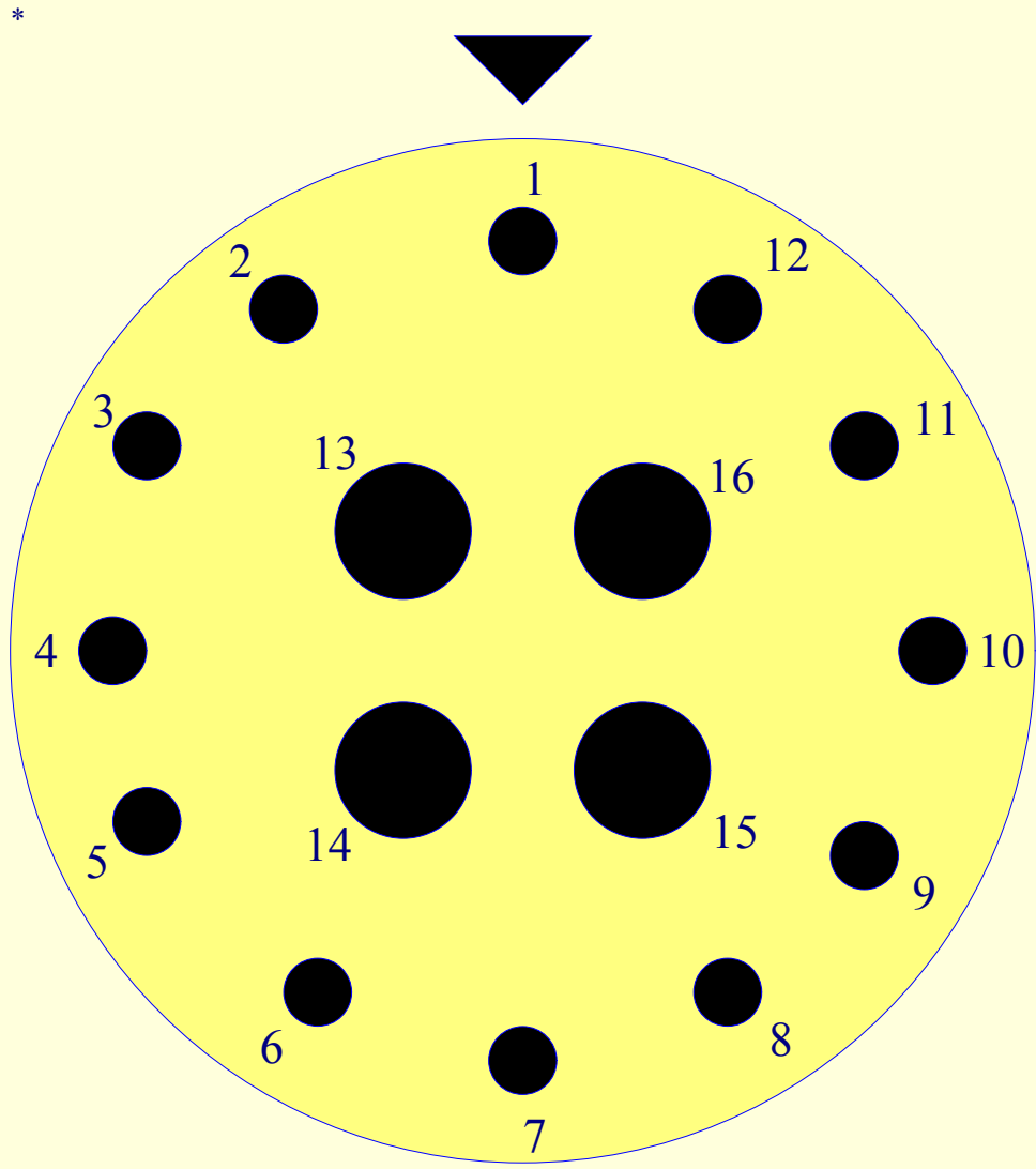
CCR Face View 4#20 12#22 300VDC Max
