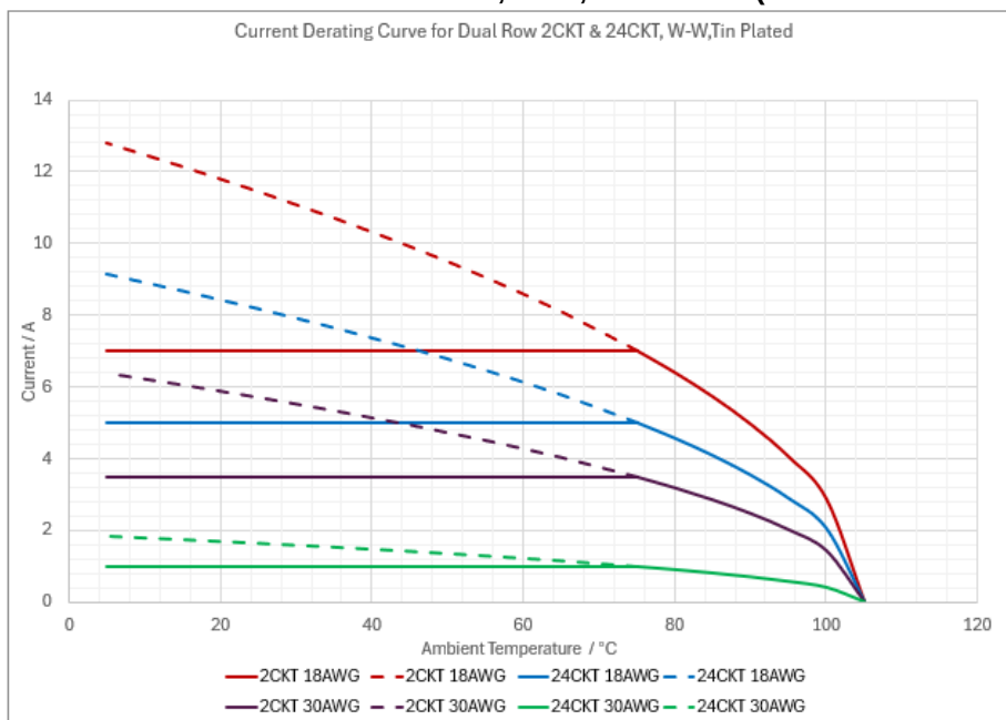
Current Derating Curve for Dual Row 2CKT & 24CKT, W-W, Tin Plated: (dash line means T-rise exceed 30°C)
