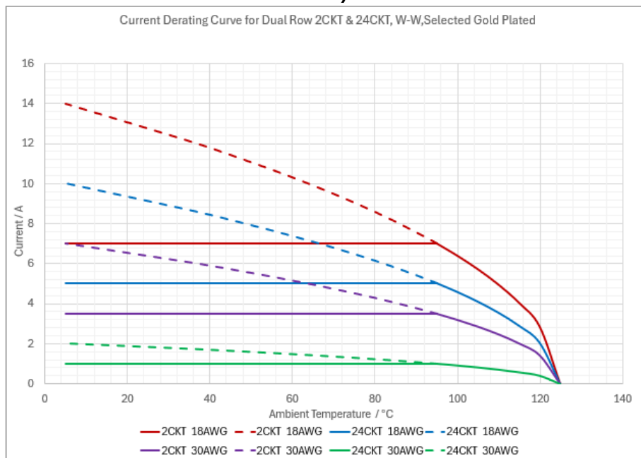
Current Derating Curve for Dual Row 2CKT & 24CKT, W-W, Select Gold Plated: (dash line means T-rise exceed 30°C)
