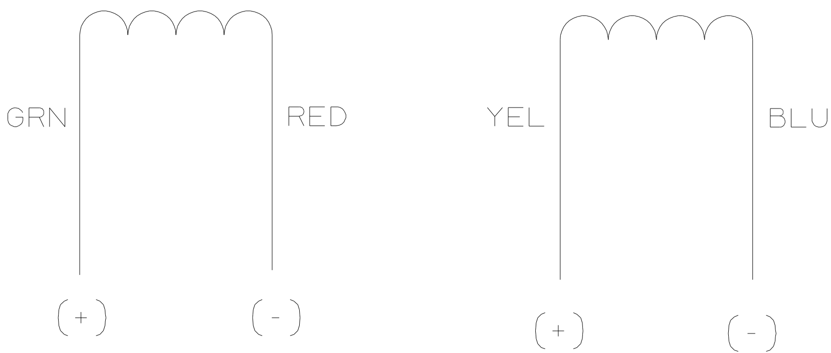
PIGTAIL
